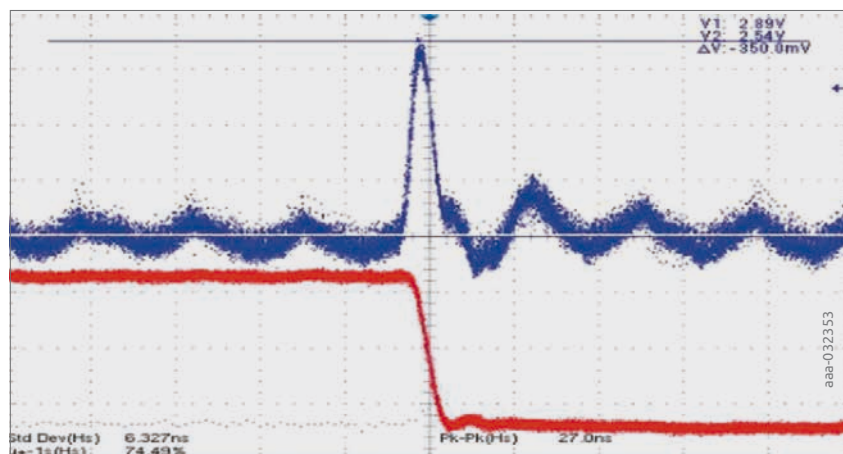
Figure 5.16 | Ground bounce effect caused by signal switching
