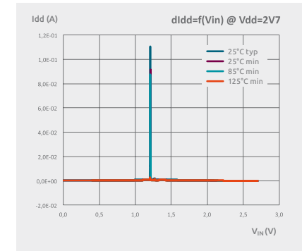
LVT Schmitt-Trigger input curves at 2V7
