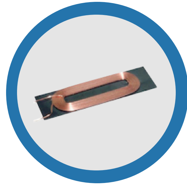
Wireless Charging Receiving Coil / Shield IWAS3010AZEB130KF1
