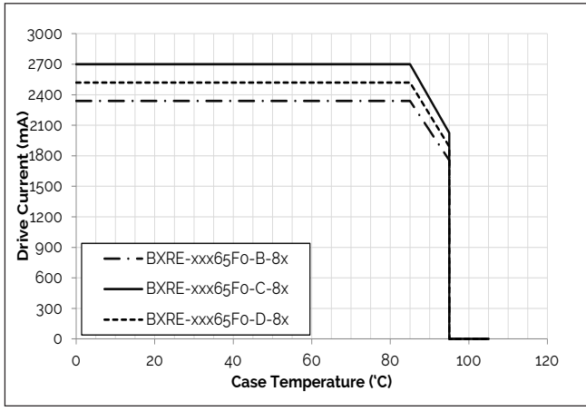
Figure 12: Derating Curve
