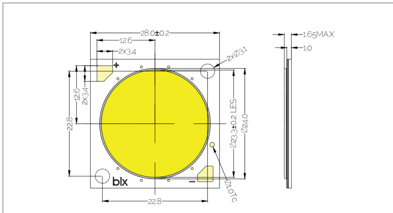
Figure 16: Drawing for V22 LED Array
