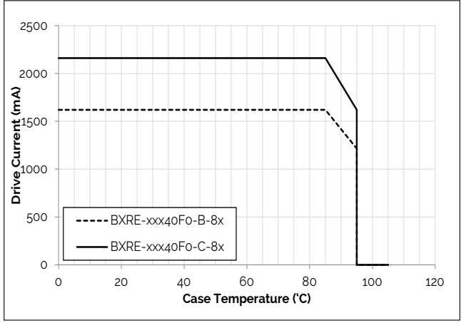
Figure 10: Derating Curve
