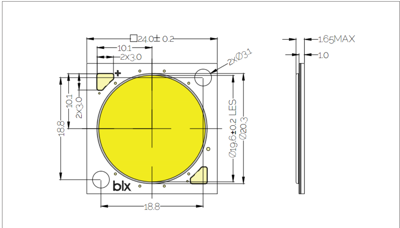
Figure 14: Drawing for V18 LED Array
