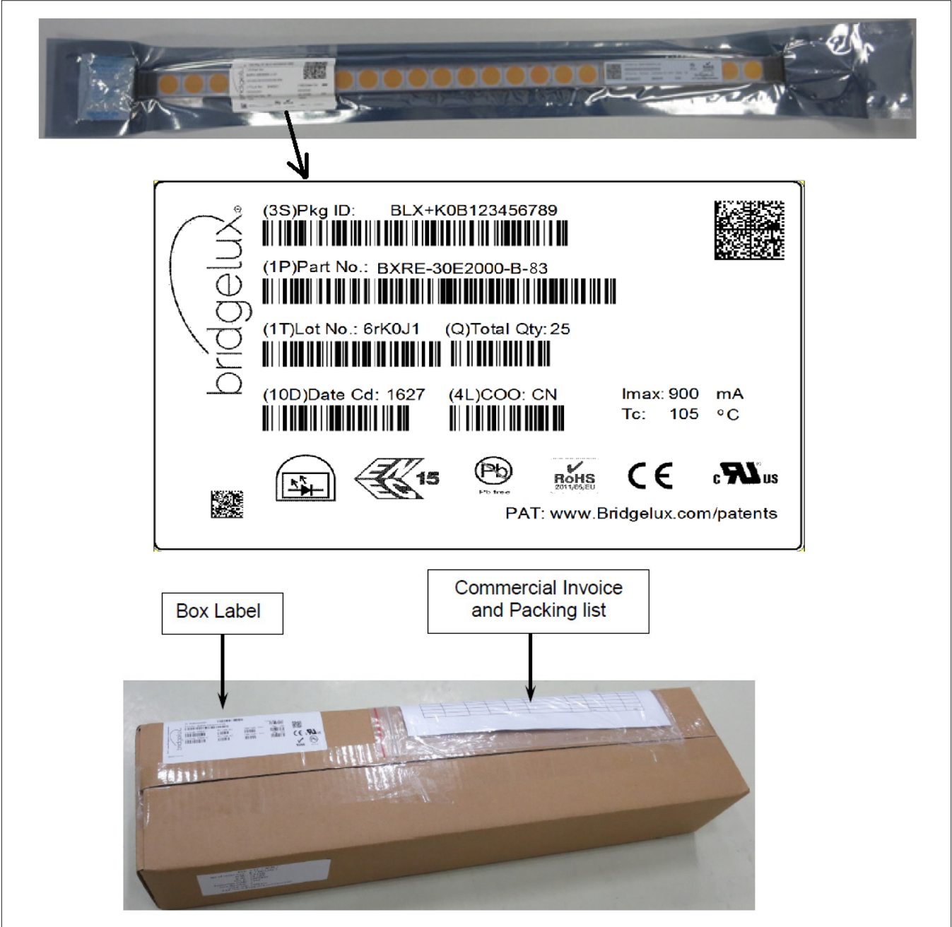
Figure 14: Drawing for V18 Packaging Tube
