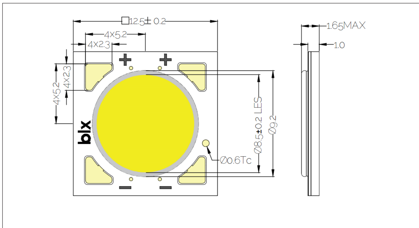
Figure 14: V8 LED Array
