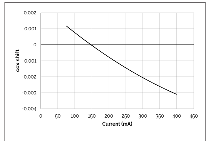
Figure 8: V8E Drive Current vs. ccx Shift
