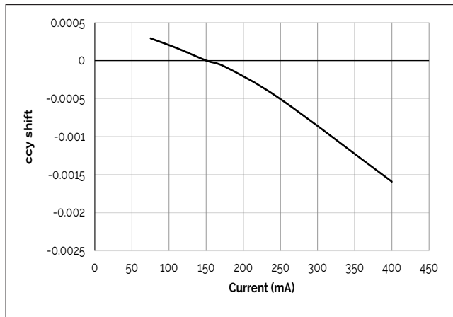
Figure 9: V8E Drive Current vs. ccy Shift
