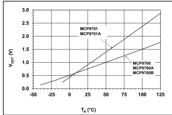
FIGURE 2-17: Output Voltage vs. Ambient Temperature.
