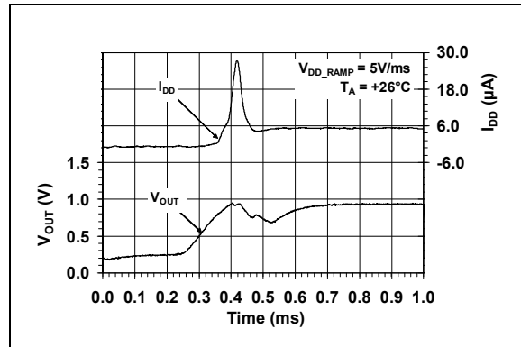
FIGURE 2-18: Output vs. Settling Time to Ramp V_{DD} .
