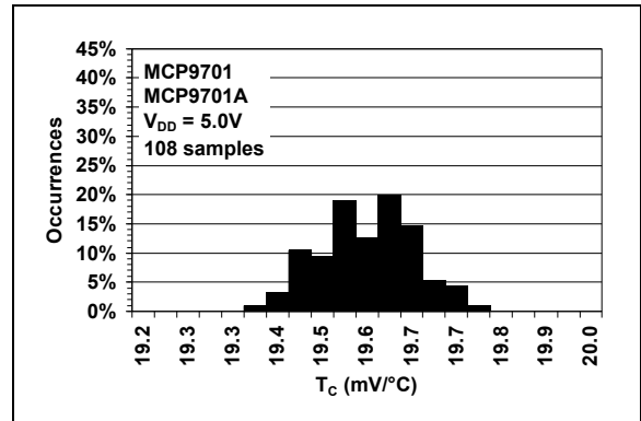
FIGURE 2-12: Occurrences vs. Temperature Coefficient (MCP9701/9701A).
