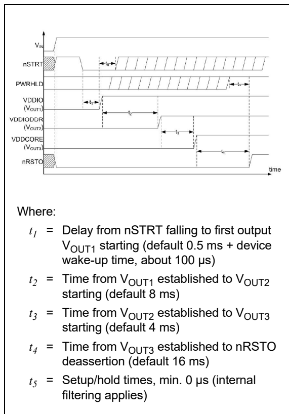
FIGURE 4-4: Start-Up from nSTRT Timing Diagram.
