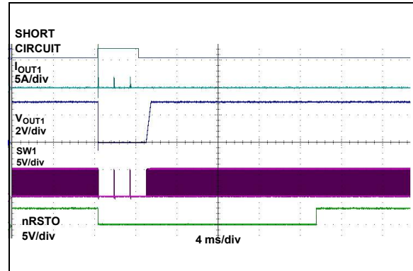
FIGURE 2-17: Output Short Circuit on V_{OUT1} .
