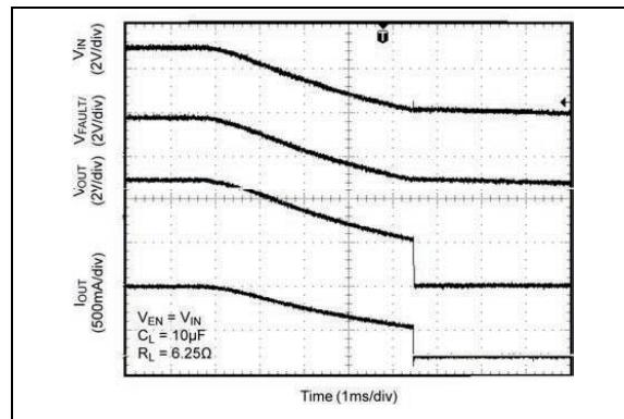
FIGURE 2-28: Turn-Off V IN .
