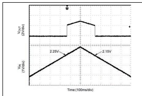
FIGURE 2-30: UVLO.
