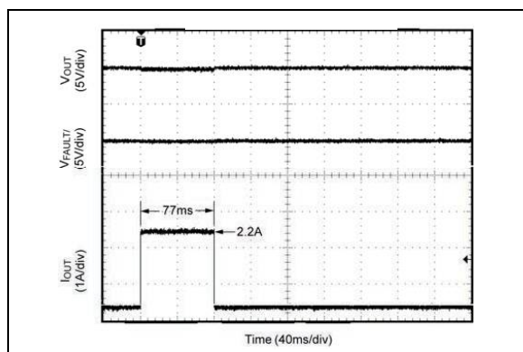
FIGURE 2-38: Kickstart Response 77 ms/2.2A Load Step.
