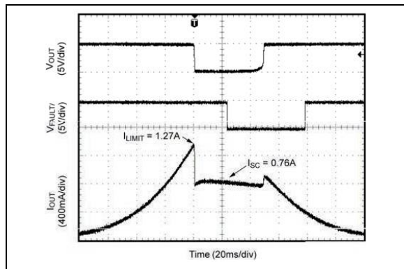
FIGURE 2-37: Current-Limit Threshold.
