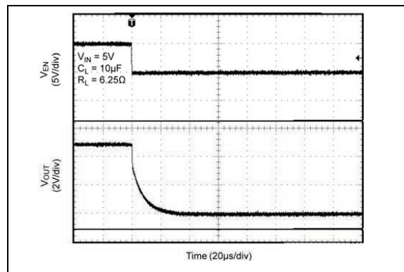
FIGURE 2-29: Enable Turn-Off Delay and Fall Time.
