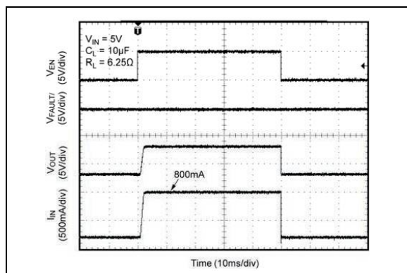
FIGURE 2-27: Enable Turn-On/Turn-Off.
