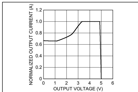
FIGURE 5-3: Normalized Output Current vs. Output Voltage (5V).
