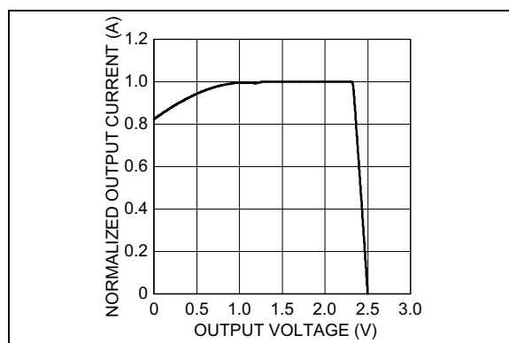
FIGURE 5-4: Normalized Output Current vs. Output Voltage (2.5V).
