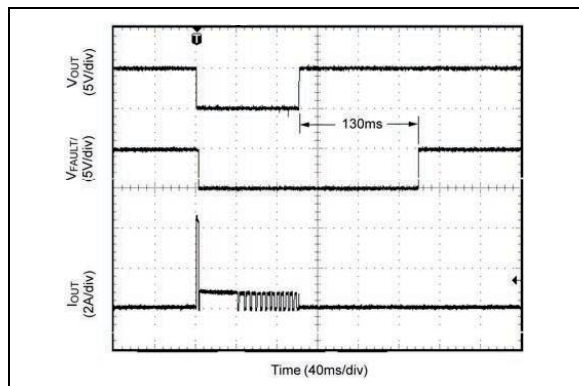
FIGURE 2-39: Kickstart Response Recovery From Thermal Shutdown.
