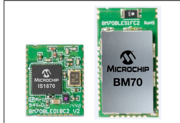
FIGURE 1: BM70 MODULE
