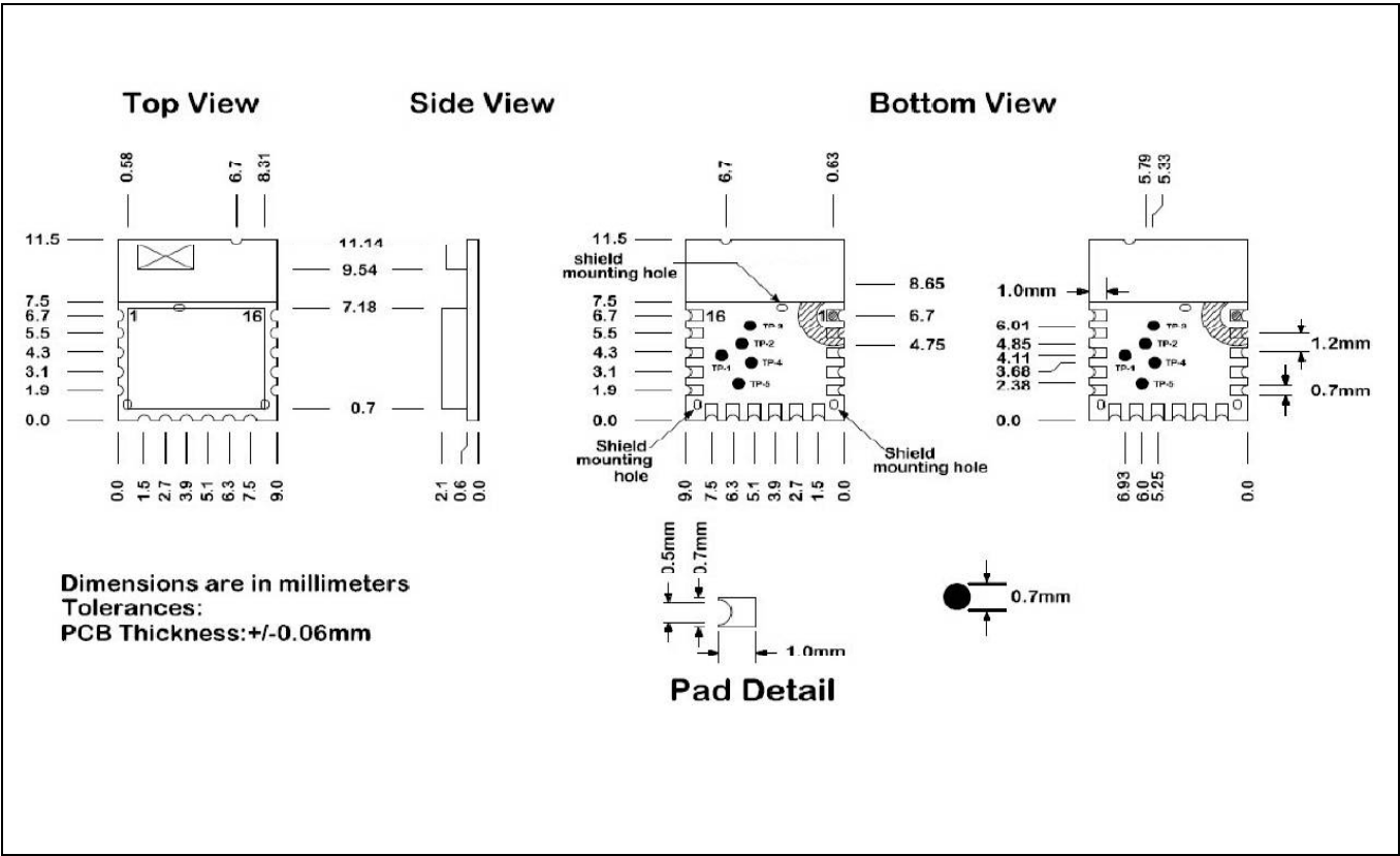
FIGURE 6-5: BM71BLES1FC2 MODULE DIMENSIONS
