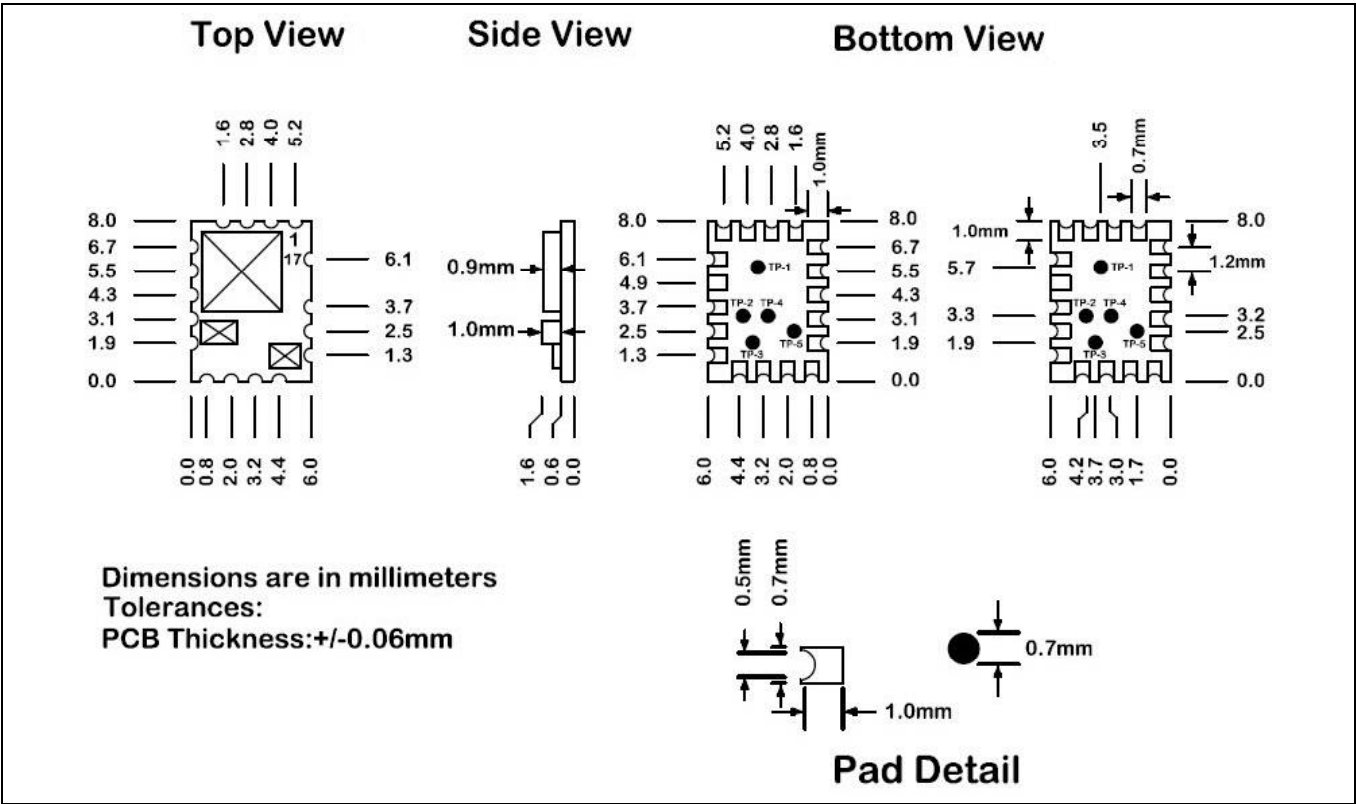
FIGURE 6-7: BM71BLE01FC2 MODULE DIMENSIONS
