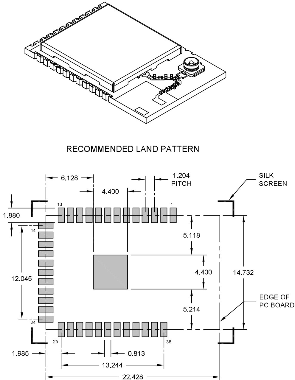
Figure 12-4. ATWINC3400-MR210UA Module Package Drawings - 3D View and Recommended Land Pattern
