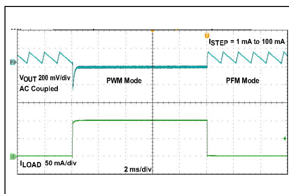
FIGURE 2-33: 3.3V V_{OUT} , Load Transient Waveforms, PFM/PWM Options.
