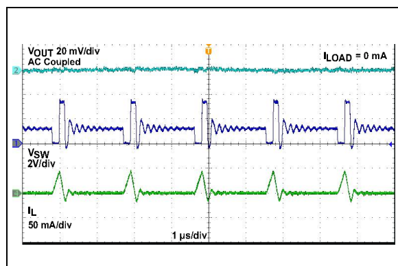
FIGURE 2-32: 3.3V V_{OUT} , No Load, PWM Mode Waveforms.
