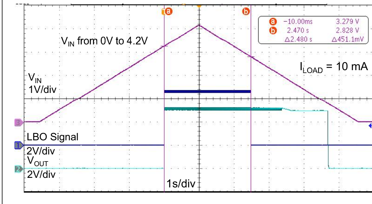
FIGURE 7-3: Dynamic LBO Threshold to Help Optimize Li-Ion Battery Life.
