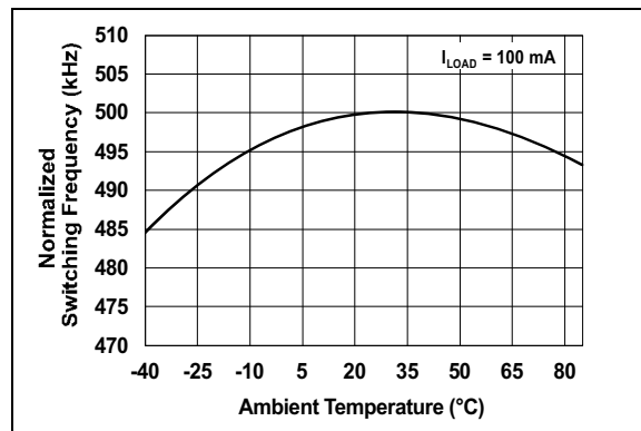
FIGURE 2-22: Normalized Switching Frequency vs. Ambient Temperature.
