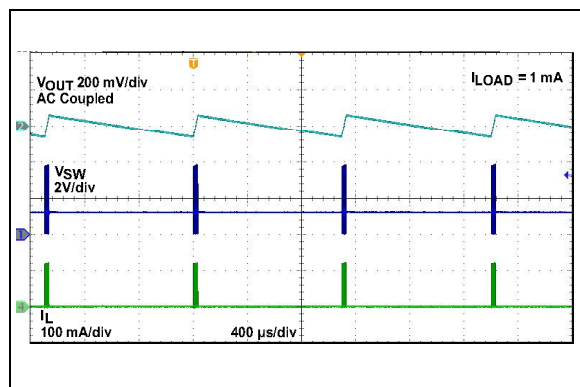
FIGURE 2-31: 3.3V V_{OUT} , PFM Mode Waveforms.
