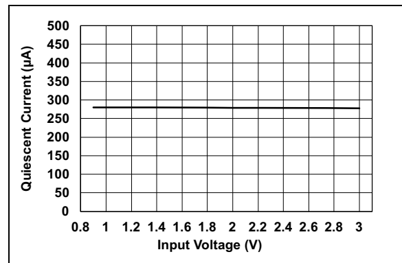
FIGURE 2-5: I_{QOUT} vs. V_{IN} , PWM Only Options.
