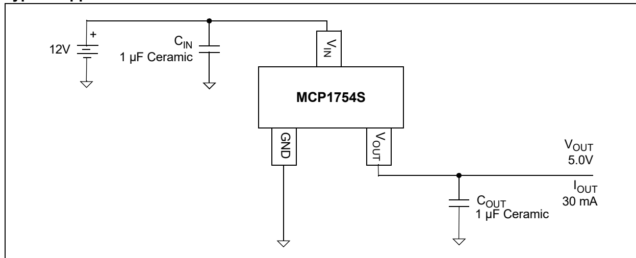
Typical Application Circuits
