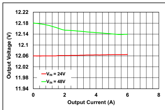
FIGURE 2-8: Output Voltage vs. Output Current ( V_{OUT} = 12V ).
