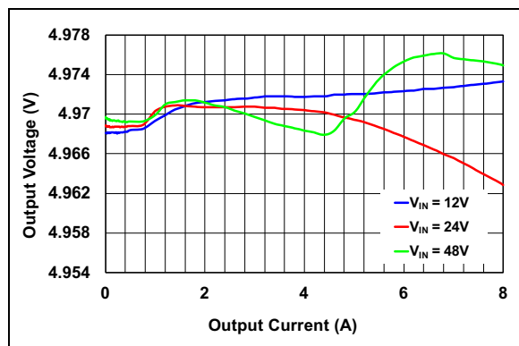
FIGURE 2-7: Output Voltage vs. Output Current ( V_{OUT} = 5V ).
