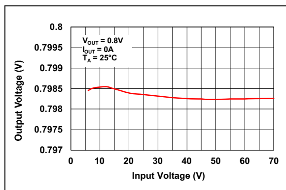
FIGURE 2-9: Output Voltage vs. Input Voltage ( V_{OUT} = 0.8V ).
