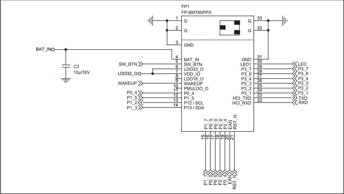
FIGURE 2-11: BM78SPPS5MC2/NC2 REFERENCE CIRCUIT
