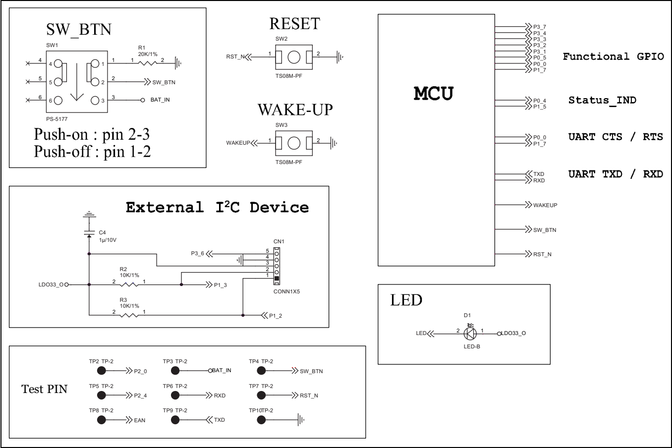
FIGURE 2-12: BM78SPPS5MC2/NC2 REFERENCE CIRCUIT
