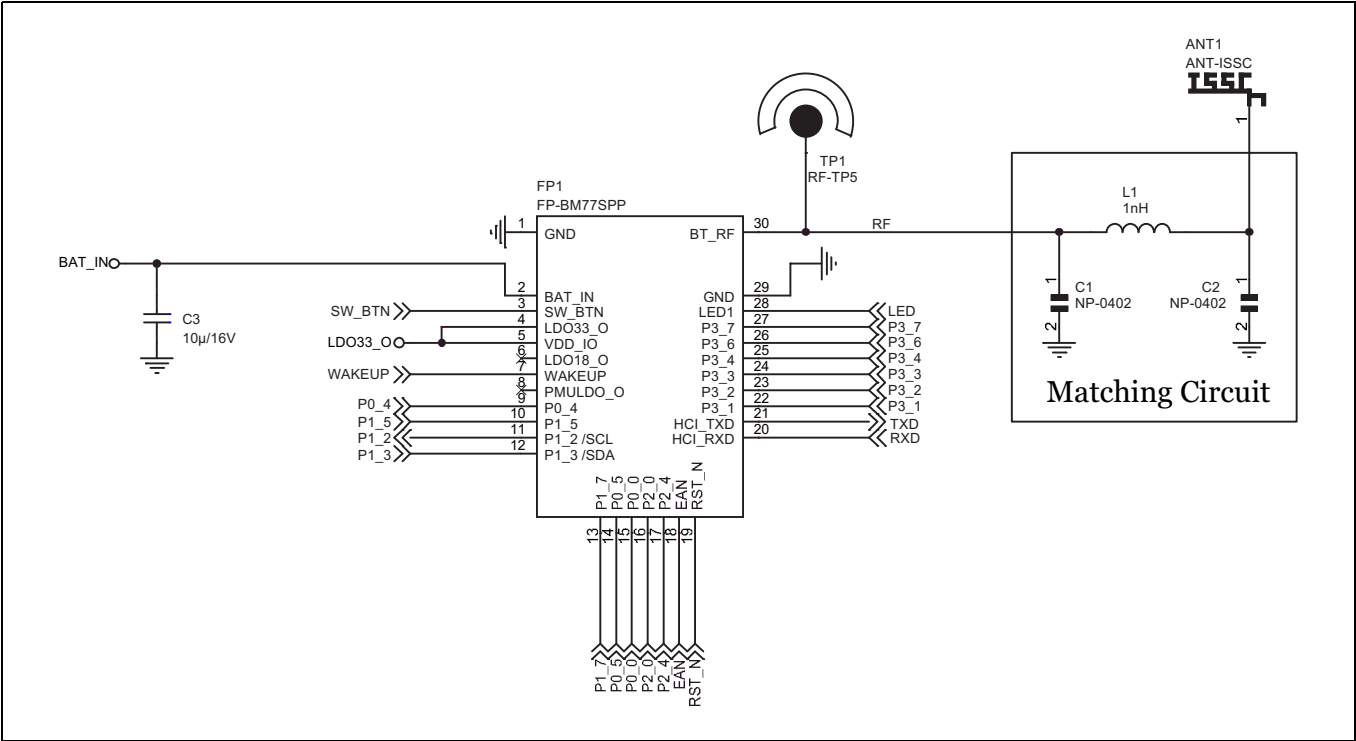
FIGURE 2-9: BM78SPP05MC2/NC2 REFERENCE CIRCUIT
