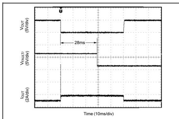
FIGURE 2-32: Current Limit Response, Stepped Short.
