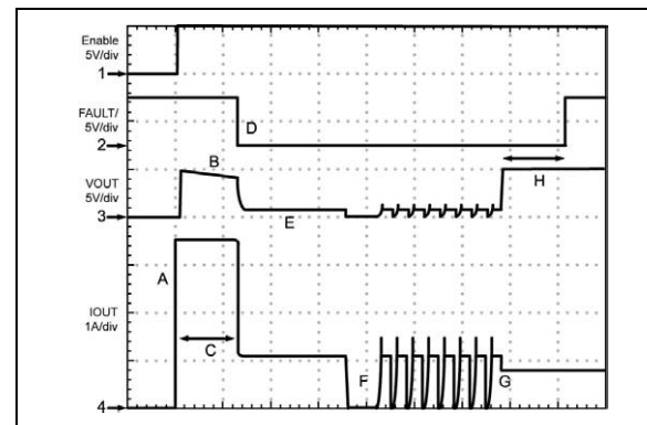
FIGURE 4-1: Kickstart Operation.
