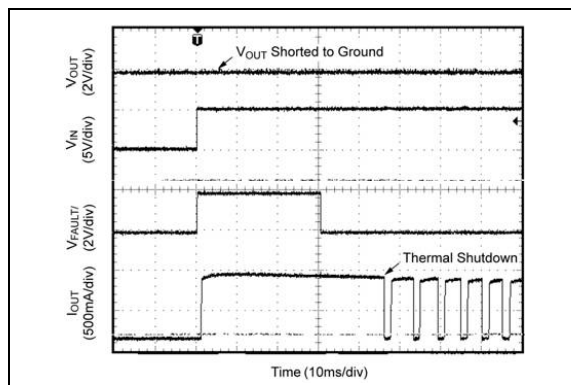
FIGURE 2-34: Power Up Into Short Circuit.
