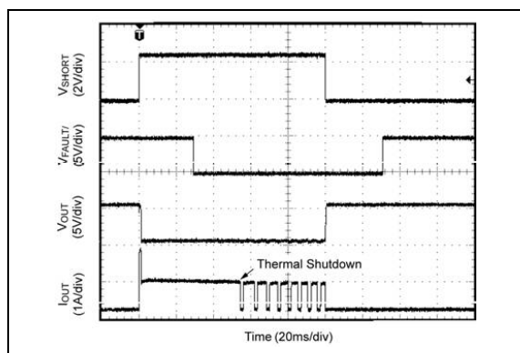
FIGURE 2-36: Output Recovery From Thermal Shutdown.
