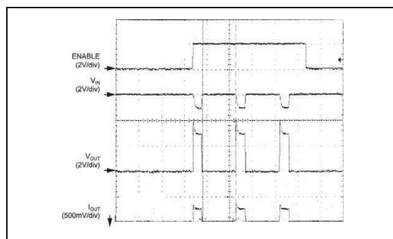
FIGURE 5-6: VUVLO Operation.
