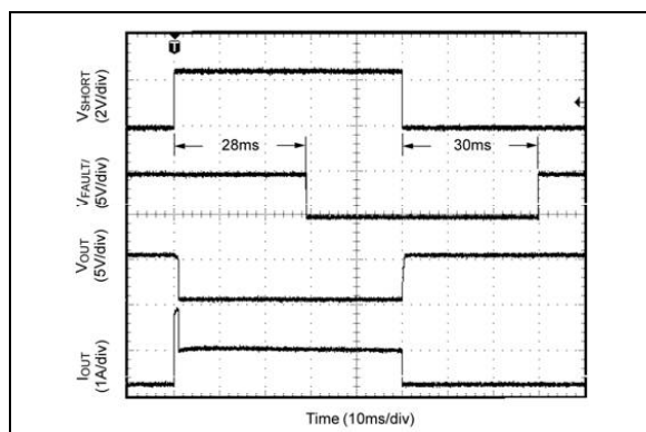
FIGURE 2-33: Output Recovery From Short Circuit.
