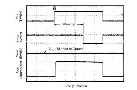
FIGURE 2-31: Enabled Into Short.
