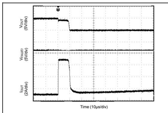
FIGURE 2-35: Current Limit Response Time, Stepped Short.
