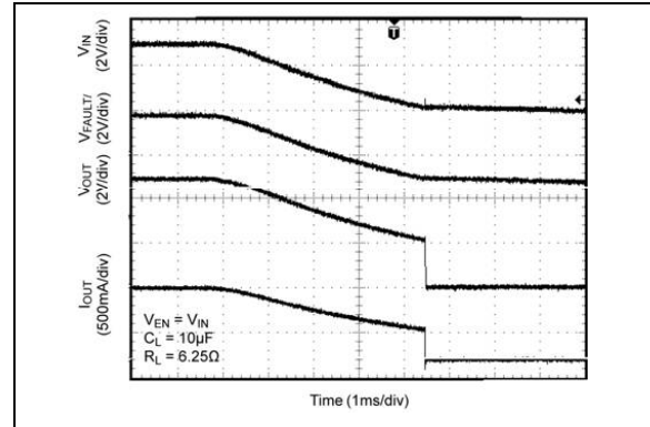
FIGURE 2-28: Turn-Off V IN .
