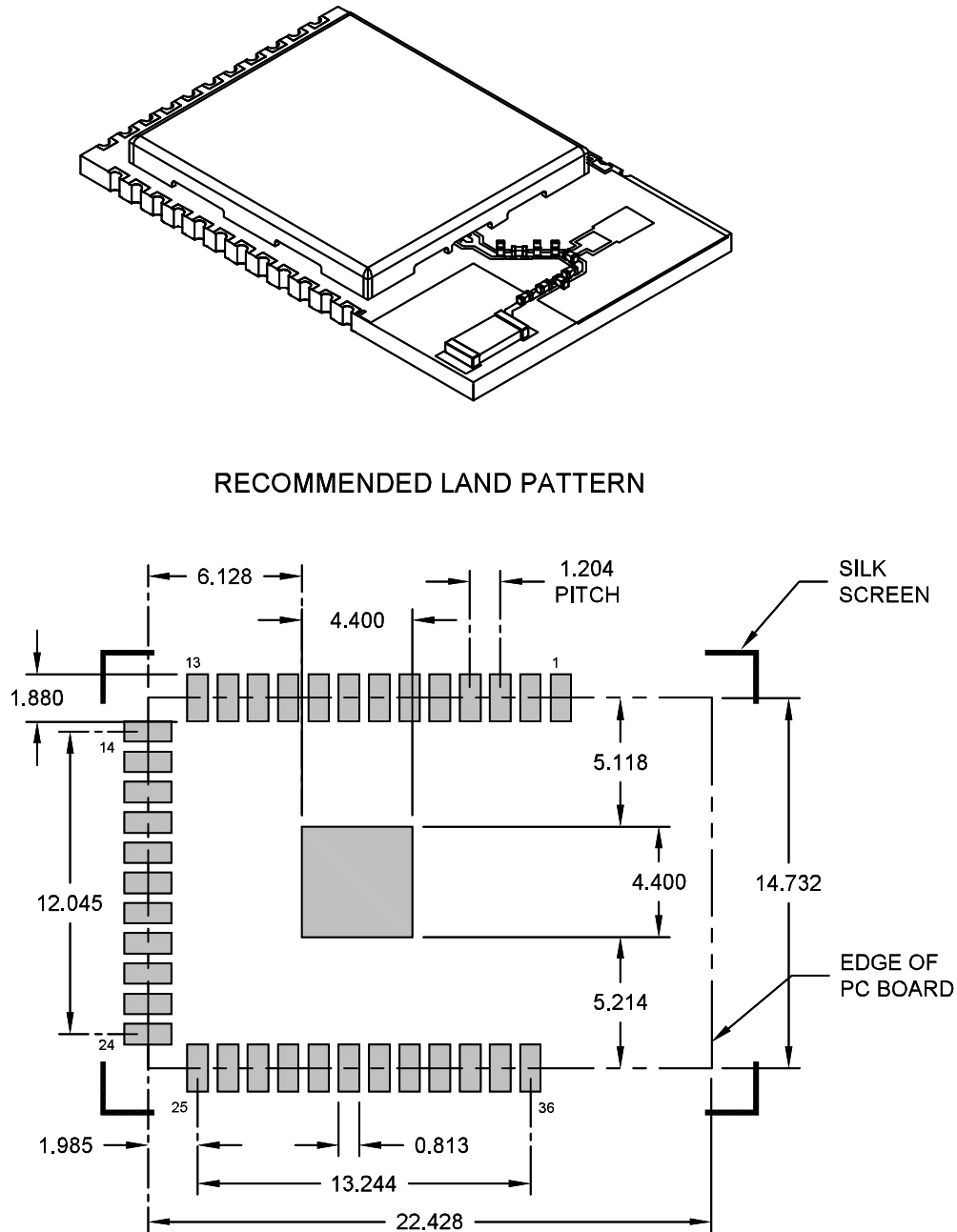
Figure 12-2. ATWINC3400-MR210CA Module Package Drawings - 3D View and Recommended Land Pattern
