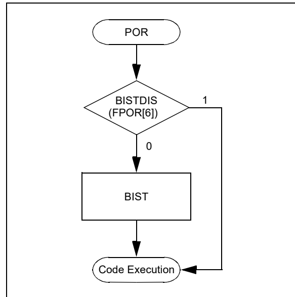
FIGURE 4-6: BIST FLOWCHART
