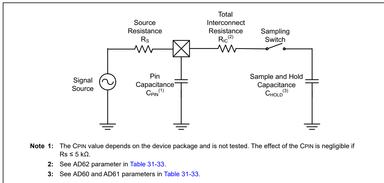
FIGURE 12-4: ADC ANALOG INPUT MODEL
