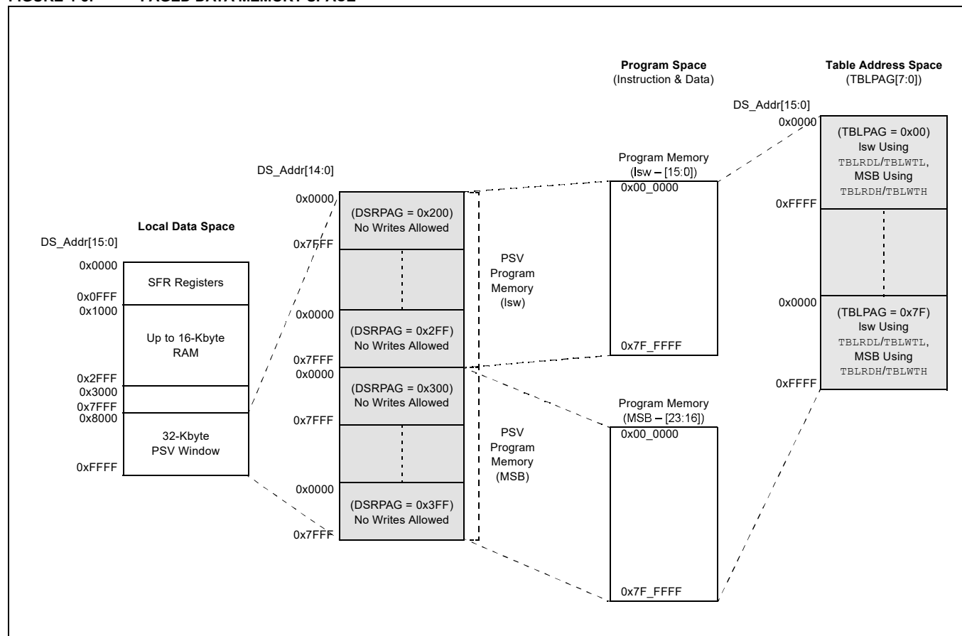
FIGURE 4-8: PAGED DATA MEMORY SPACE
