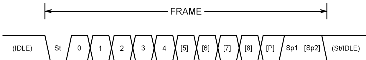
Figure 23-2. Frame Formats
