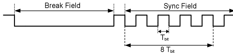
Figure 23-9. Auto-Baud Timing
