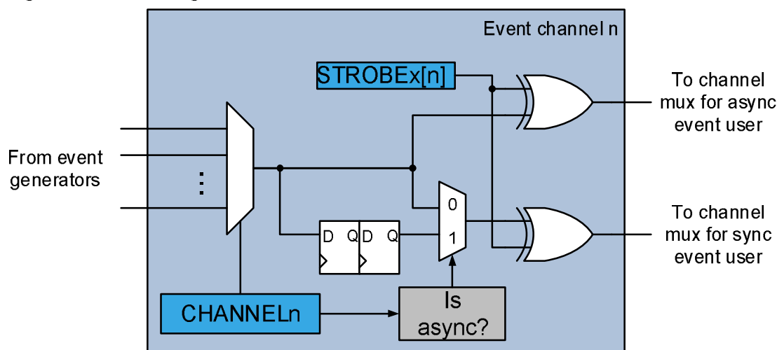
Figure 14-1. Block Diagram
