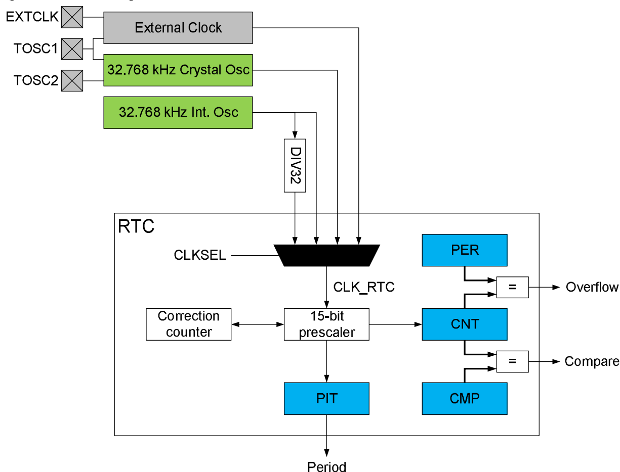
Figure 22-1. Block Diagram
