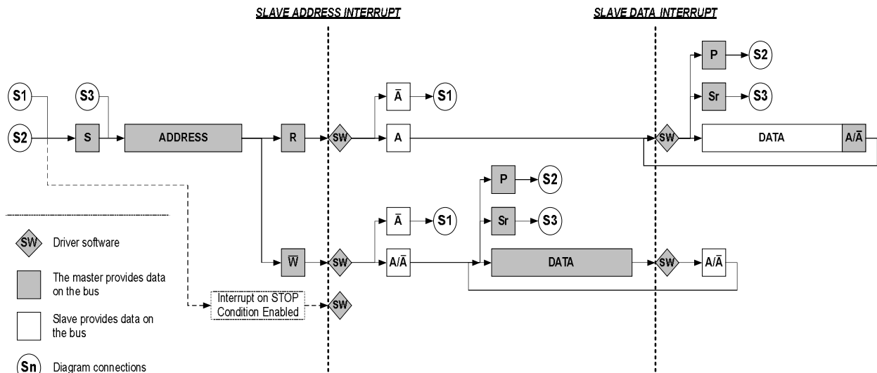
Figure 25-16. TWI Slave Operation
