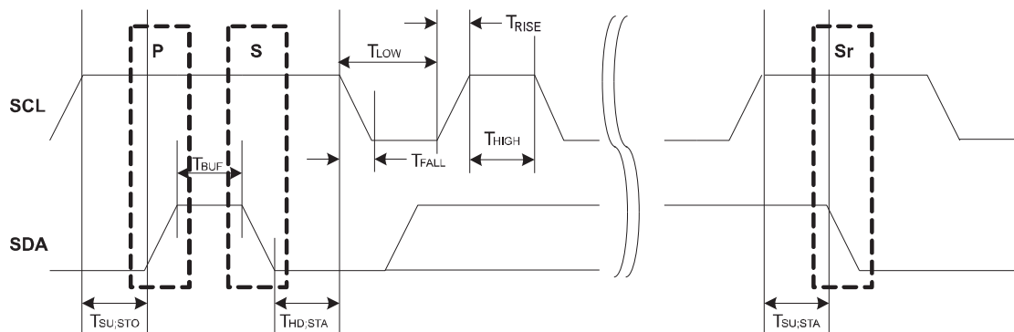
Figure 25-14. SCL Timing
