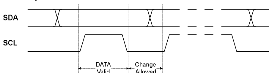
Figure 25-5. Data Validity
