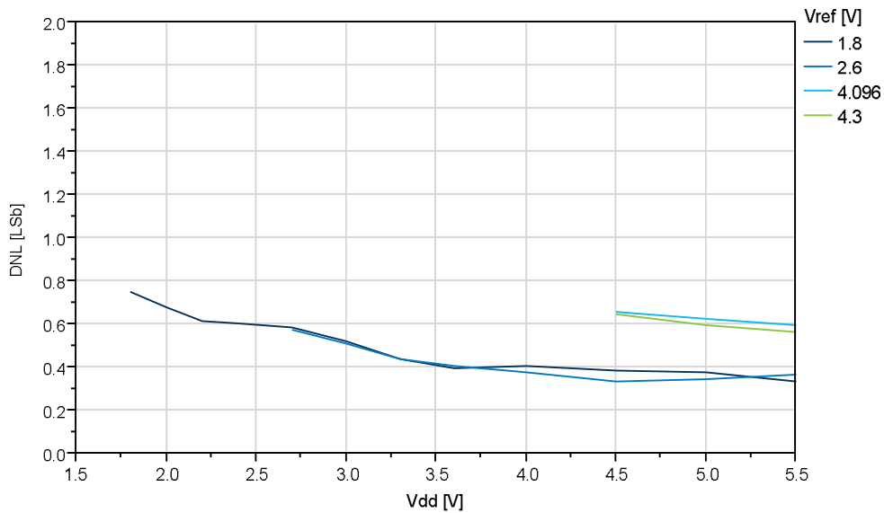
Figure 33-56. DNL vs. V_{DD} ( f_{ADC} = 115 ksp/s, T = 25^{\circ}C , REFSEL = External Reference)
