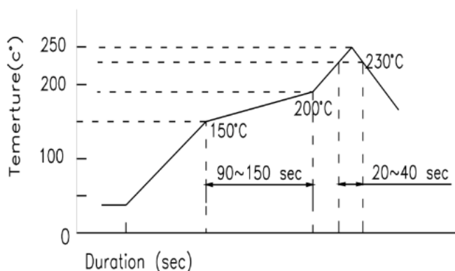
Fig.1. Recommended Reflow Temperature Profile
