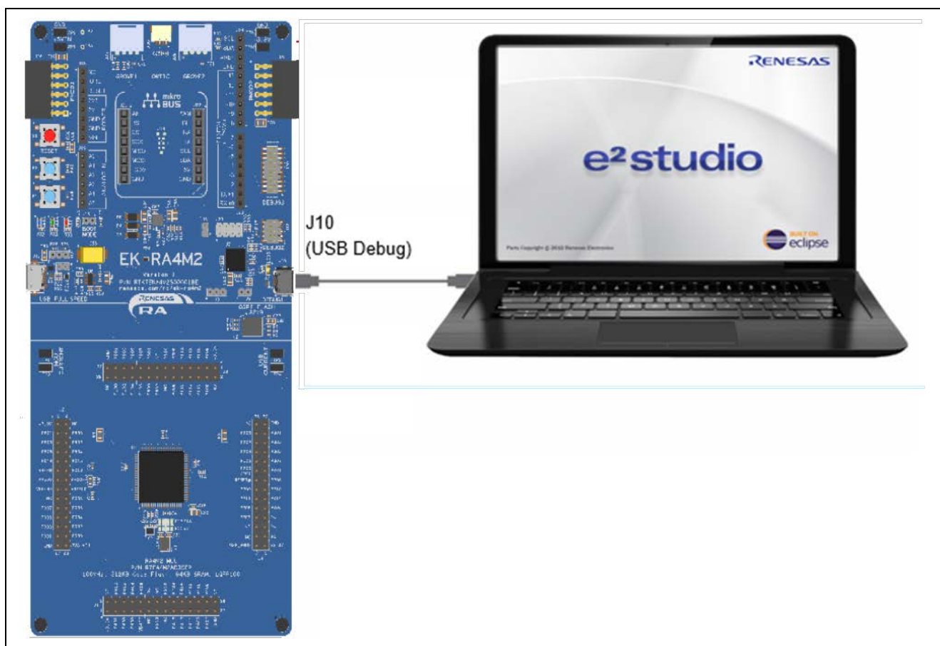
Figure 23. Connecting the EK-RA4M2 Board to the Host PC via USB Debug Port
