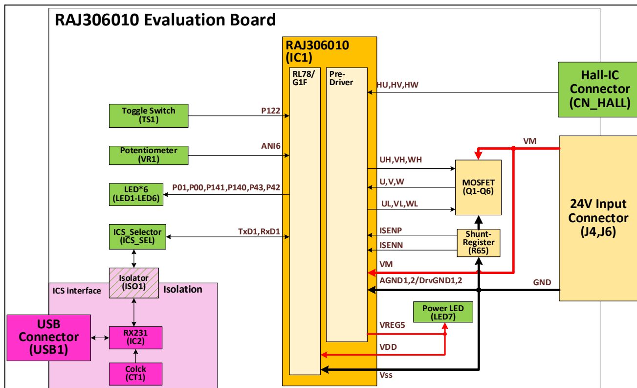
Figure 2-3. Outline functional block diagram
