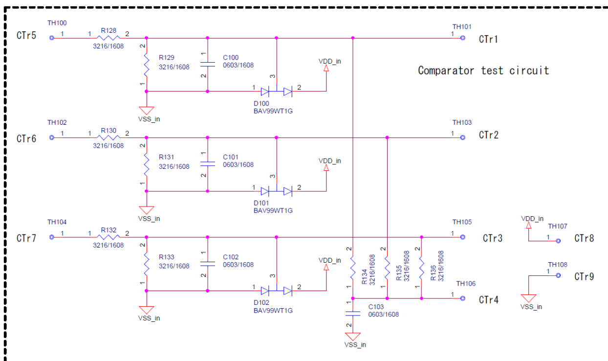
Figure 4-13. Spare_circuit
