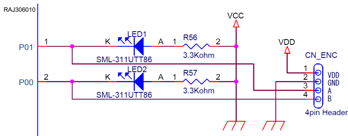
Figure 4-10. Encoder terminal
