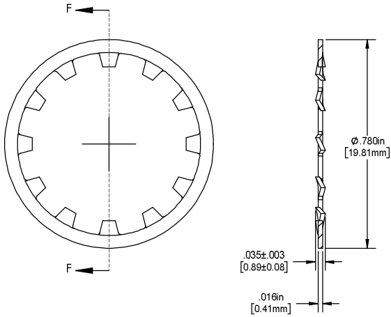
SECTION F-F
