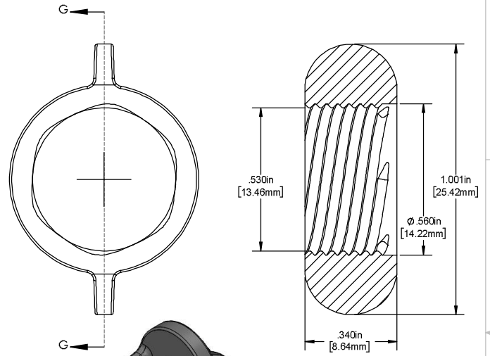
SECTION G-G
