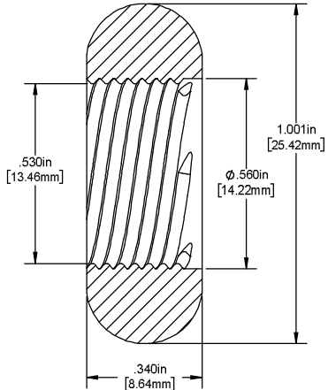
SECTION F-F
