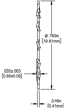
SECTION E-E
