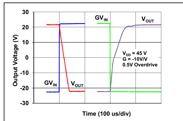
FIGURE 2-46: Output Overdrive Recovery vs. Time with G = -10 \text{ V/V}
