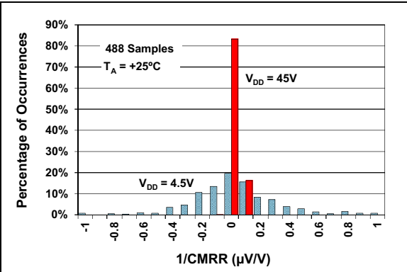
FIGURE 2-8: CMRR
