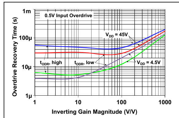
FIGURE 2-47: Output Overdrive Recovery Time vs. Inverting Gain
