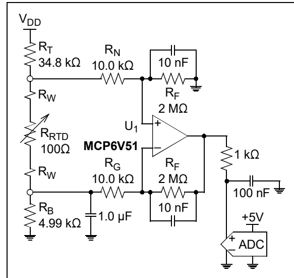
FIGURE 4-14: RTD Sensor
