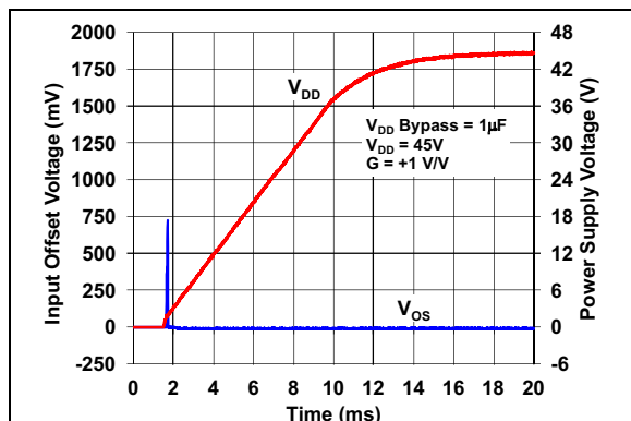
FIGURE 2-37: Input Offset Voltage vs. Time at Power-up
