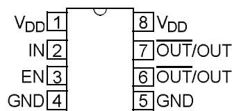
MCP14A0901/MCP14A0902 MSOP/SOIC
