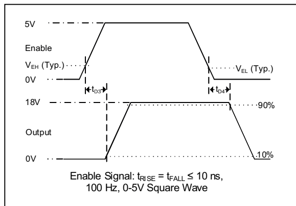
FIGURE 4-3: Enable Timing Waveform.
