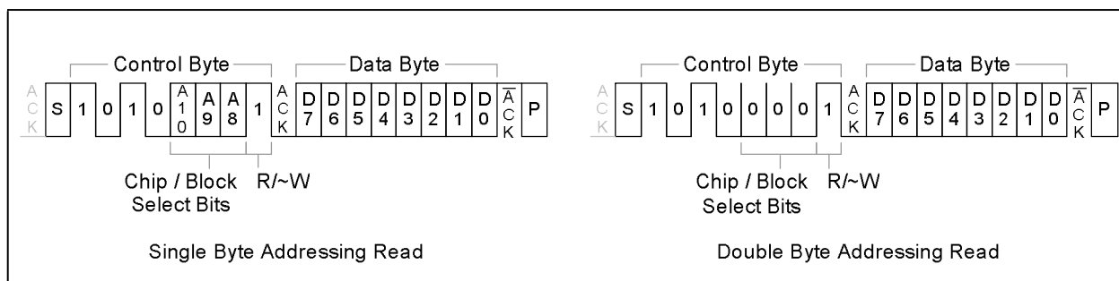
FIGURE 13-4: I 2 C EEPROM BYTE READ
