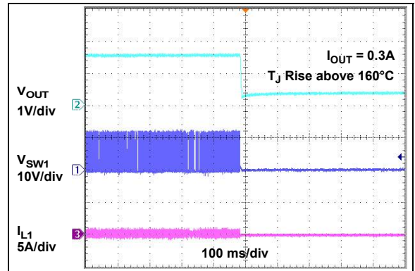
FIGURE 2-47: Thermal Shutdown.
