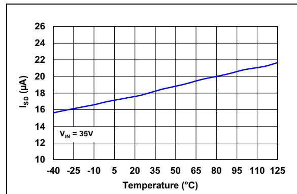
FIGURE 2-6: V_{IN} Shutdown Current vs. Temperature.
