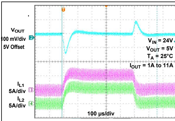
FIGURE 2-38: Load Transient without Droop ( V_{IN} = 24V , I_{OUT} = 1A to 11A ).
