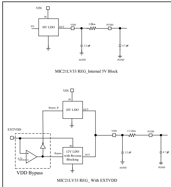
FIGURE 4-14: MIC21LV33 EXTVDD.
