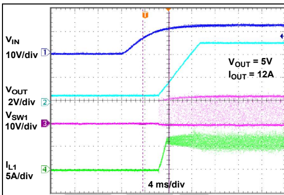
FIGURE 2-45: Power-up with V_{IN} and 12A Load.
