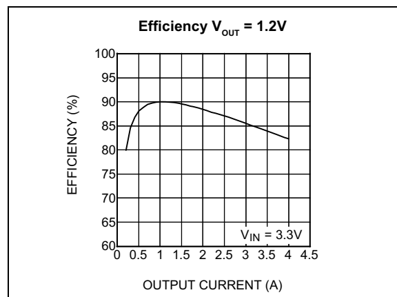
FIGURE 5-1: Efficiency Curve.
