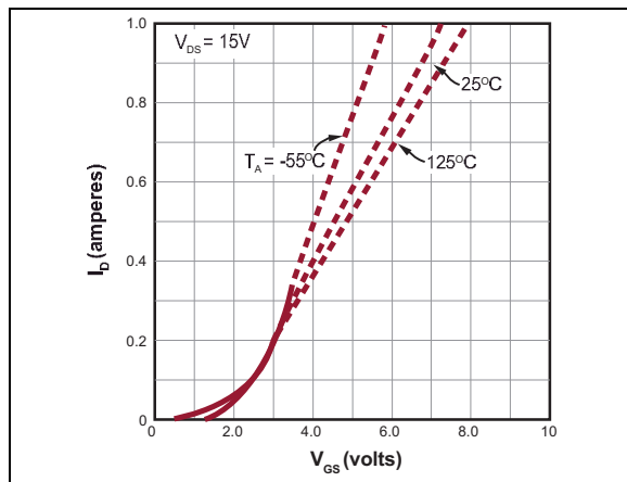
FIGURE 2-8: Transfer Characteristics.
