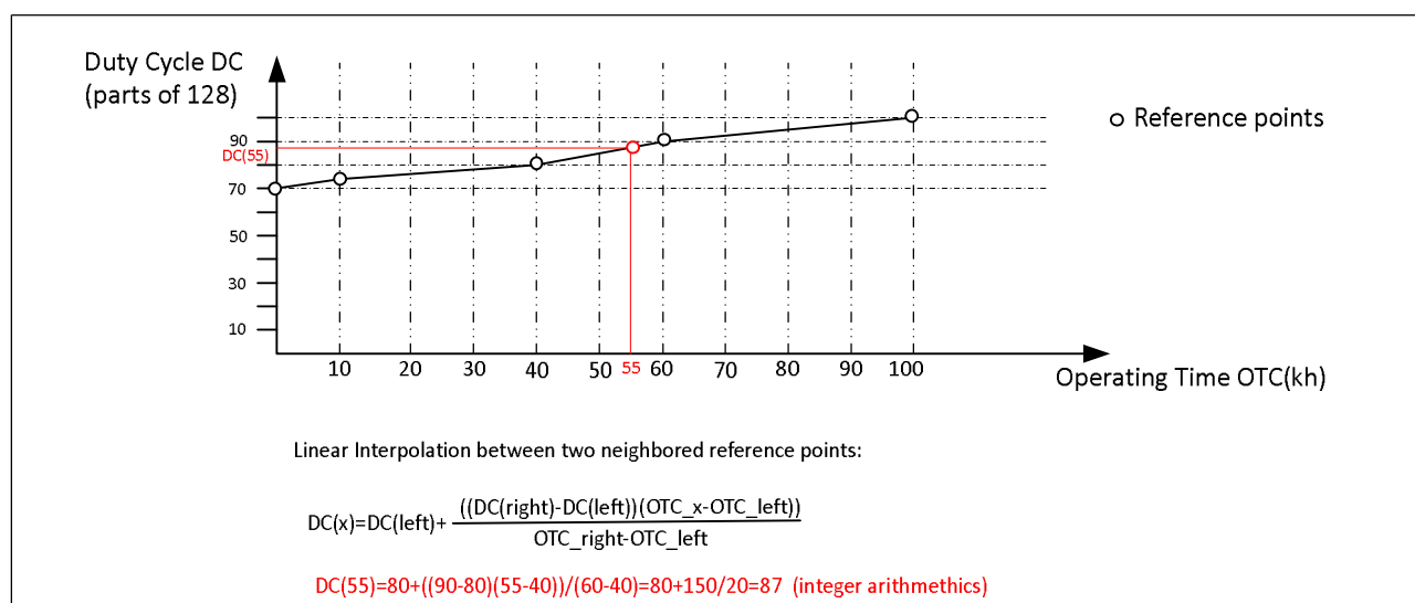
Figure 11 Constant Lumen Output Principle
