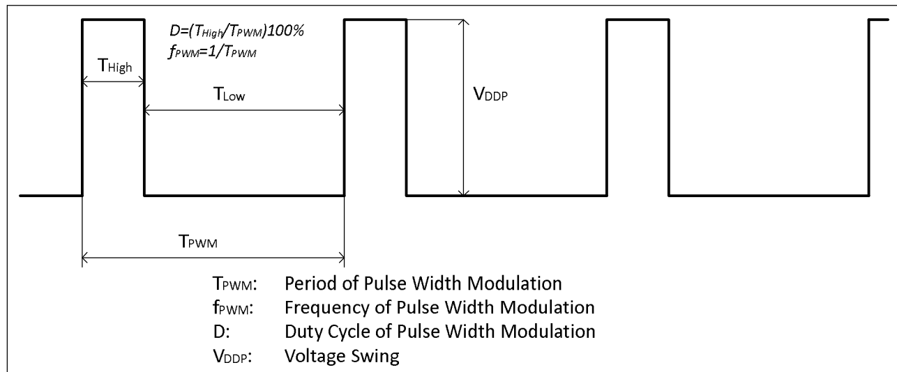
Figure 14 PWM Output Characteristics
