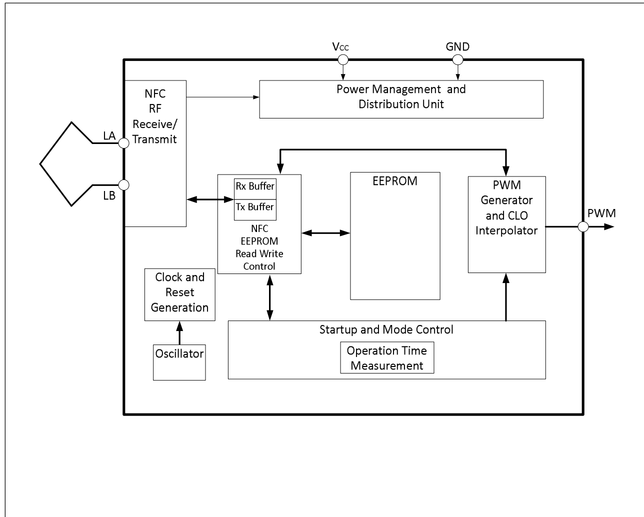
Figure 3 Block Diagram
