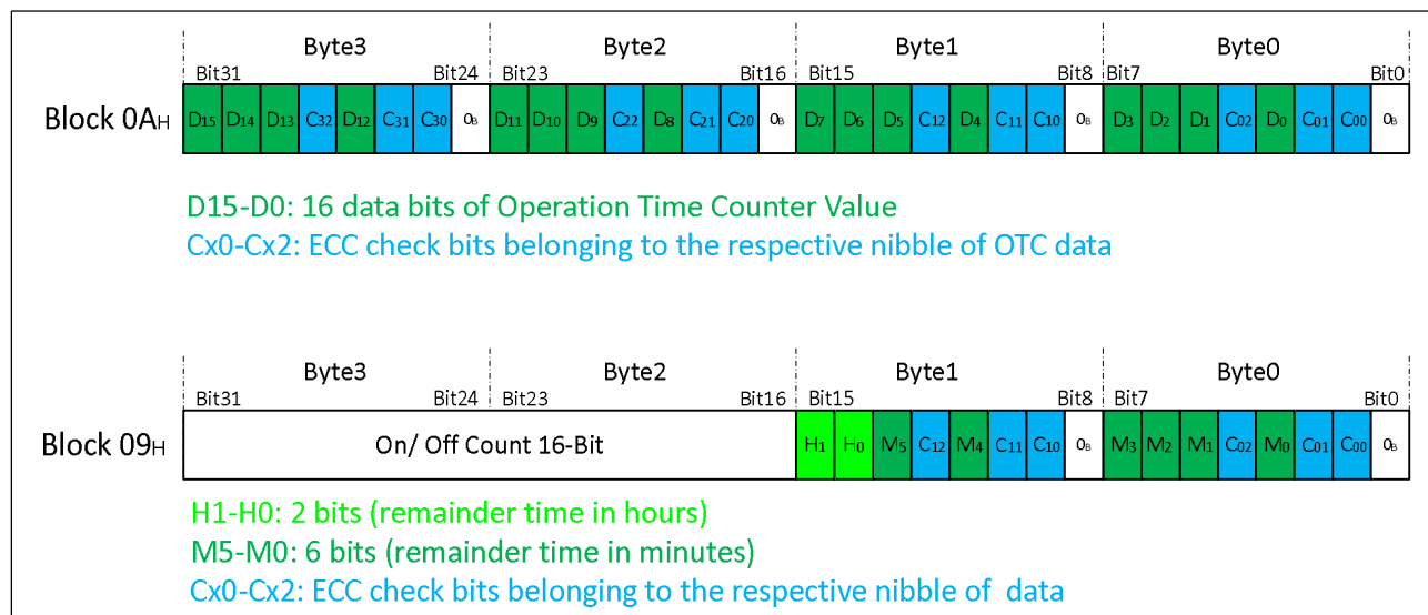
Figure 13 OTC related NVM content
