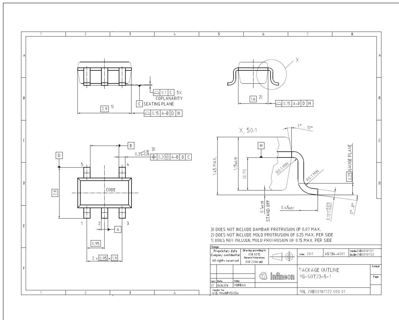
Figure 15 Package Outline PG-SOT23-5-1
