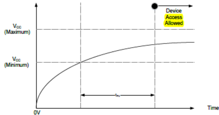
Figure 1: Power-Up Behavior
