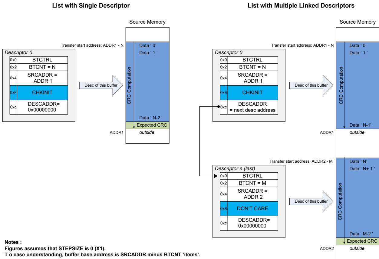
Figure 25-21. CRC Computation and Check with Single or Linked Transfers
