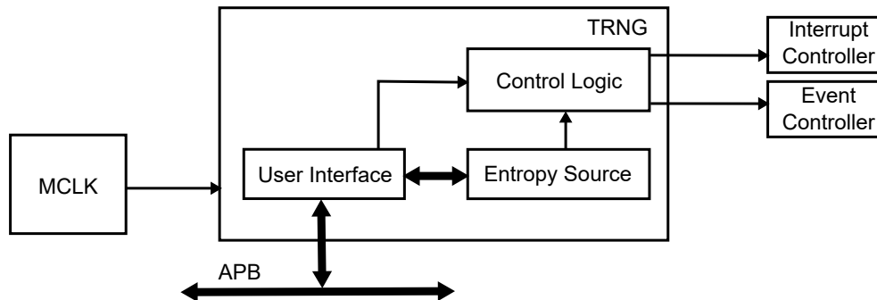
Figure 48-1. TRNG Block Diagram.
