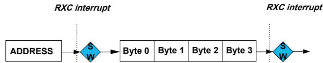
Figure 33-9. 32-bit Extension Client Operation
