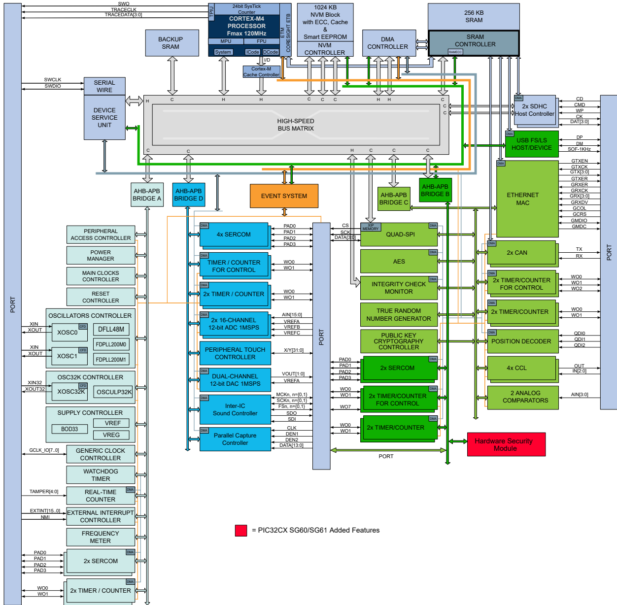
Figure 3-1. PIC32CX SG41/SG60/SG61 Block Diagram
