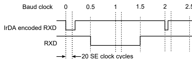
Figure 32-13. IrDA Receive Decoding
