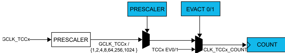
Figure 45-2. Prescaler
