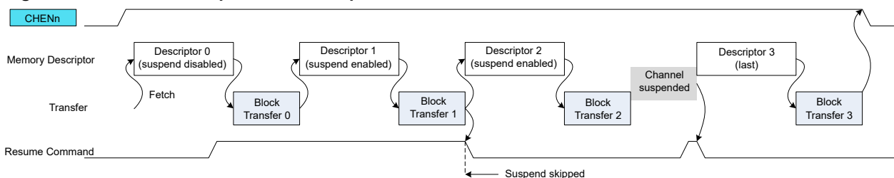
Figure 25-11. Channel Suspend/Resume Operation
