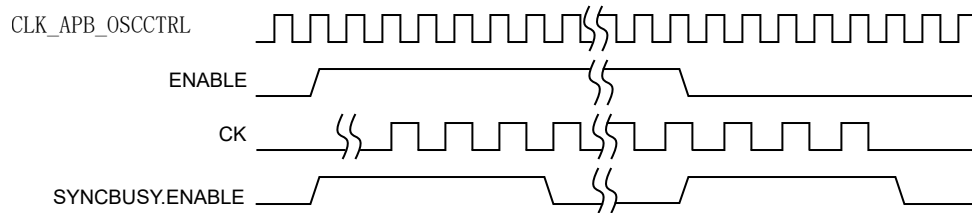
Figure 18-3. Enable Synchronization Busy Operation
