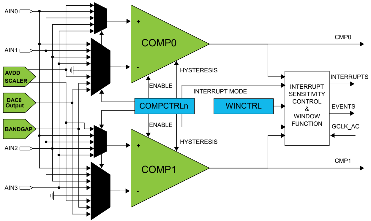
Figure 52-1. Analog Comparator Block Diagram
