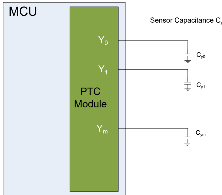
Figure 54-4. Self-Capacitance Sensor Arrangement
