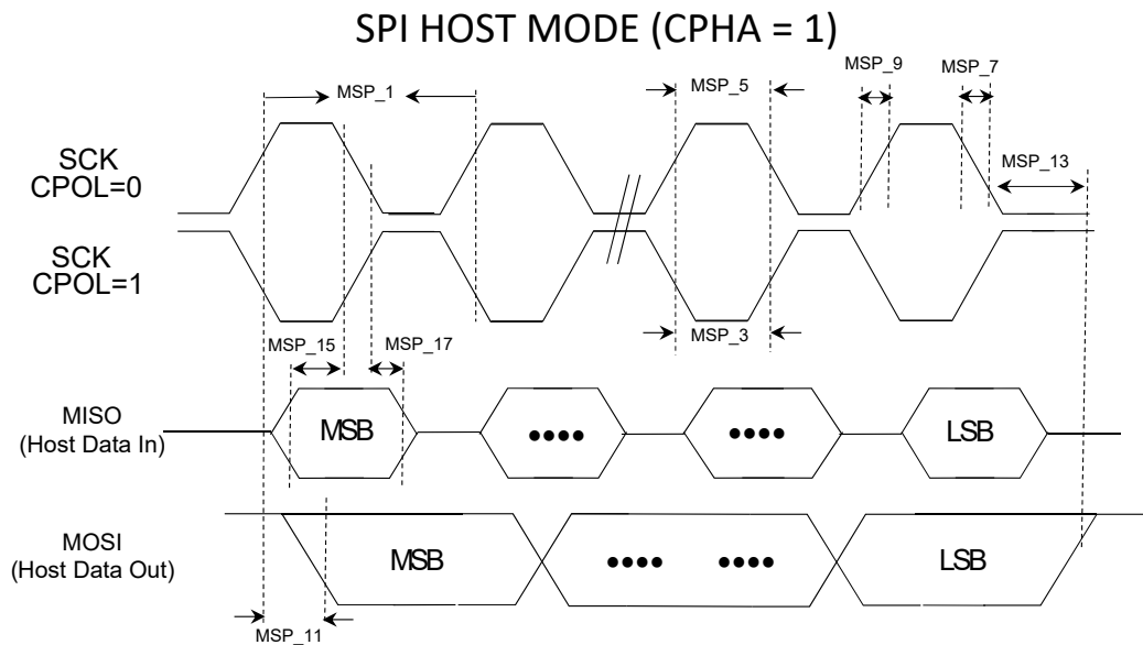
Figure 56-2. SPI Host Module (CPHA=1) Timing Diagrams
