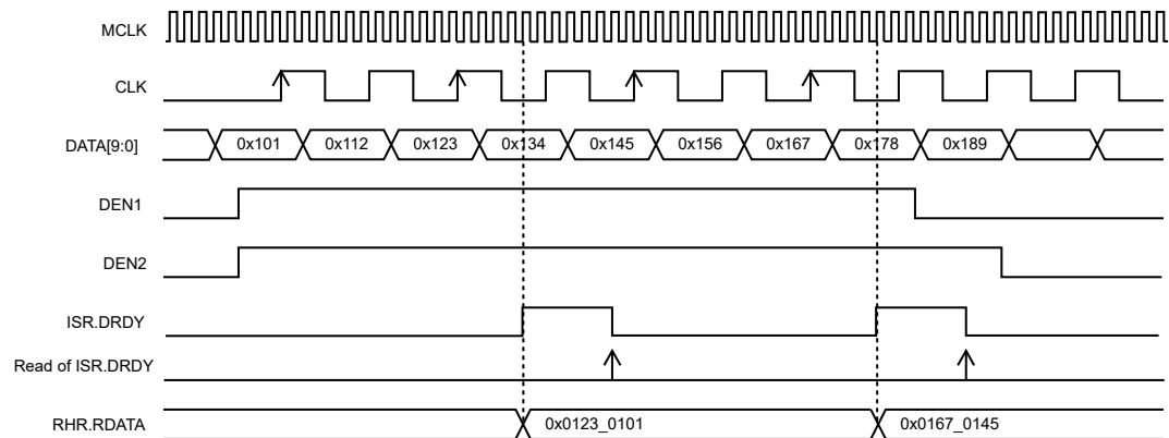
Figure 39-11. PCC Waveforms (ISIZE = 10_BITS, DSIZE = 2_DATA, ALWAYS = 0, HALFS = 1, FRSTS = 0, SCALE = 1)
