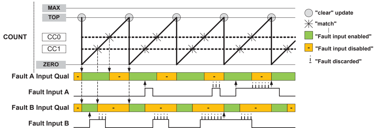
Figure 45-24. Fault Qualification in RAMP2 Operation with Inverted Polarity
