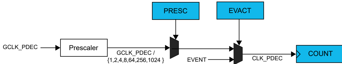
Figure 42-2. Prescaler Selection
