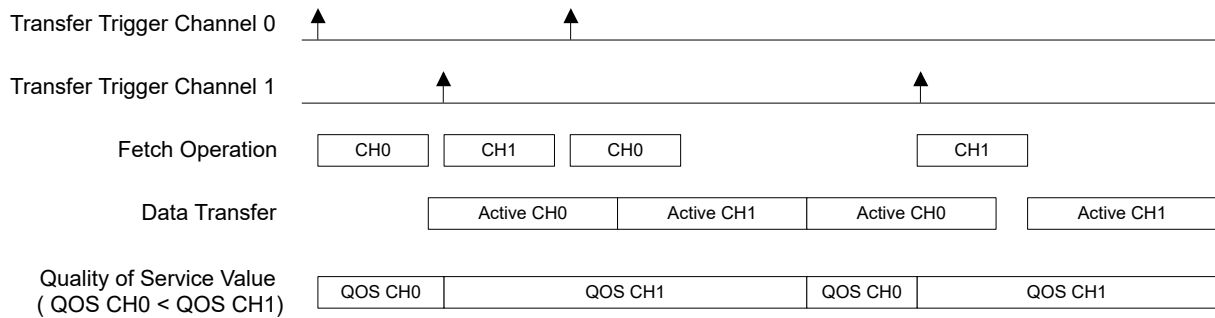
Figure 25-10. Quality of Service
