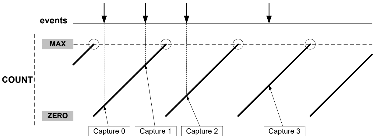
Figure 45-14. Input Capture Timing
