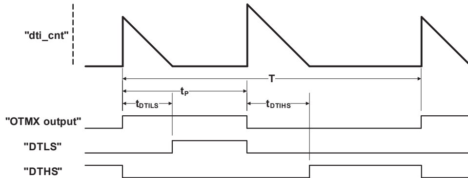
Figure 45-36. Dead-Time Generator Timing Diagram
