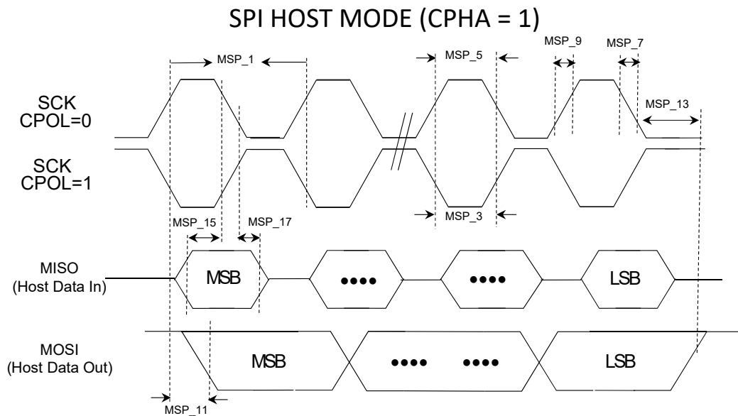
Figure 55-2. SPI Host Module (CPHA = 1) Timing Diagrams
