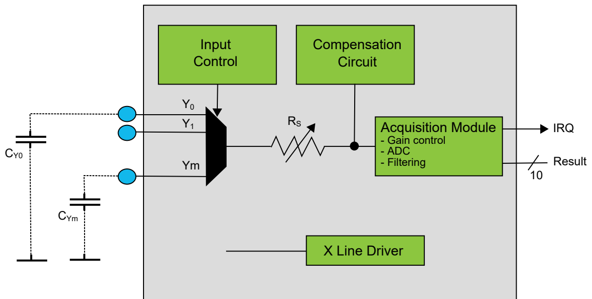
Figure 54-2. PTC Block Diagram Self Capacitance
