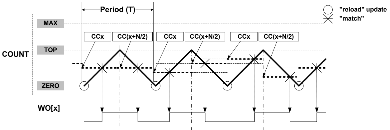
Figure 45-8. Dual-Slope Critical Pulse Width Modulation (N=CC_NUM)
