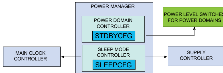
Figure 20-1. PM Block Diagram
