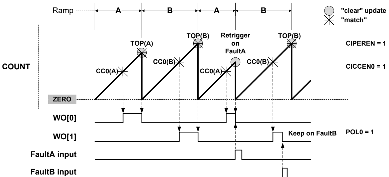
Figure 45-19. RAMP2 Alternate Operation
