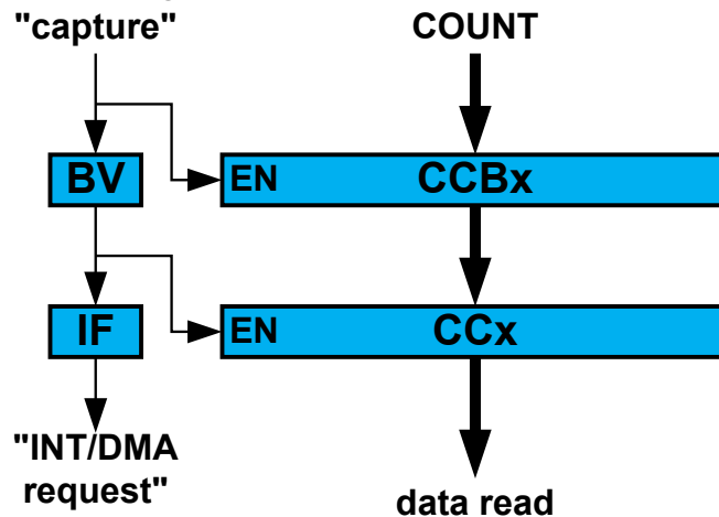
Figure 44-11. Capture Double Buffering
