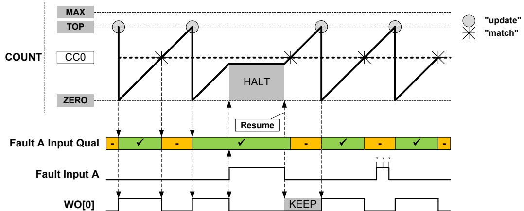
Figure 45-31. Waveform Generation with Fault Qualification, Halt, and Restart Actions
