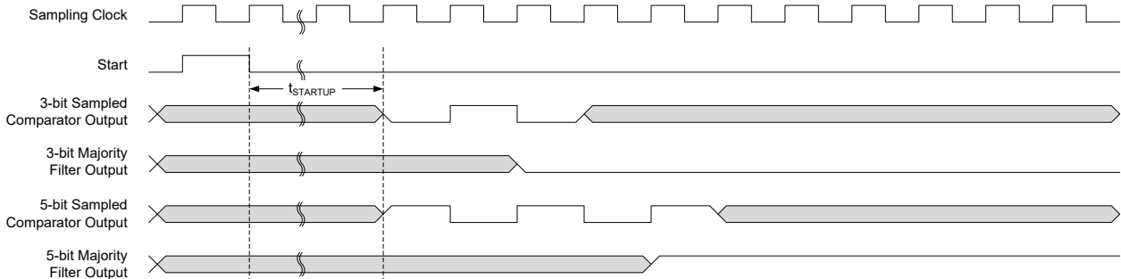
Figure 52-7. Single-Shot Filtering
