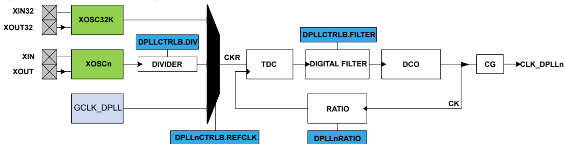
Figure 18-2. DPLL Block Diagram
