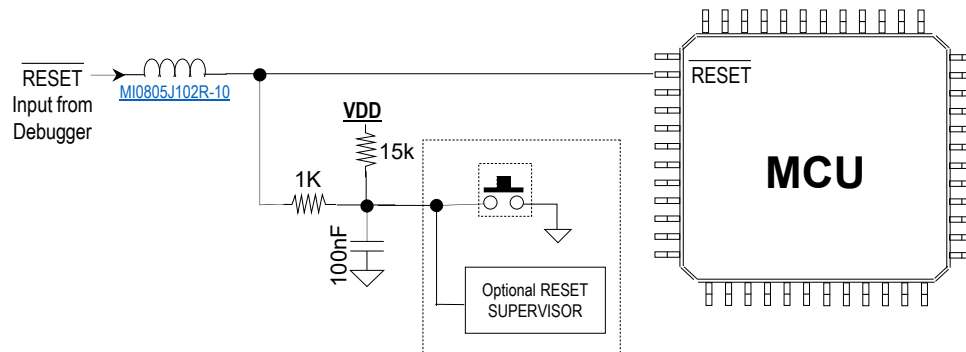
Figure 58-7. External Reset Circuit Schematic
