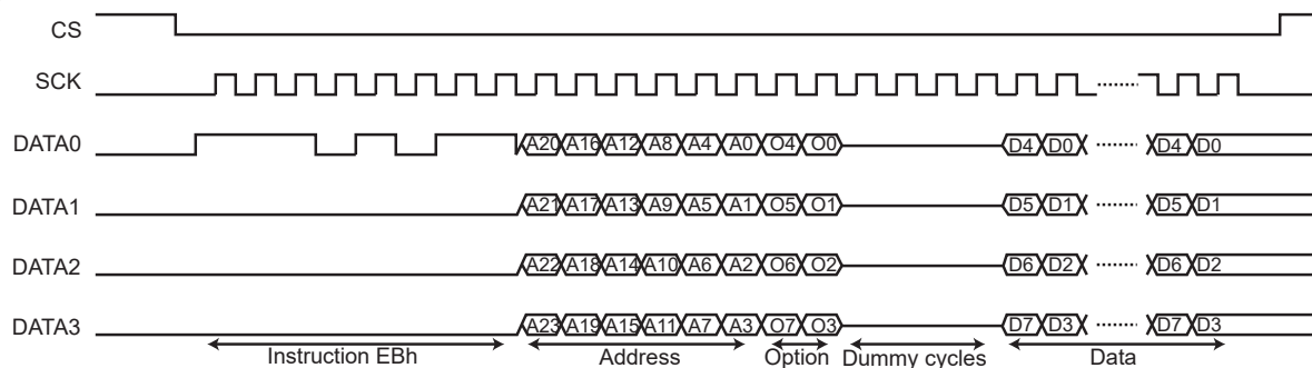
Figure 35-9. Instruction Frame
