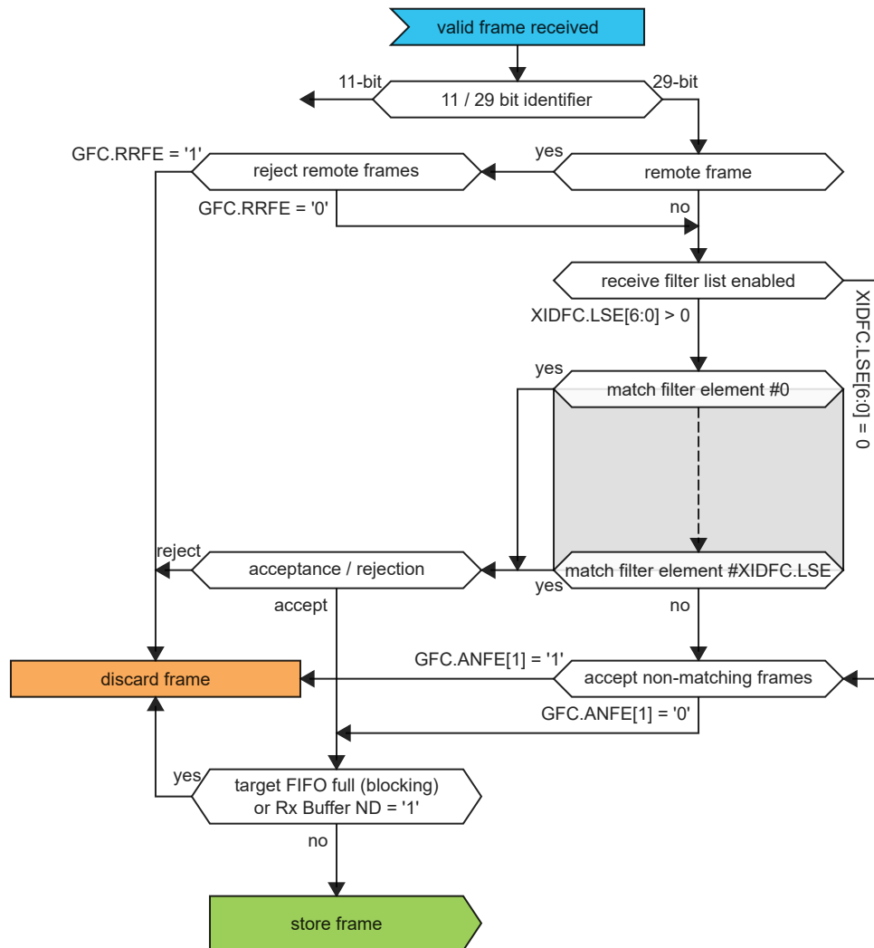
Figure 38-6. Extended Message ID Filtering
