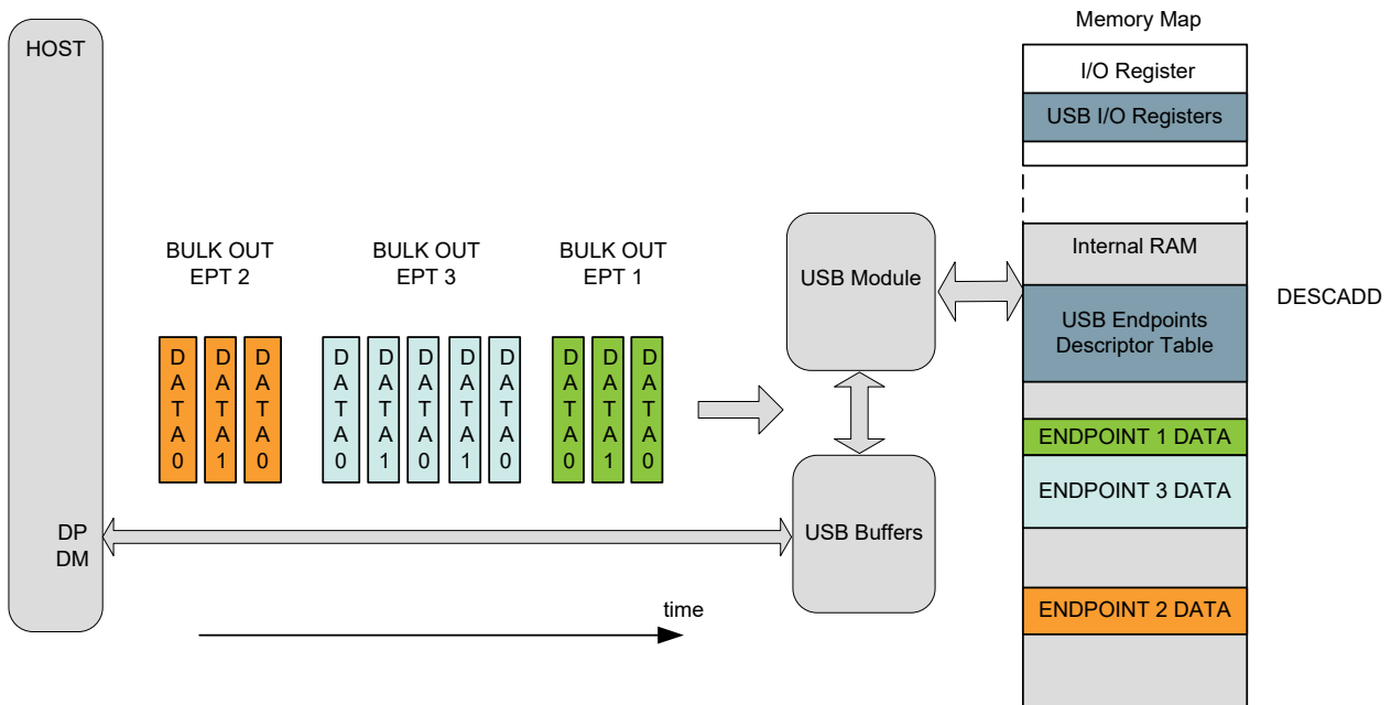
Figure 40-4. OUT Transfer: Data Packet Host to USB Device
