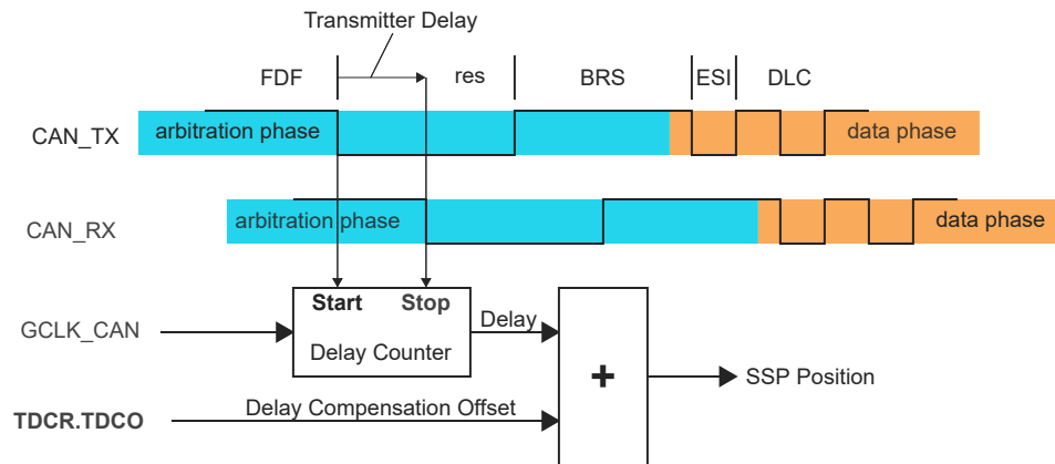
Figure 38-2. Transceiver delay measurement
