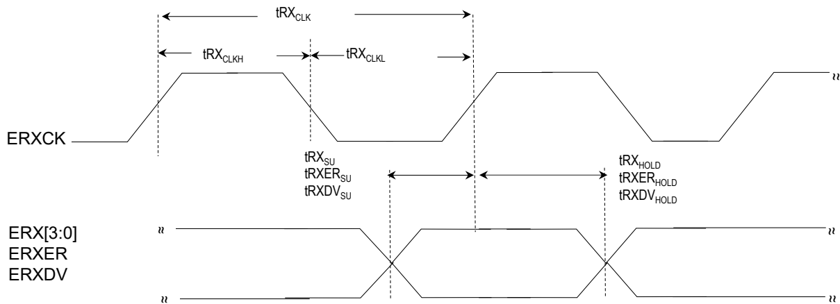
Figure 55-23. MII Receive Ethernet Module Timing Diagram (Media-Independent Interface)
