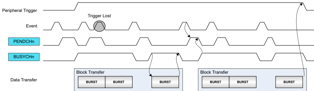
Figure 25-12. Burst Event Trigger Action
