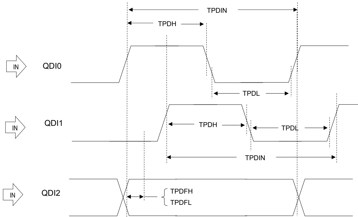
Figure 55-27. Position Decoder (PDEC) Input Timing Diagrams
