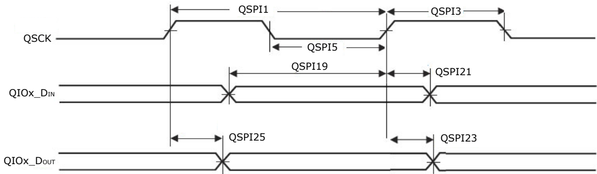
Figure 55-13. QSPI DDR Mode 0 Write Timing Diagram
