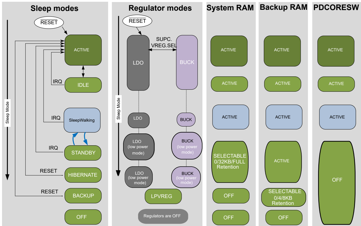
Figure 20-2. Operating Conditions and SleepWalking
