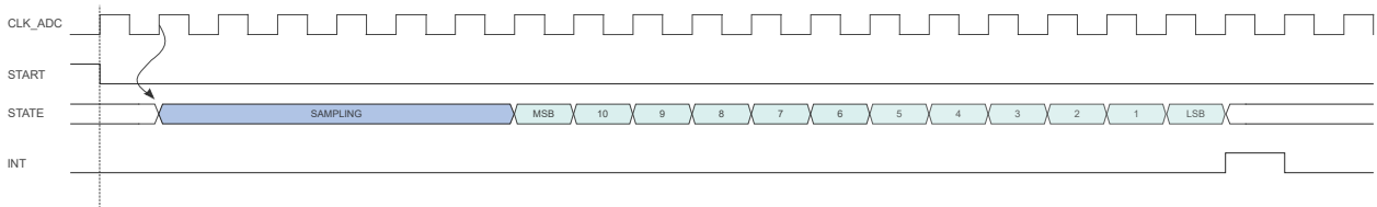
Figure 51-4. ADC Timing for One Conversion with Increased Sampling Time, 12-bit
