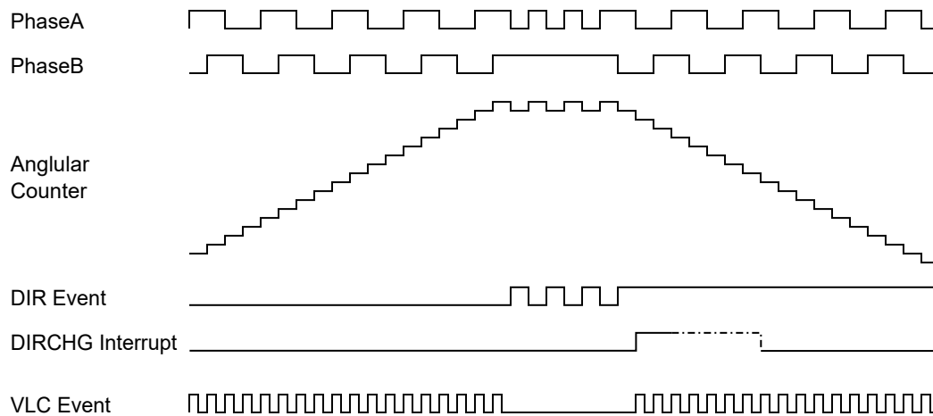
Figure 42-8. Rotation Direction Change
