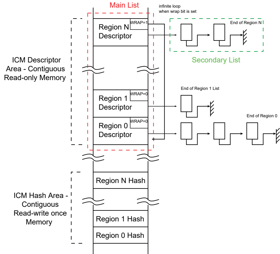
Figure 49-2. ICM Region Descriptor and Hash Areas
