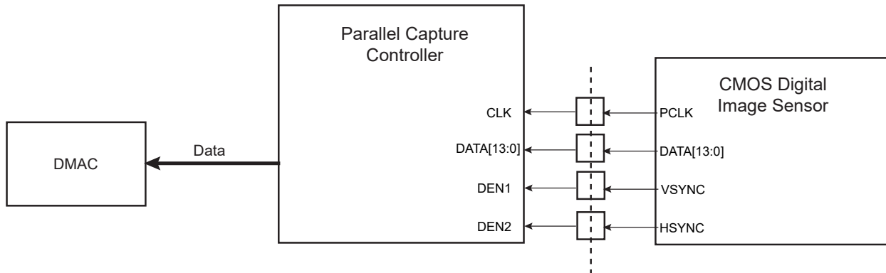
Figure 39-2. Parallel Capture Controller Connection with CMOS Digital Image Sensor
