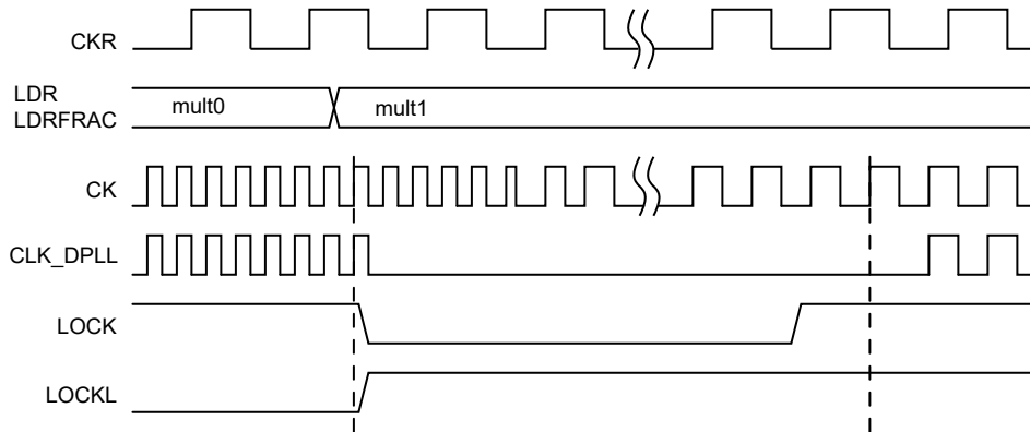
Figure 18-7. RATIOCTRL Register Update Operation
