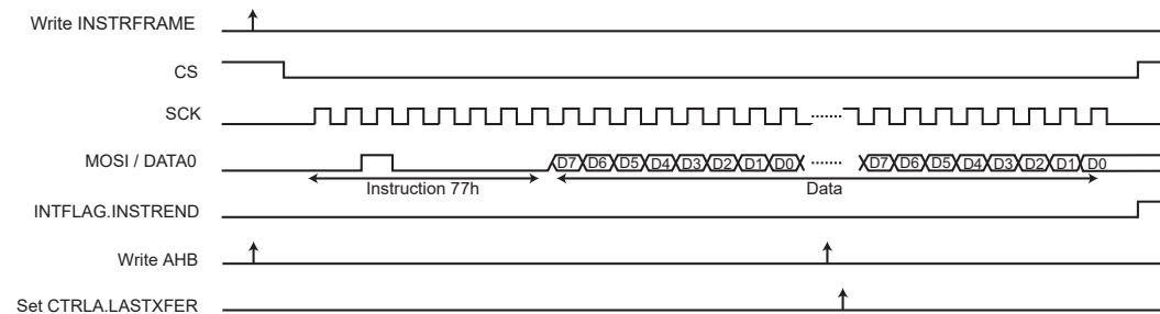
Figure 35-15. Instruction Transmission Waveform 4
