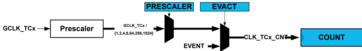
Figure 44-2. Prescaler
