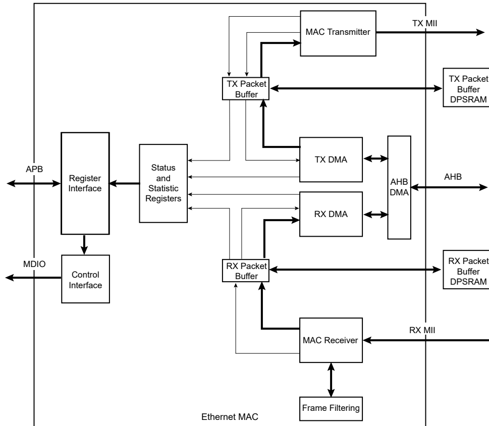
Figure 41-2. Data Paths with Packet Buffers Included
