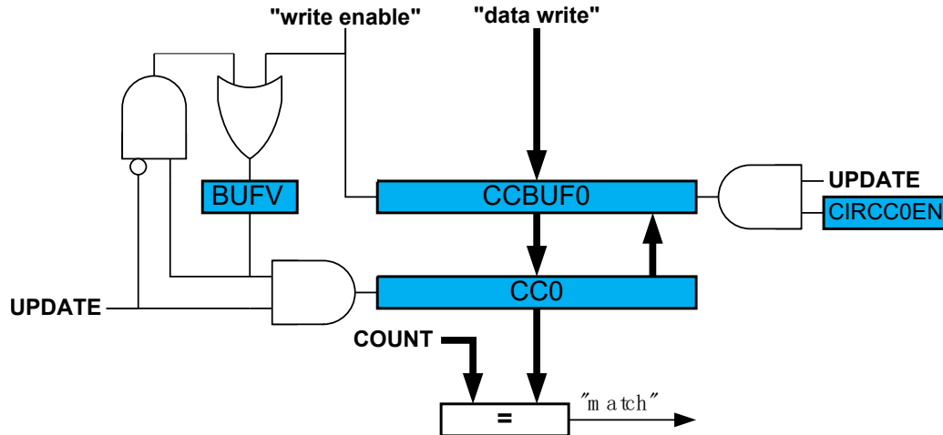
Figure 45-17. Circular Buffer on Channel 0
