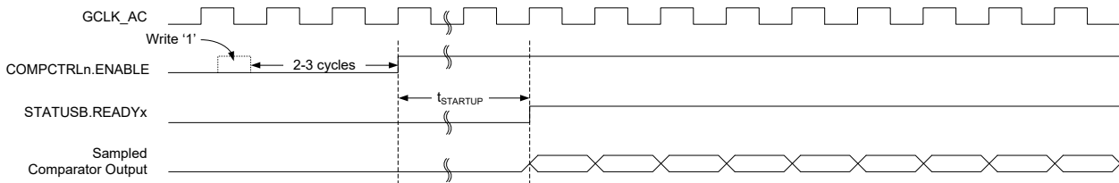
Figure 52-9. Continuous Mode SleepWalking
