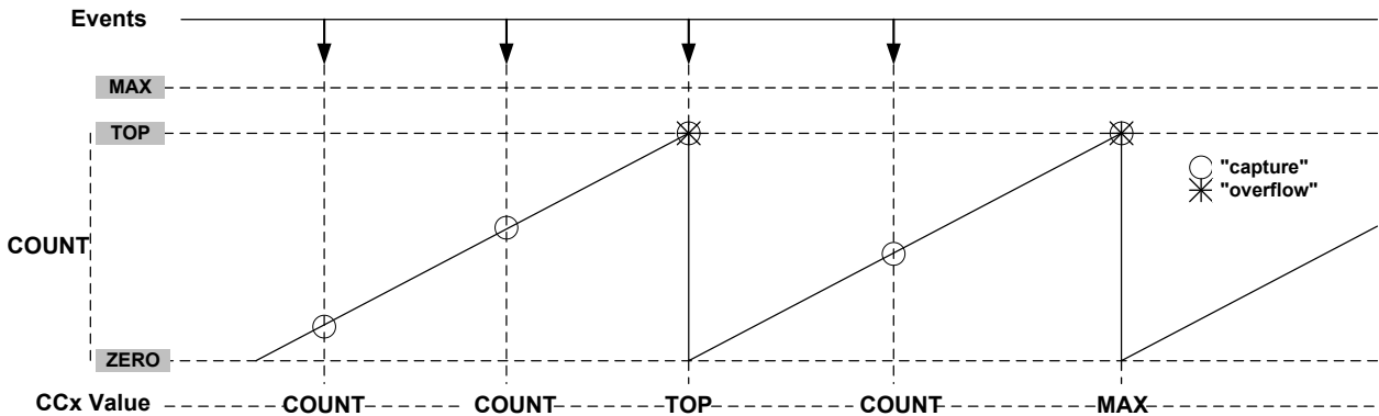
Figure 45-33. Time-Stamp
