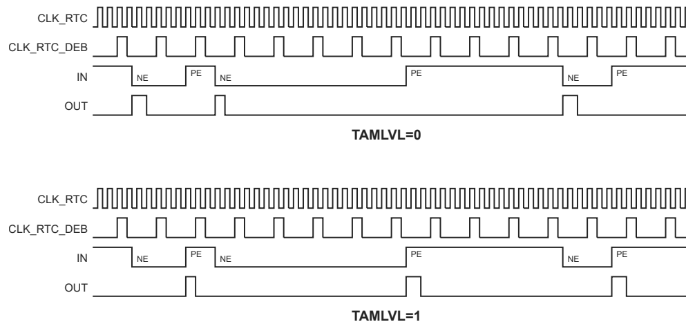
Figure 23-5. Edge Detection with Debouncer Disabled
