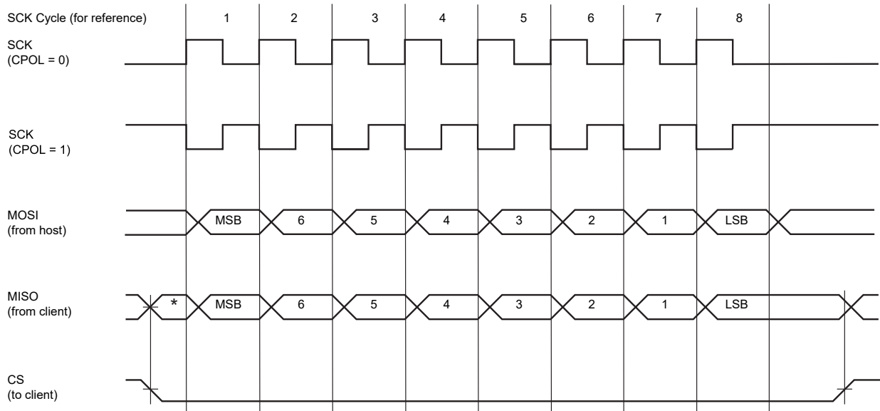
Figure 35-4. QSPI Transfer Modes (BAUD.CPHA = 1, 8-bit transfer)
