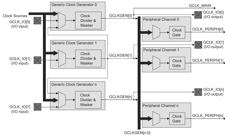
Figure 15-2. Generic Clock Controller Block Diagram
