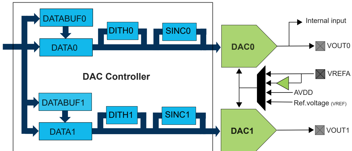
Figure 53-1. DAC Controller Block Diagram
