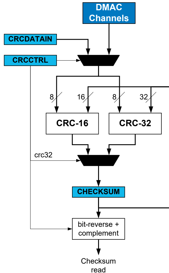
Figure 25-19. CRC Generator Block Diagram
