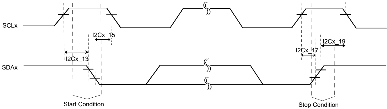
Figure 55-11. I 2 C Bus Data Client Mode Timing Diagrams
