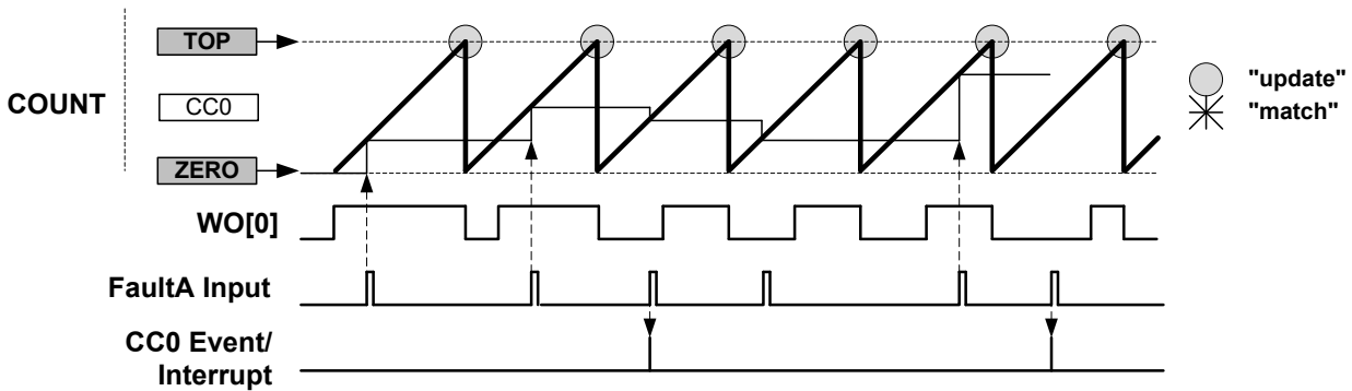
Figure 45-29. Capture Action “DERIV0”
