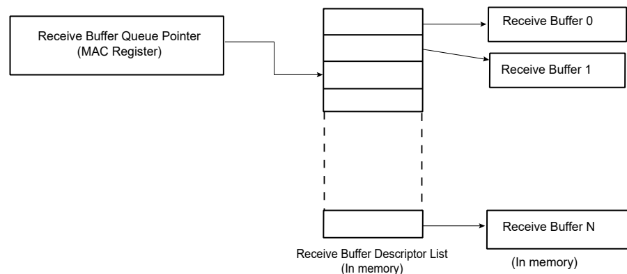
Figure 41-3. Receive Buffer List
