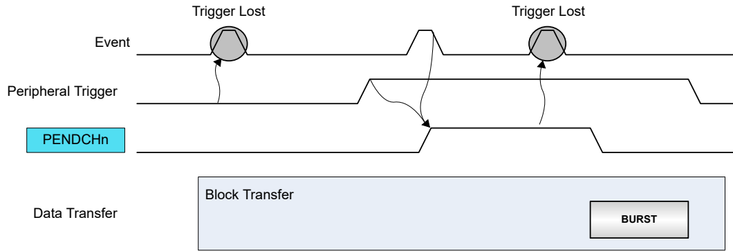
Figure 25-13. Periodic Event with Burst Peripheral Triggers
