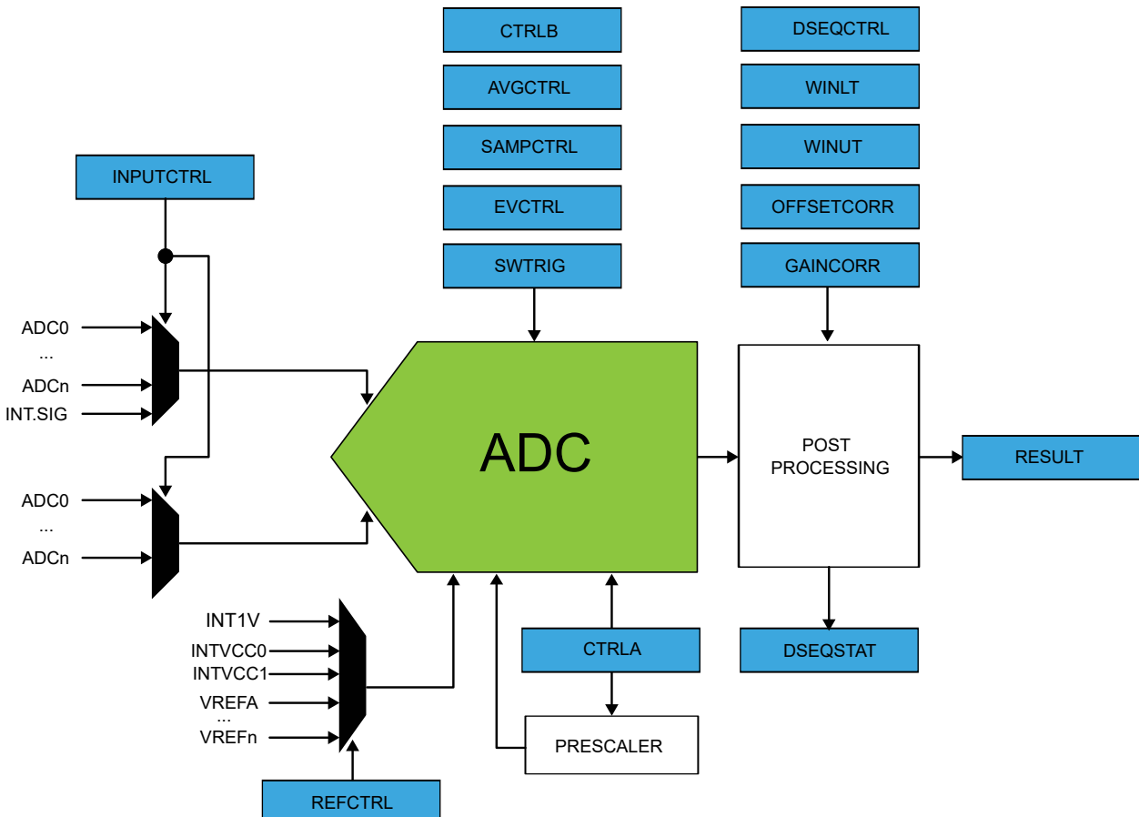
Figure 51-1. ADC Block Diagram
