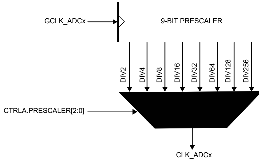
Figure 51-2. ADC Prescaler
