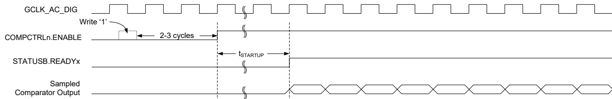
Figure 52-2. Continuous Measurement Example
