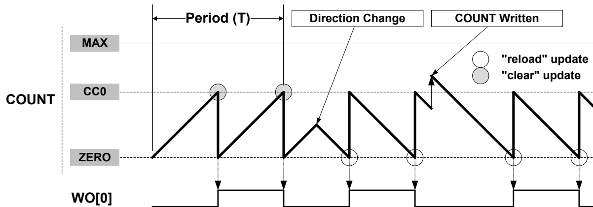
Figure 44-5. Match Frequency Operation
