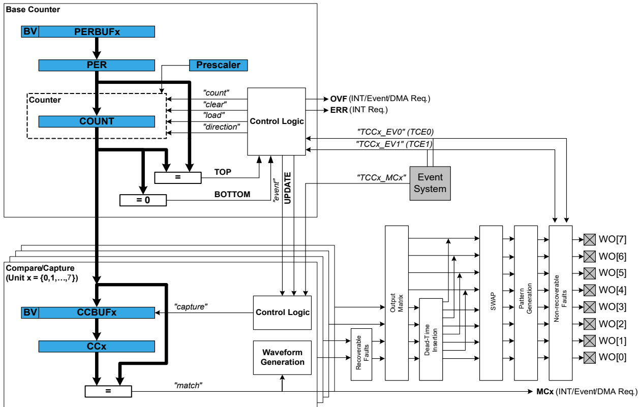
Figure 45-1. Timer/Counter for Control Applications - Block Diagram
