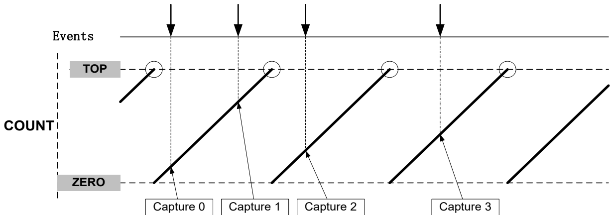
Figure 44-12. Input Capture Timing
