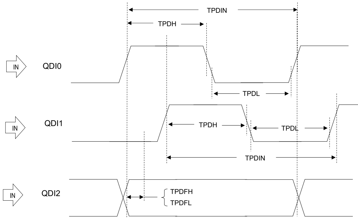
Figure 56-18. Position Decoder (PDEC) Input Timing Diagrams
