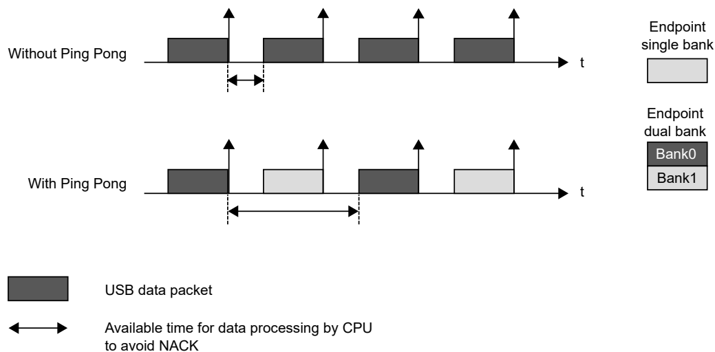
Figure 40-6. Ping-Pong Overview
