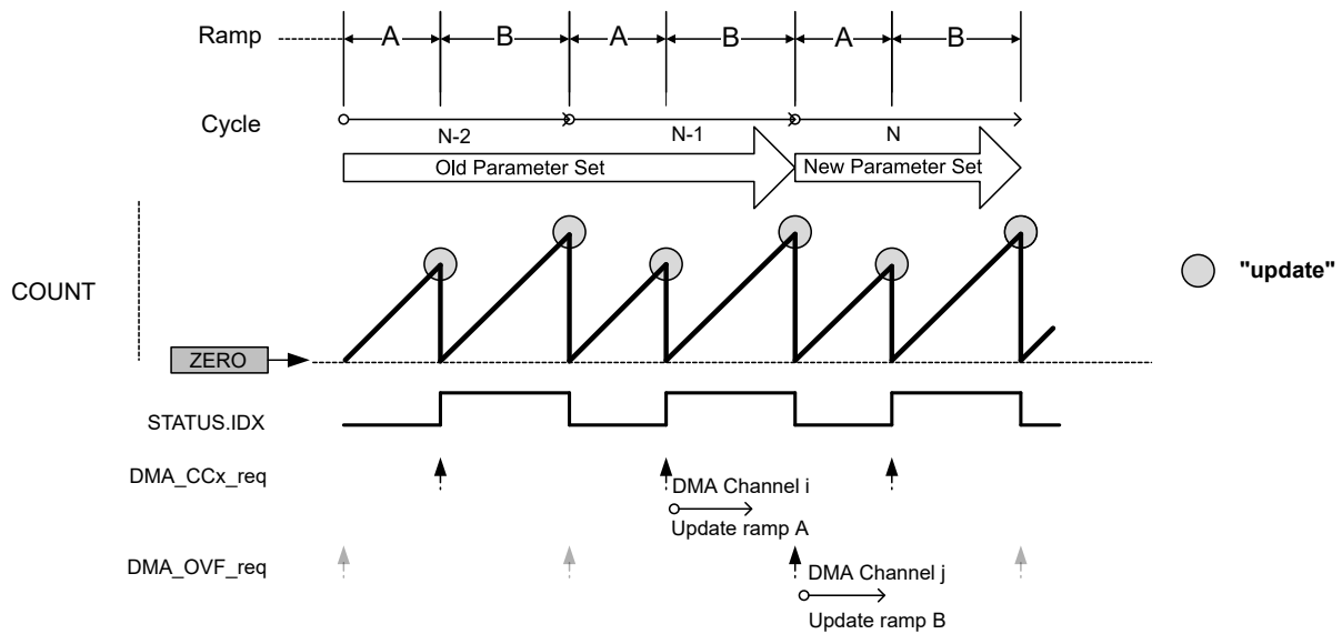
Figure 45-38. DMA Triggers in RAMP and RAMP2 Operation Mode and Circular Buffer Enabled
