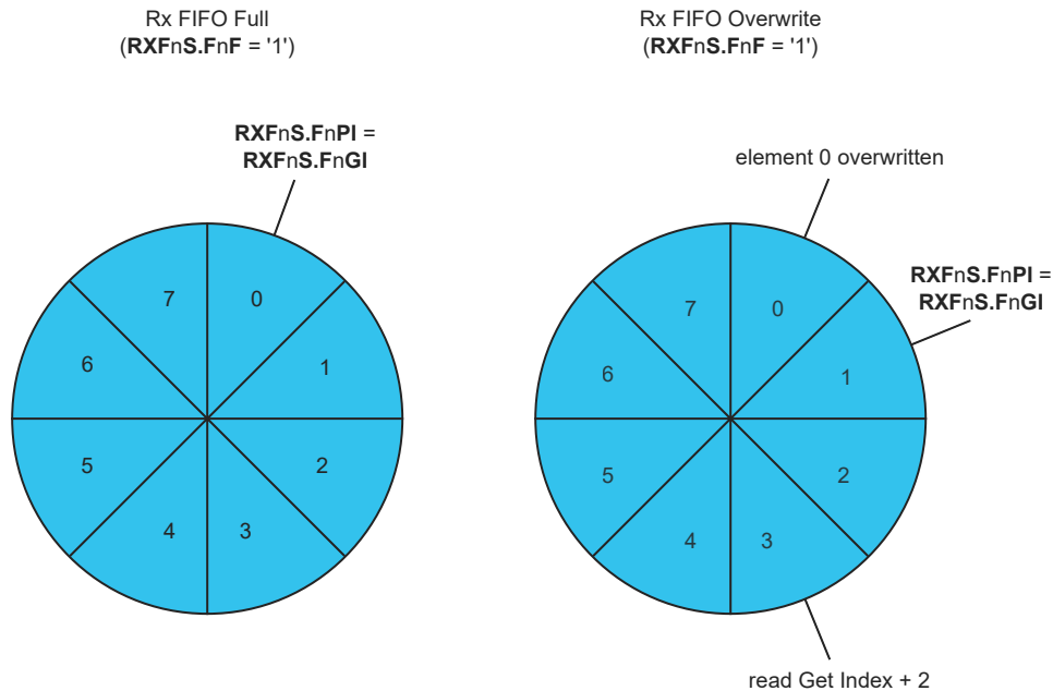
Figure 38-8. Rx FIFO Overflow Handling
