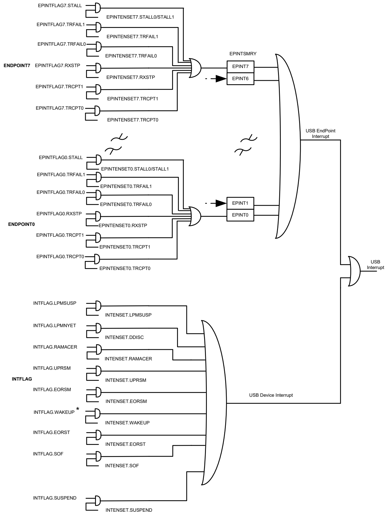
Figure 40-9. Device Interrupt
