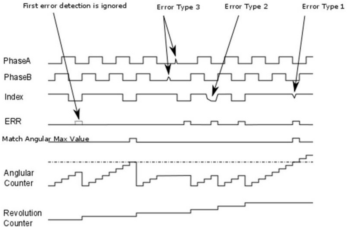
Figure 42-7. Secure Decoder Detections
