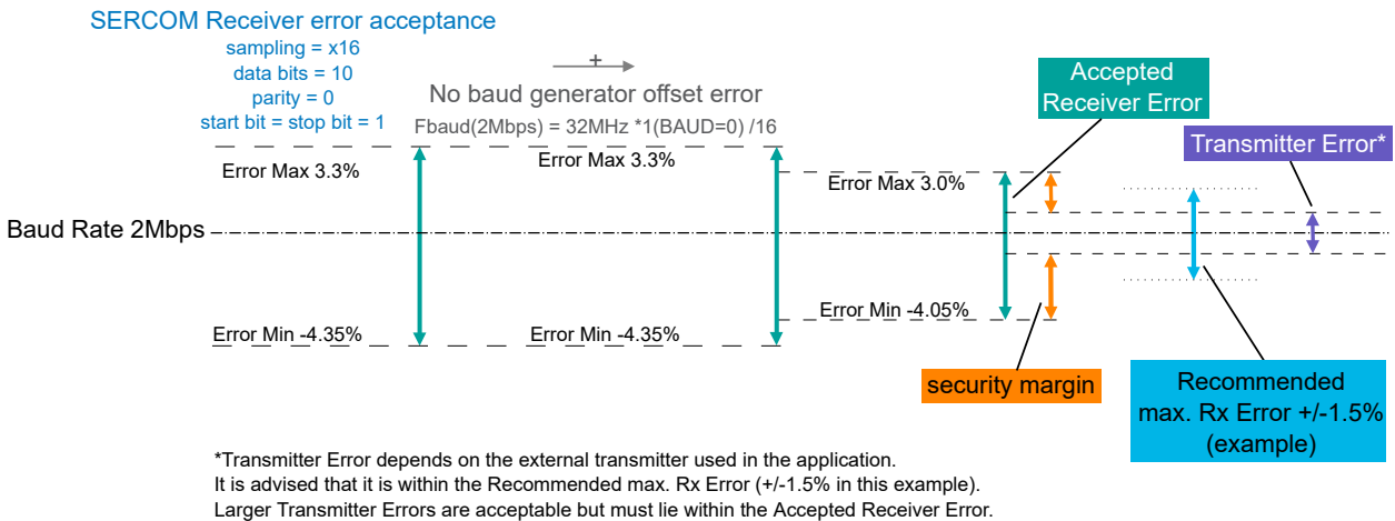
Figure 32-8. USART Rx Error Calculation Example
