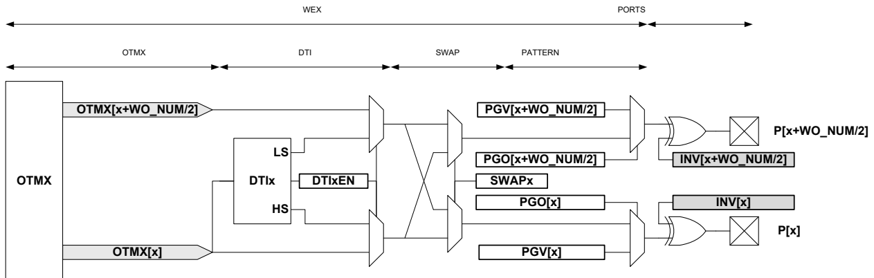
Figure 45-34. Waveform Extension Stage Details
