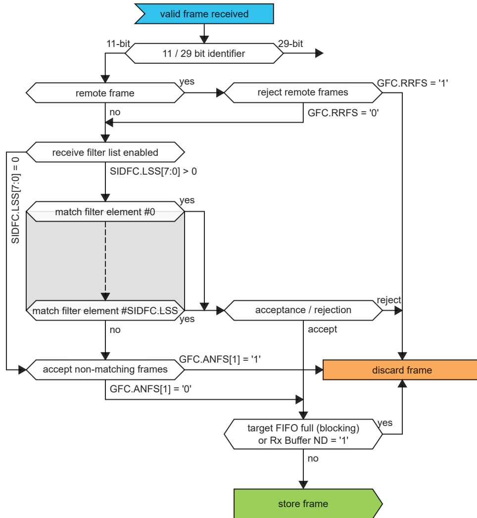
Figure 38-5. Standard Message ID Filtering
