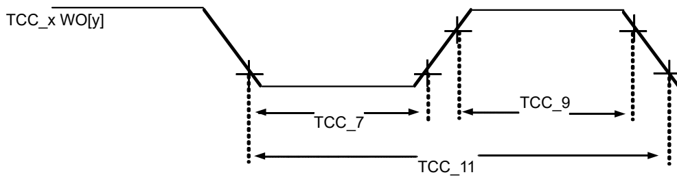
Figure 55-20. TCC Timer Compare Fault Output Module Timing Diagrams
