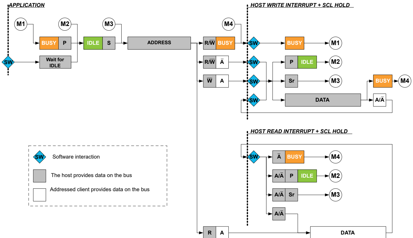
Figure 34-5. I 2 C Host Behavioral Diagram
