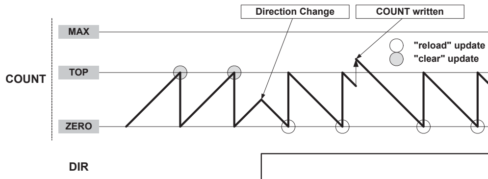
Figure 45-3. Counter Operation
