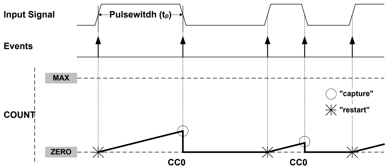
Figure 44-14. Pulse-Width Capture on Channel 0
