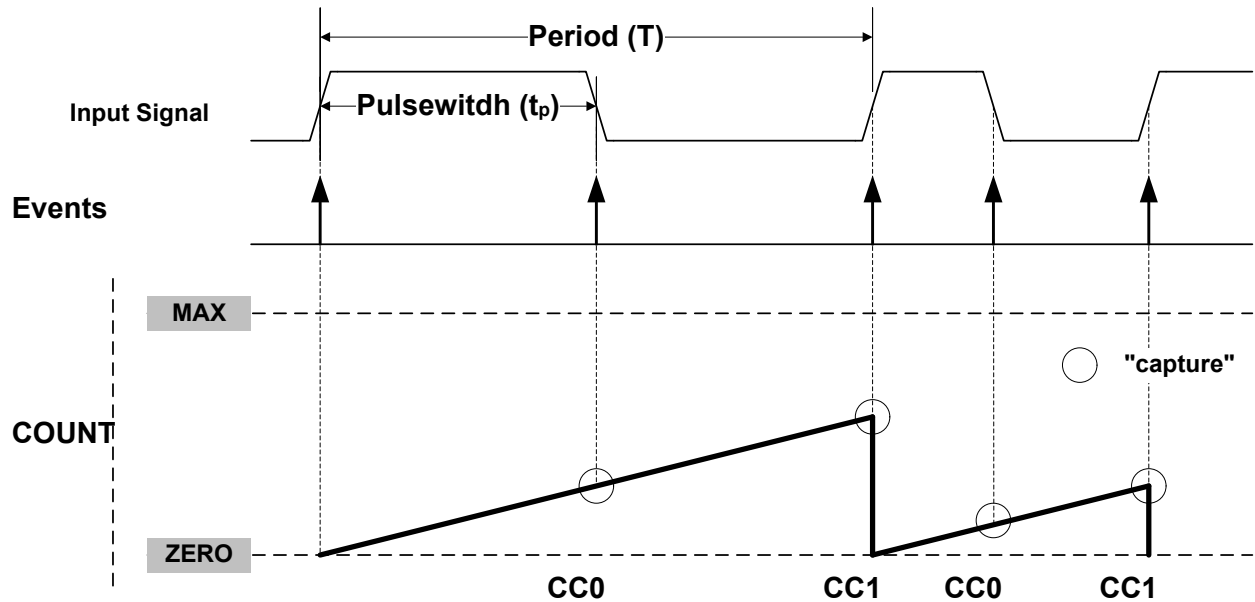
Figure 44-13. PWP Capture
