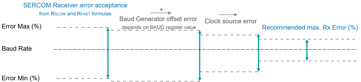
Figure 32-7. USART Rx Error Calculation
