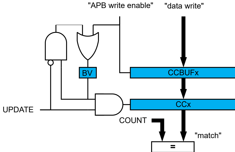
Figure 45-9. Compare Channel Double Buffering
