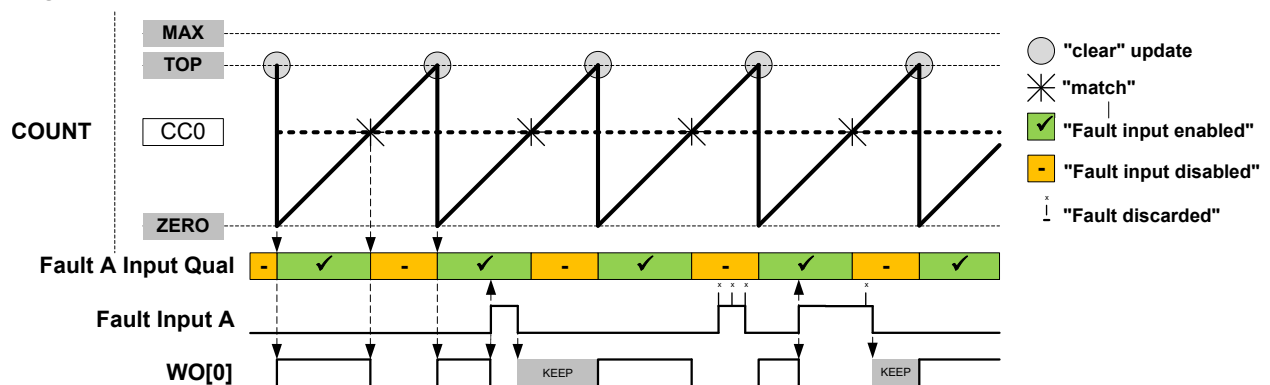
Figure 45-25. Waveform Generation with Fault Qualification and Keep Action
