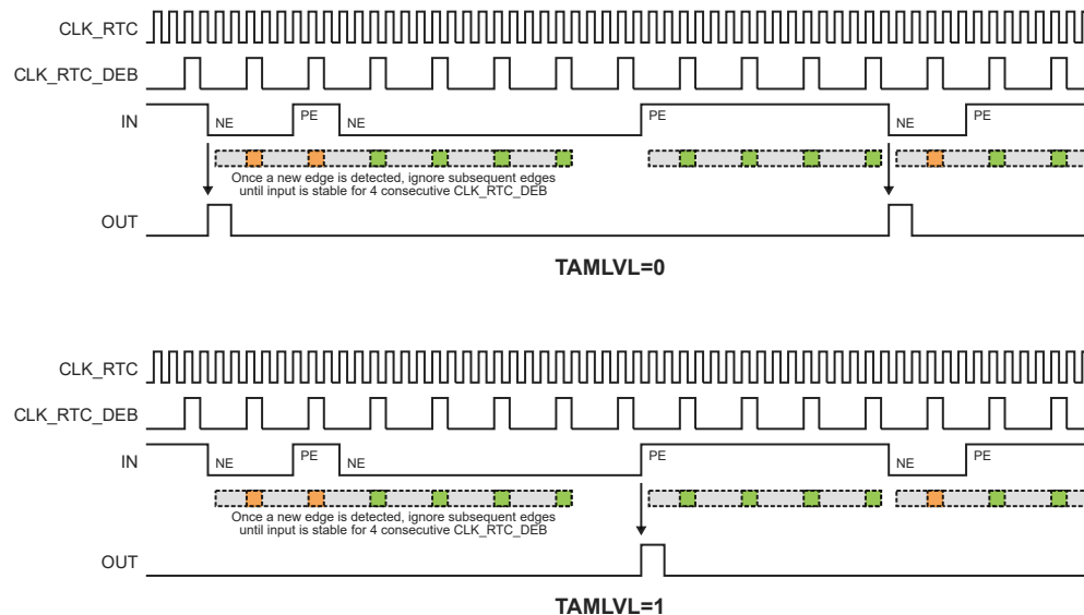
Figure 23-7. Edge Detection with Asynchronous Stability Debouncing
