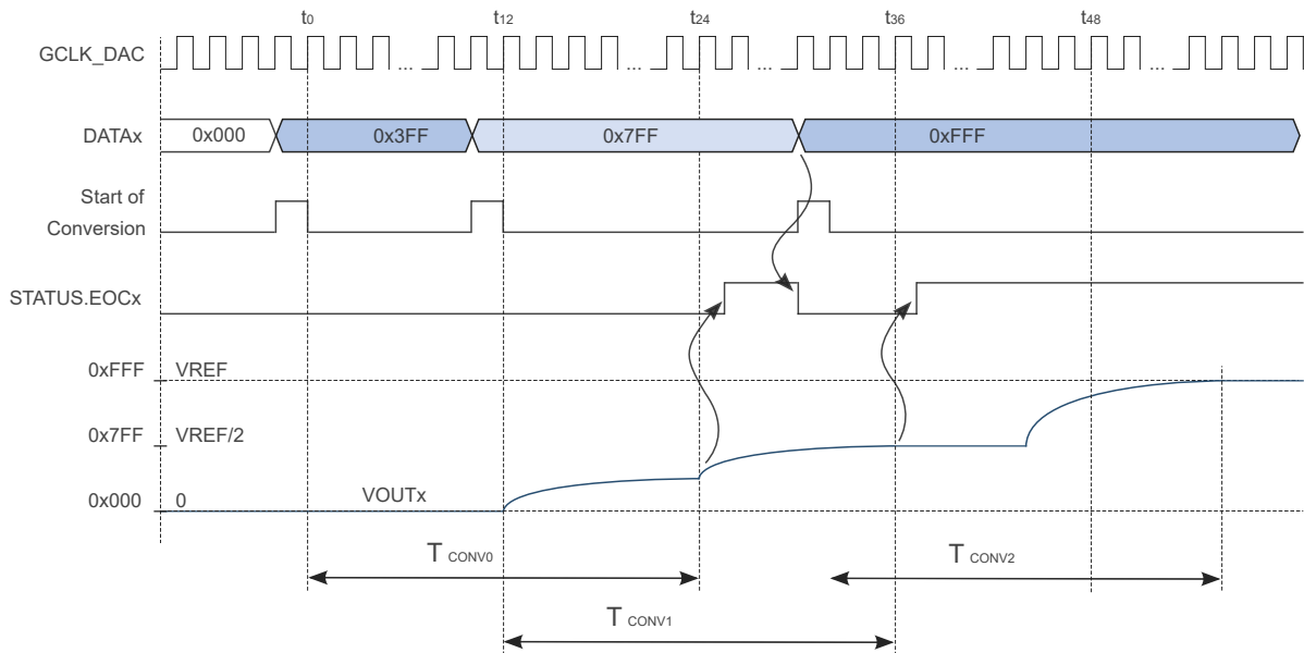
Figure 53-3. Multiple DAC Conversions
