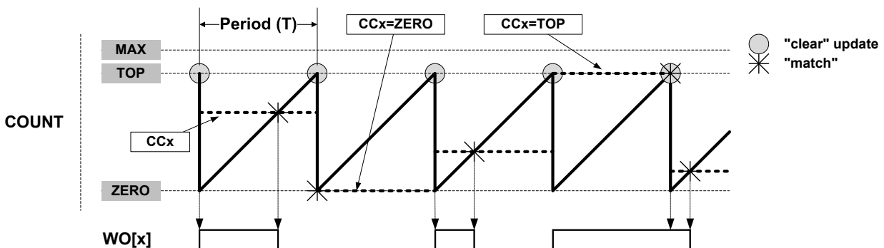
Figure 45-6. Single-Slope PWM Operation
