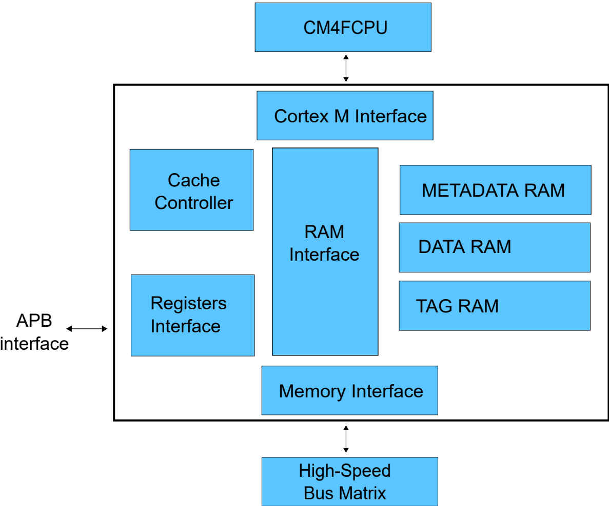
Figure 11-2. CMCC Organization
