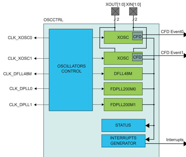
Figure 18-1. OSCCTRL Block Diagram
