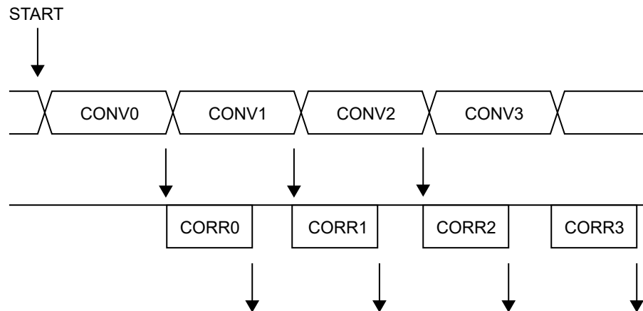
Figure 51-7. ADC Timing Correction Enabled
