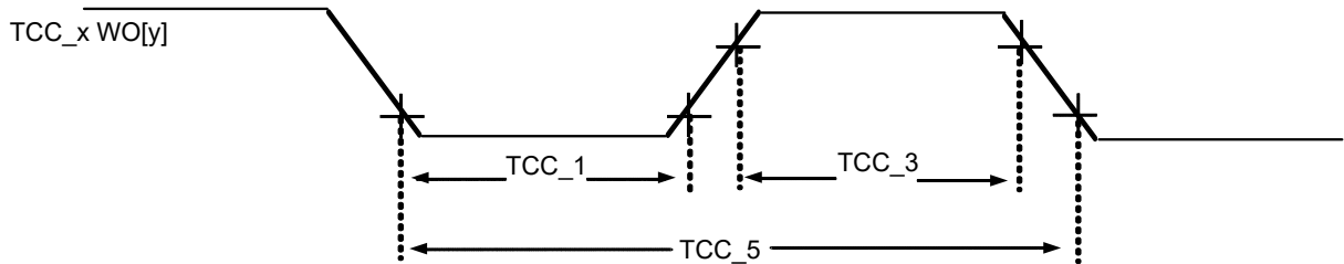
Figure 55-19. TCC Timer Compare Output Module Timing Diagrams
