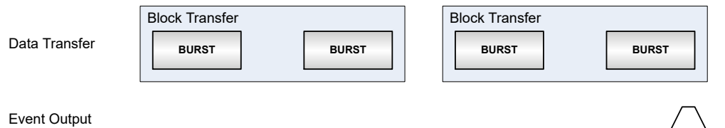
Figure 25-16. Block Event Output Generation
