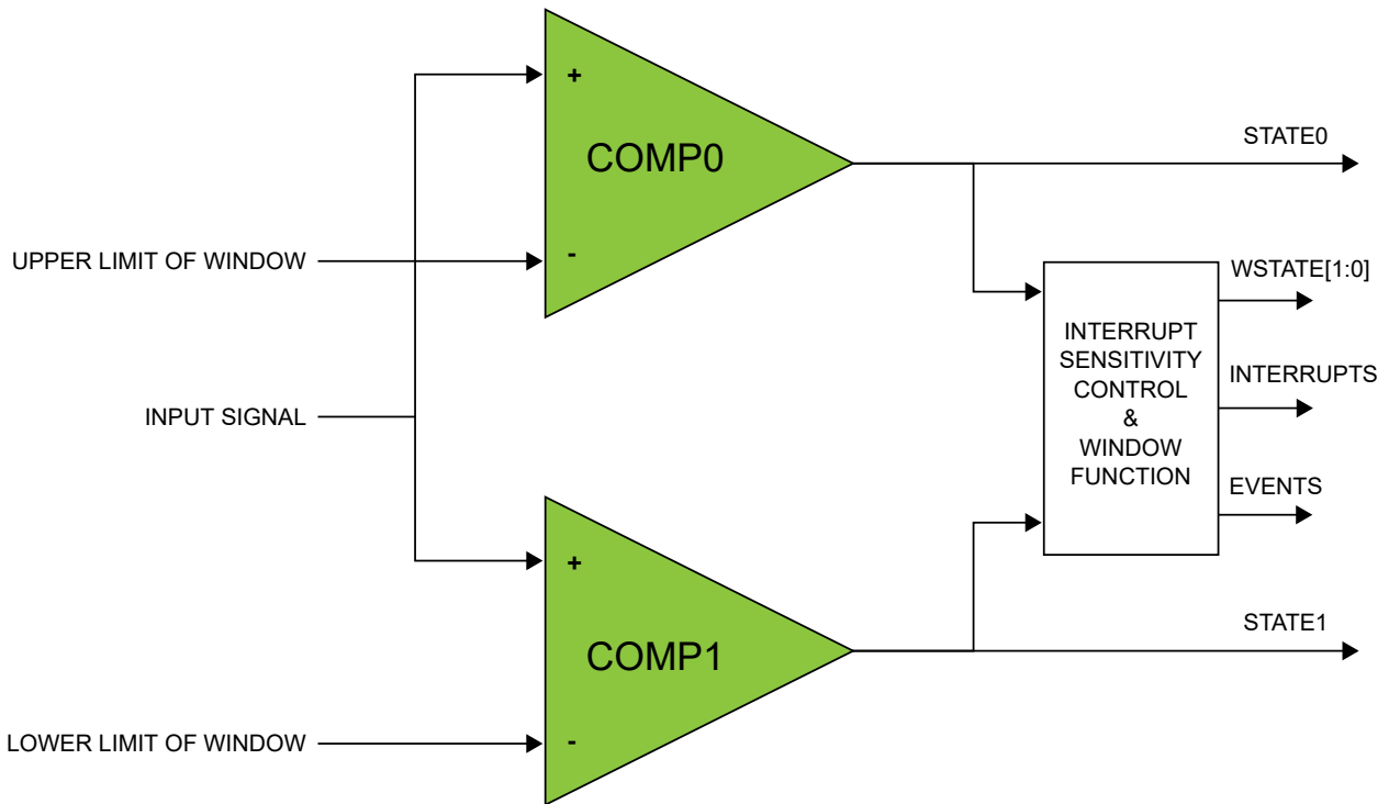
Figure 52-4. Comparators in Window Mode
