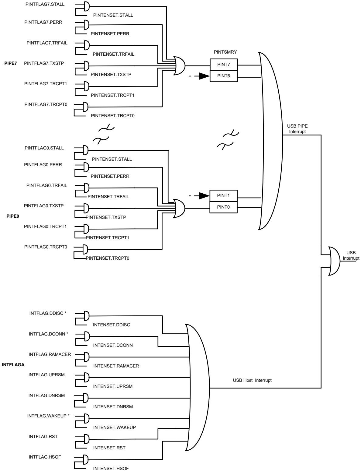
Figure 40-10. Host Interrupt
