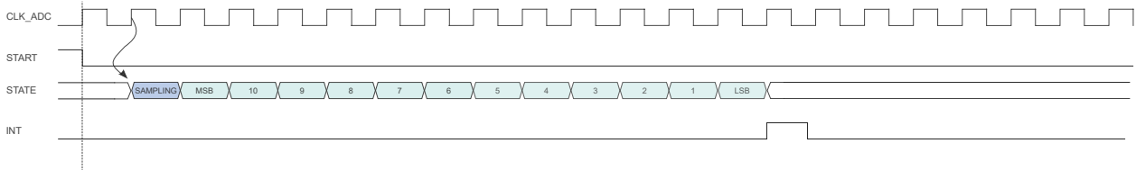
Figure 51-3. ADC Timing for One Conversion in 12-bit Resolution
