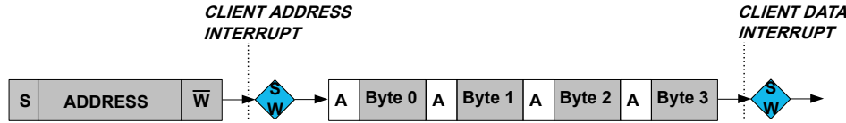
Figure 34-15. 32-bit Extension Client Operation
