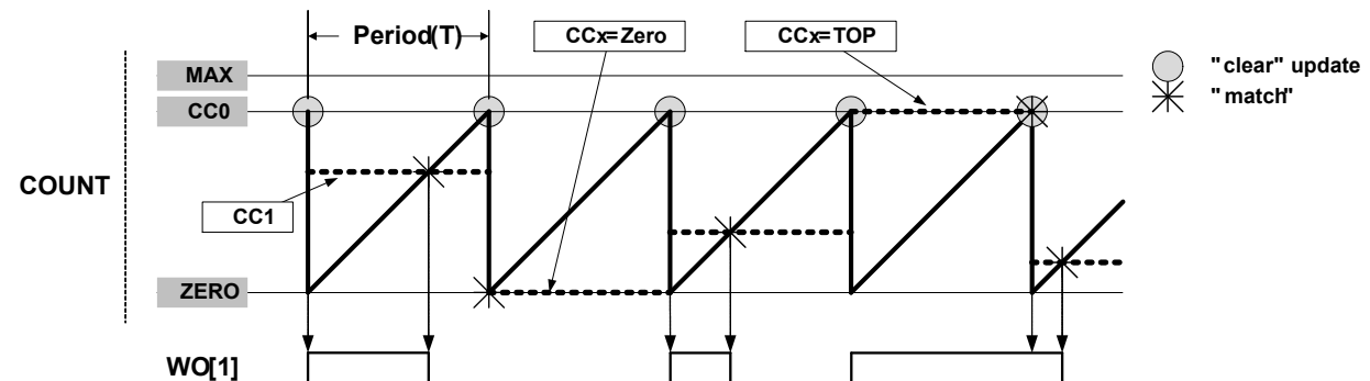
Figure 44-6. Match PWM Operation
