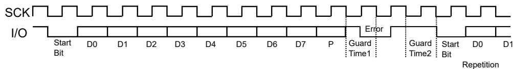
Figure 32-21. T=0 Protocol with Parity Error
