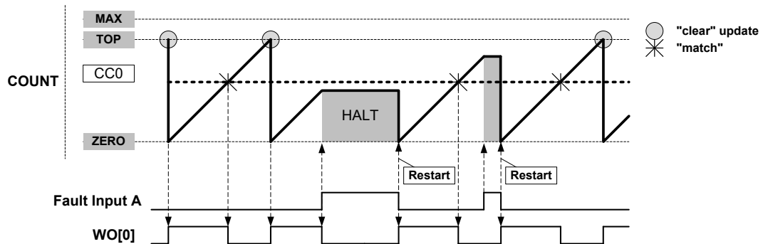
Figure 45-30. Waveform Generation with Halt and Restart Actions
