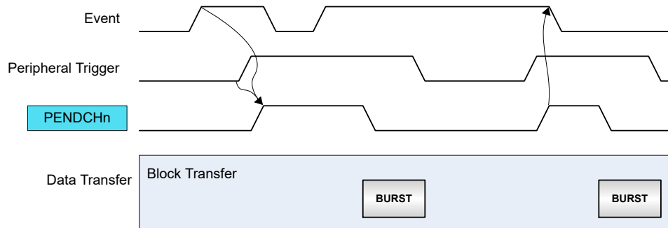
Figure 25-14. Conditional Event with Burst Peripheral Triggers
