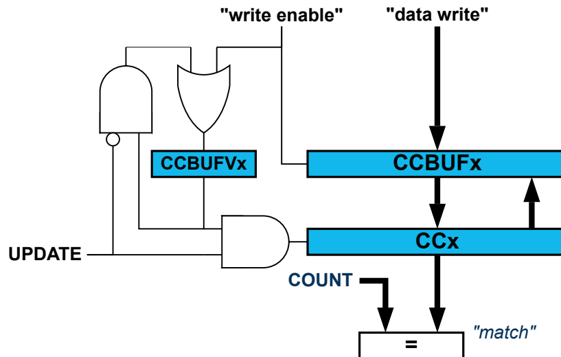
Figure 44-7. Compare Channel Double Buffering
