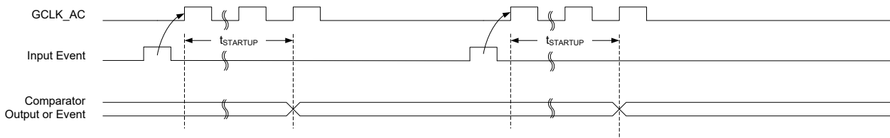
Figure 52-10. Single-Shot SleepWalking
