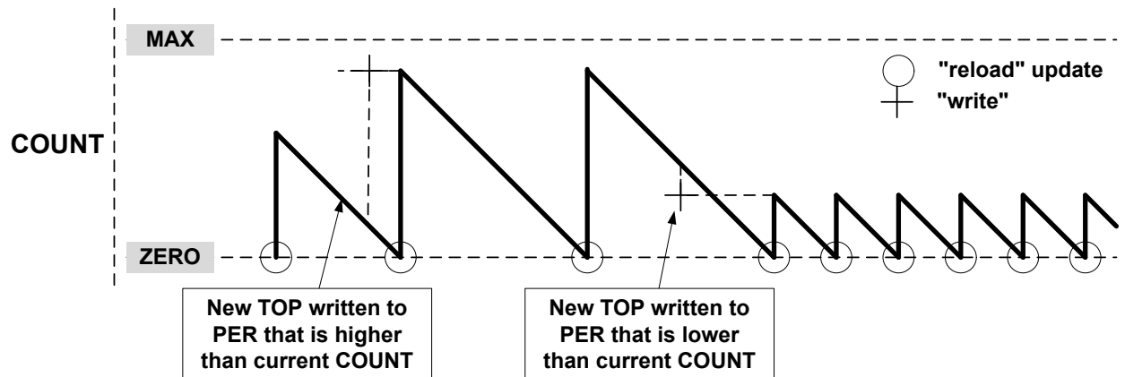
Figure 44-9. Unbuffered Single-Slope Down-Counting Operation
