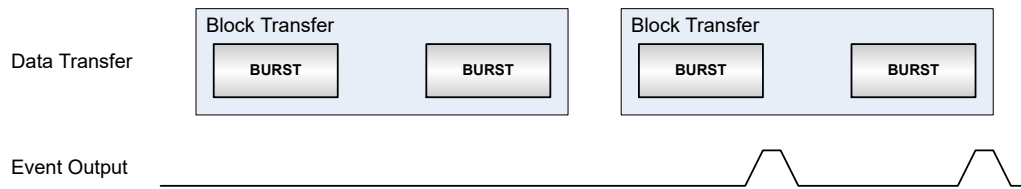
Figure 25-17. Burst Event Output Generation
