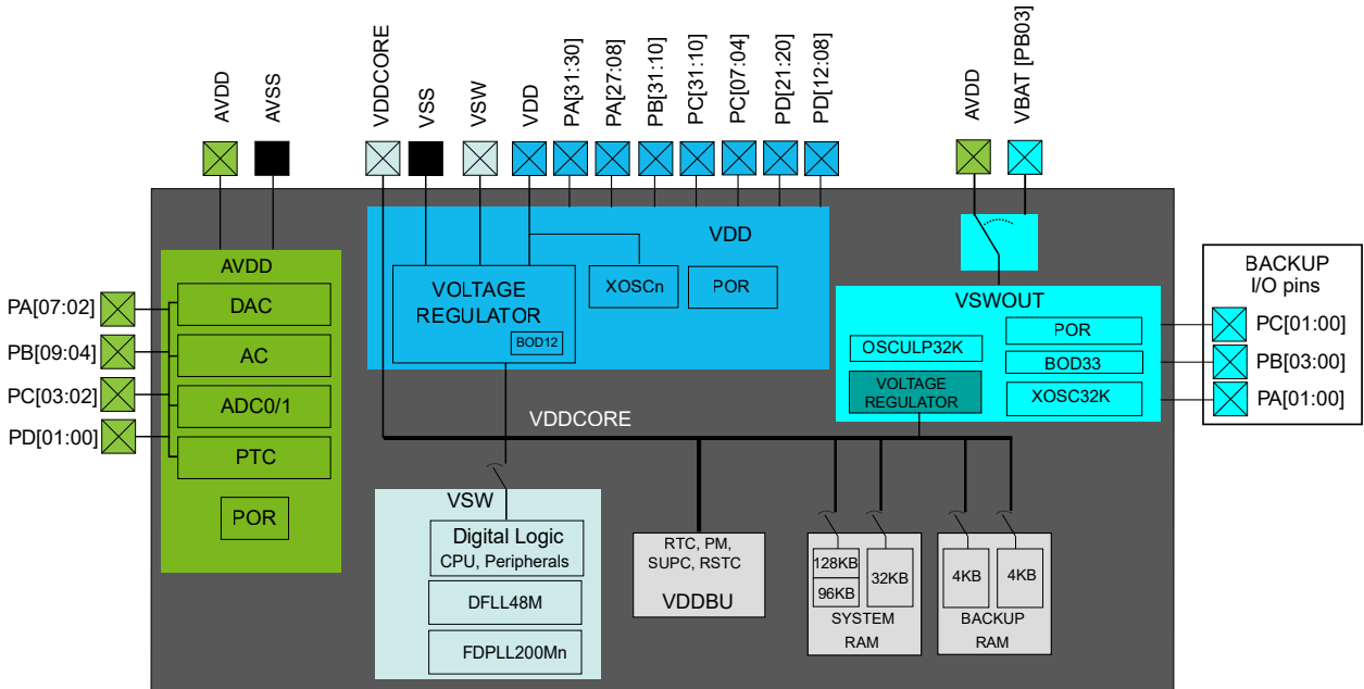
Figure 6-1. Power Supplies Block Diagram
