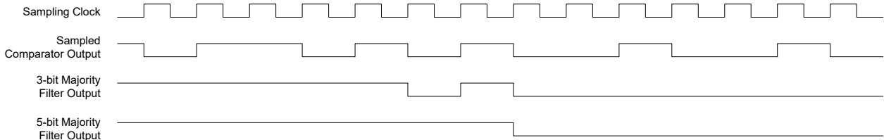
Figure 52-6. Continuous Mode Filtering
