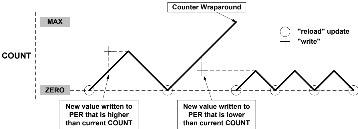
Figure 45-12. Unbuffered Dual-Slope Operation
