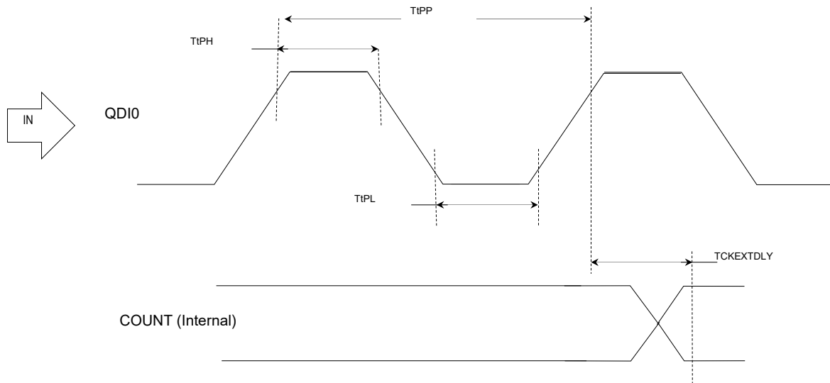
Figure 56-18. Position Decoder (PDEC) Input Timing Diagrams
