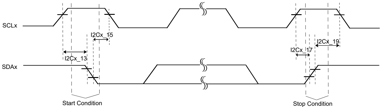
Figure 55-9. I 2 C Bus Data Host Mode Timing Diagrams
