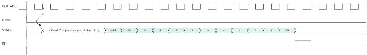
Figure 51-5. ADC Timing for One Conversion with Offset Compensation, 12-bit
