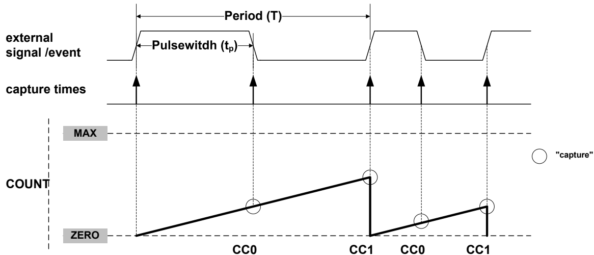
Figure 45-16. PWP Capture
