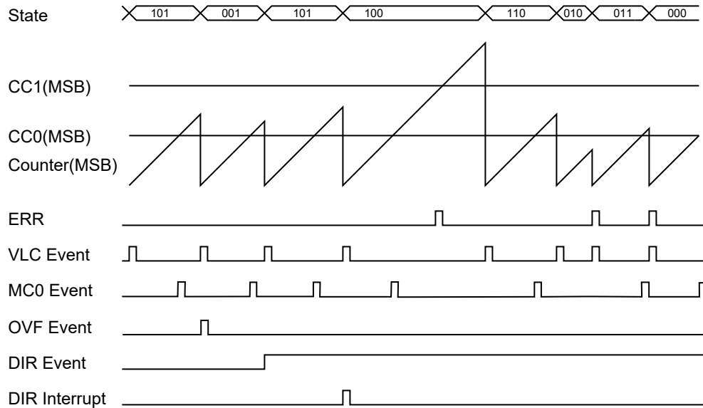
Figure 42-12. Hall Waveforms
