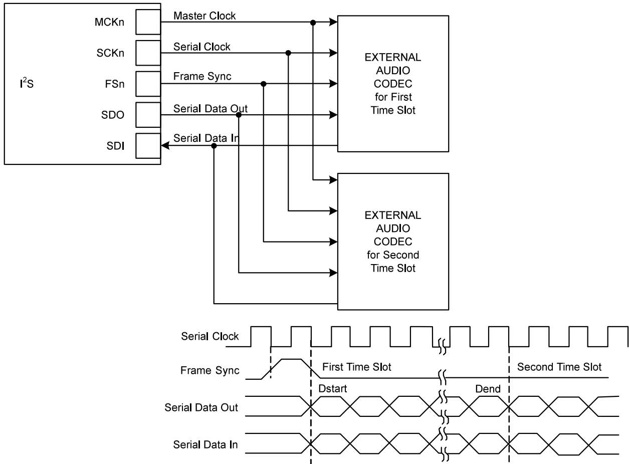
Figure 37-9. Codec Application Block Diagram
