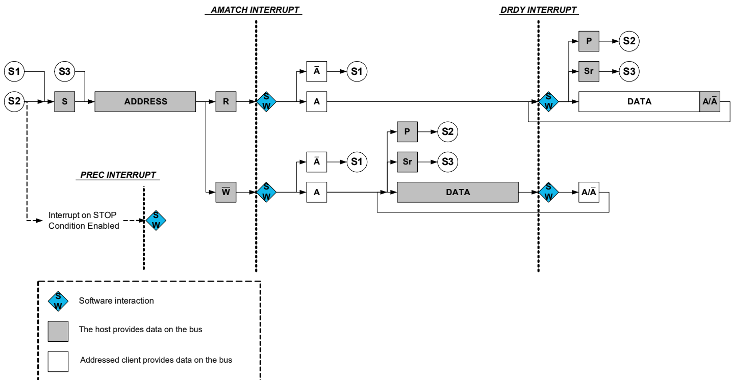
Figure 34-10. I 2 C Client Behavioral Diagram
