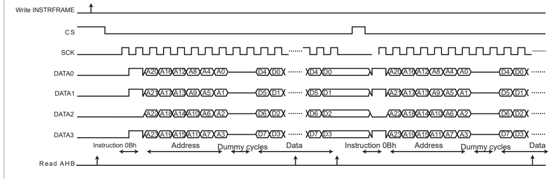
Figure 35-19. Instruction Transmission Waveform 8
