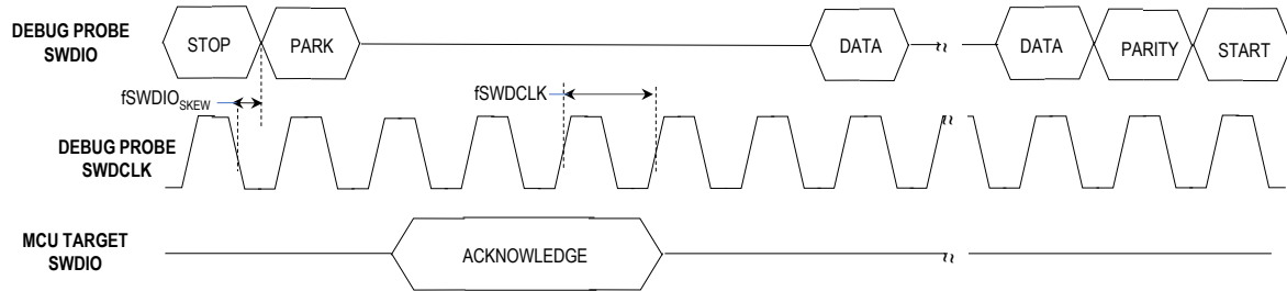
Figure 55-29. SWD 2-Wire Read/Write Timing Diagrams
