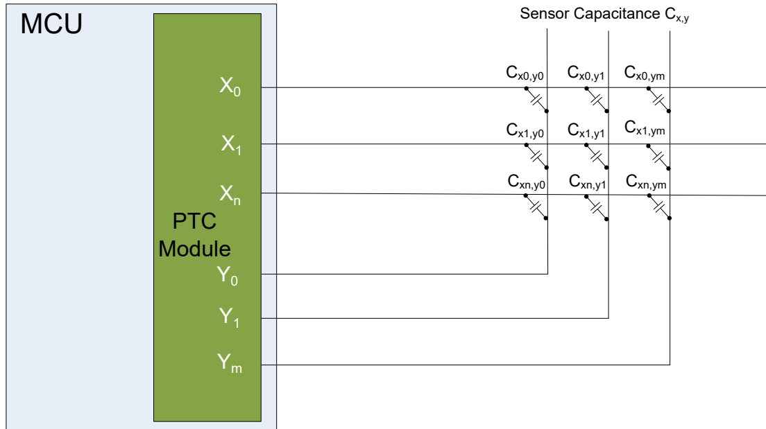
Figure 54-3. Mutual Capacitance Sensor Arrangement
