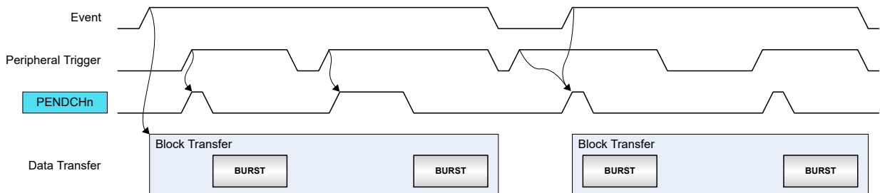
Figure 25-15. Conditional Block Transfer with Burst Peripheral Triggers
