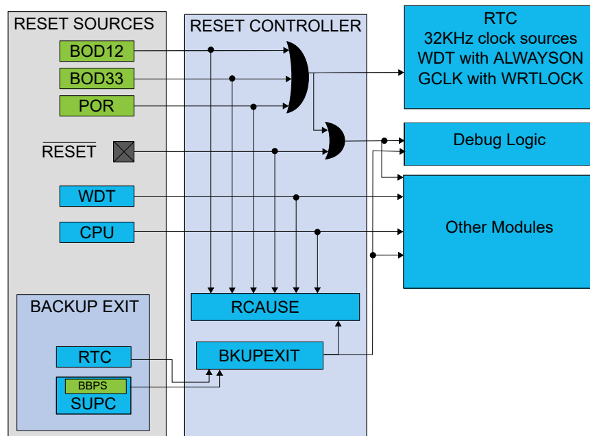
Figure 21-1. Reset System
