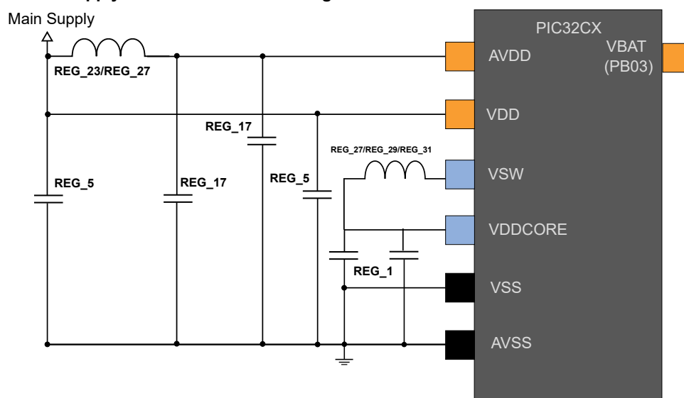
Figure 58-1. Power Supply Connection for Switching/Linear Mode
