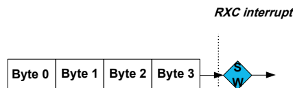
Figure 32-25. 32-bit Extension Receive Operation
