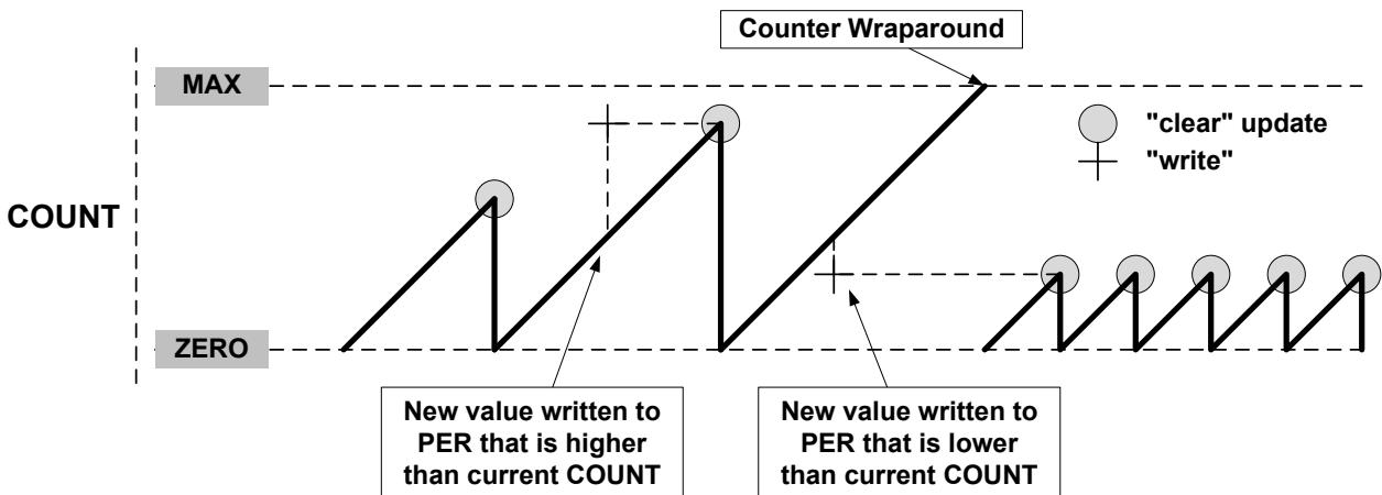
Figure 45-10. Unbuffered Single-Slope Up-Counting Operation
