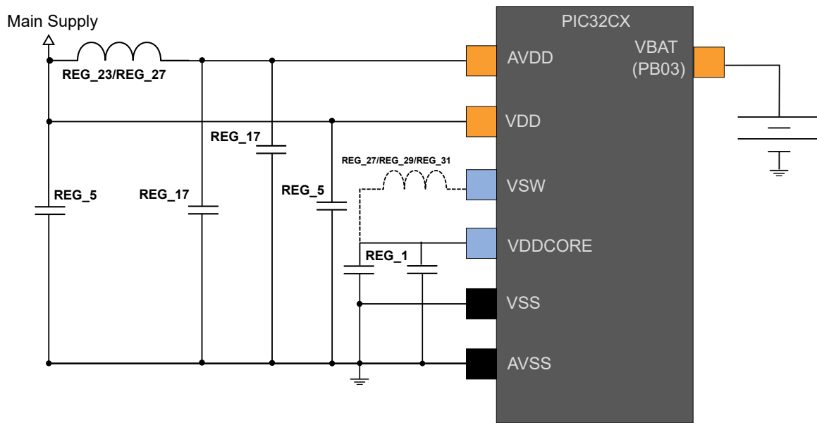
Figure 58-3. Power Supply Connection for Battery Backup Mode
