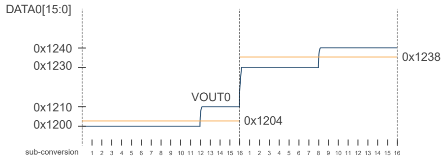
Figure 53-5. DAC Conversions in Dithering Mode
