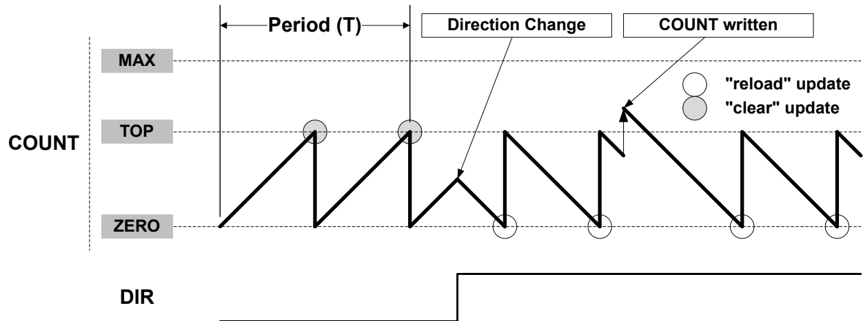
Figure 44-3. Counter Operation
