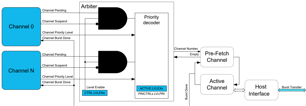
Figure 25-4. Arbiter Overview
