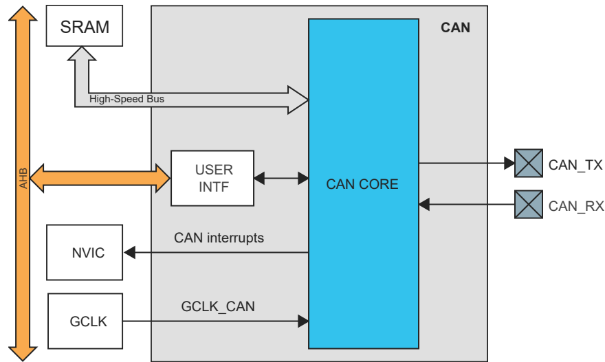
Figure 38-1. CAN Block Diagram
