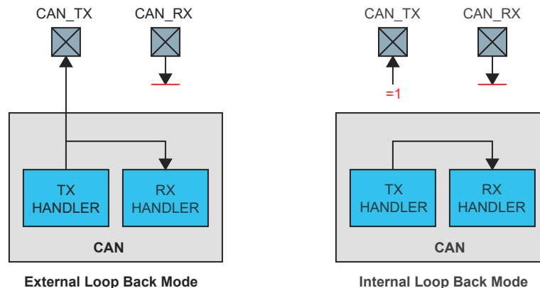
Figure 38-4. Pin Control in Loop Back Modes
