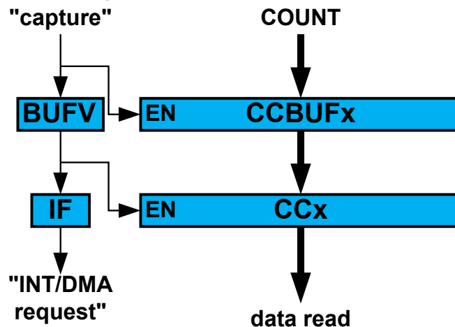
Figure 45-15. Capture Double Buffering
