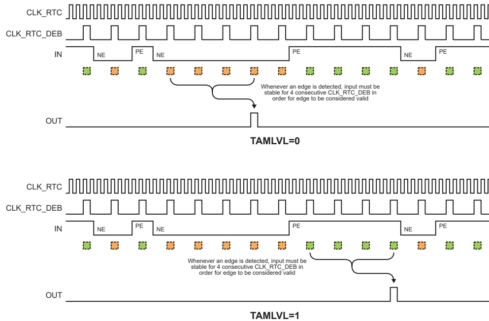
Figure 23-7. Edge Detection with Asynchronous Stability Debouncing
