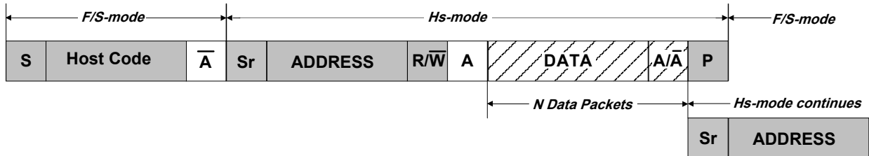
Figure 34-8. High Speed Transfer
