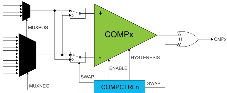
Figure 52-8. Input Swapping for Offset Compensation
