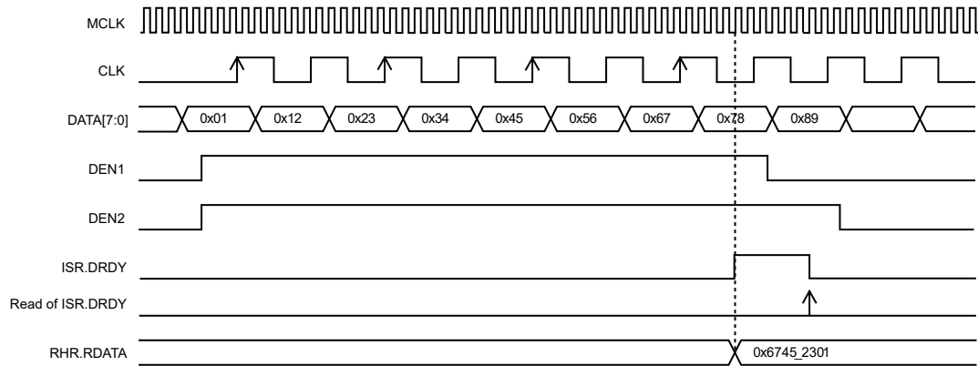
Figure 39-10. PCC Waveforms (ISIZE = 10_BITS, DSIZE = 2_DATA, ALWAYS = 0, HALFS = 1, FRSTS = 0, SCALE = 0)
