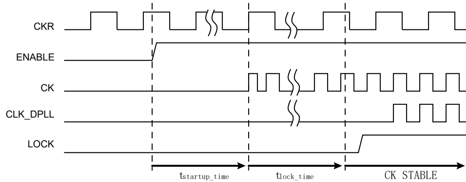
Figure 18-5. CK and CLK_DPLL Output from DPLL Off Mode to Running Mode When Wake Up Fast is Activated
