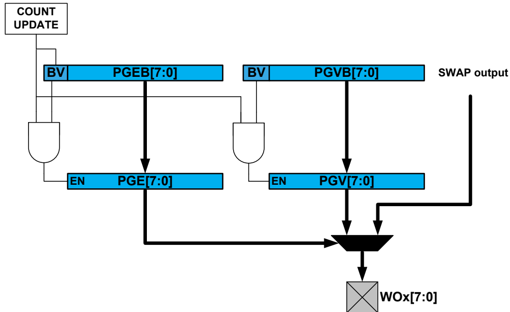
Figure 45-37. Pattern Generator Block Diagram
