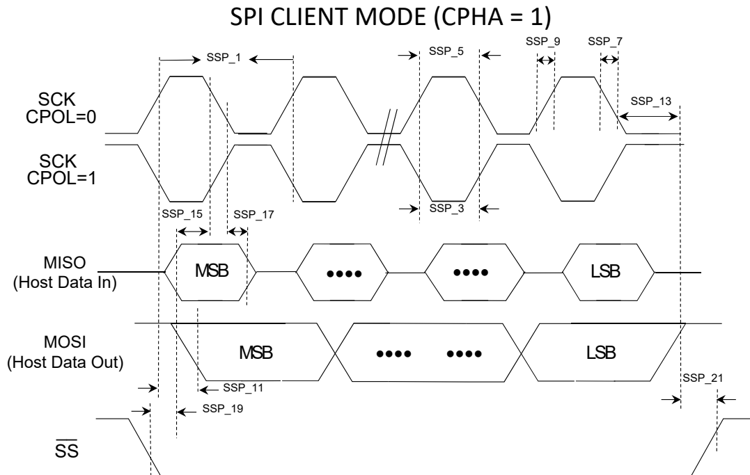
Figure 56-4. SPI Client Module (CPHA=1) Timing Diagrams
