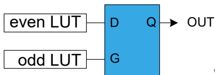
Figure 43-15. D-Latch
