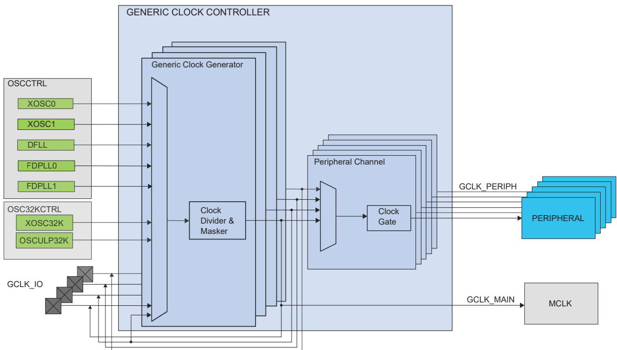
Figure 15-1. Device Clocking Diagram
