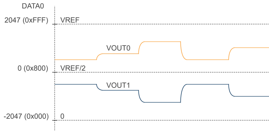
Figure 53-4. DAC Conversions in Differential Mode
