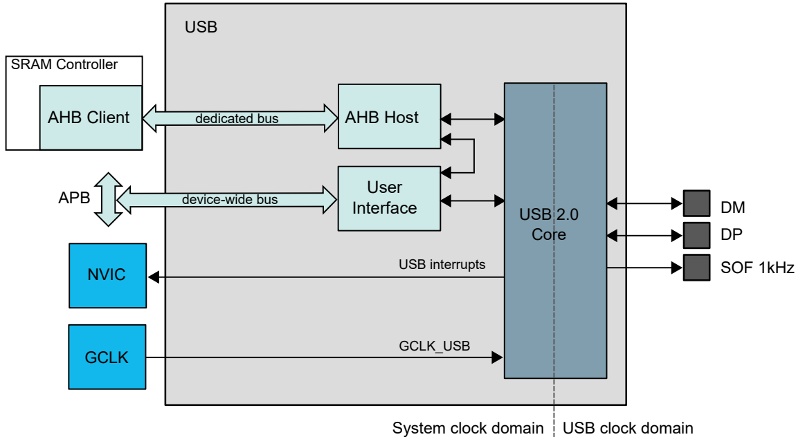
Figure 40-1. LS/FS Implementation: USB Block Diagram
