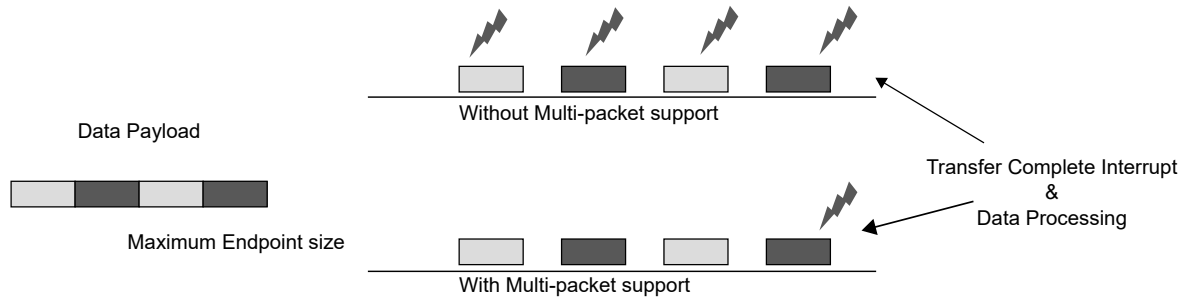
Figure 40-3. Multi-Packet Feature - Reduction of CPU Overhead
