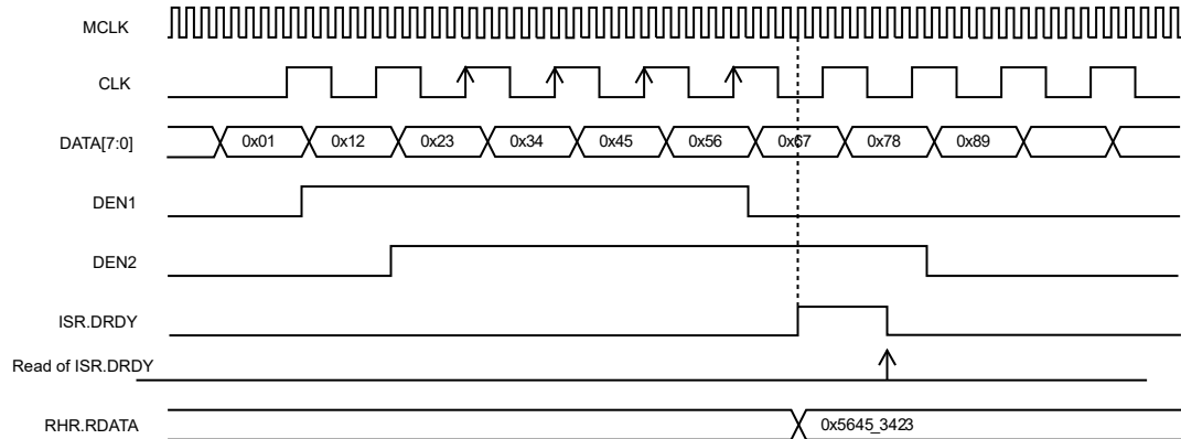
Figure 39-4. PCC Waveforms (ISIZE = 10_BITS, DSIZE = 2_DATA, ALWAYS = 0, HALFS = 0, SCALE = 0)
