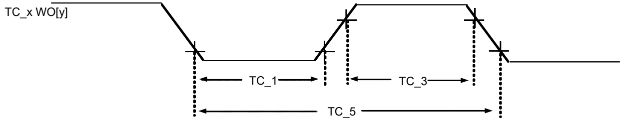
Figure 56-12. TC Timer Compare Output Module Timing Diagrams
