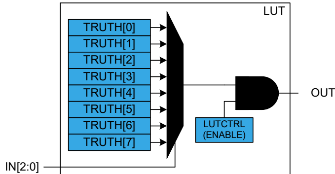
Figure 43-2. Truth Table Output Value Selection
