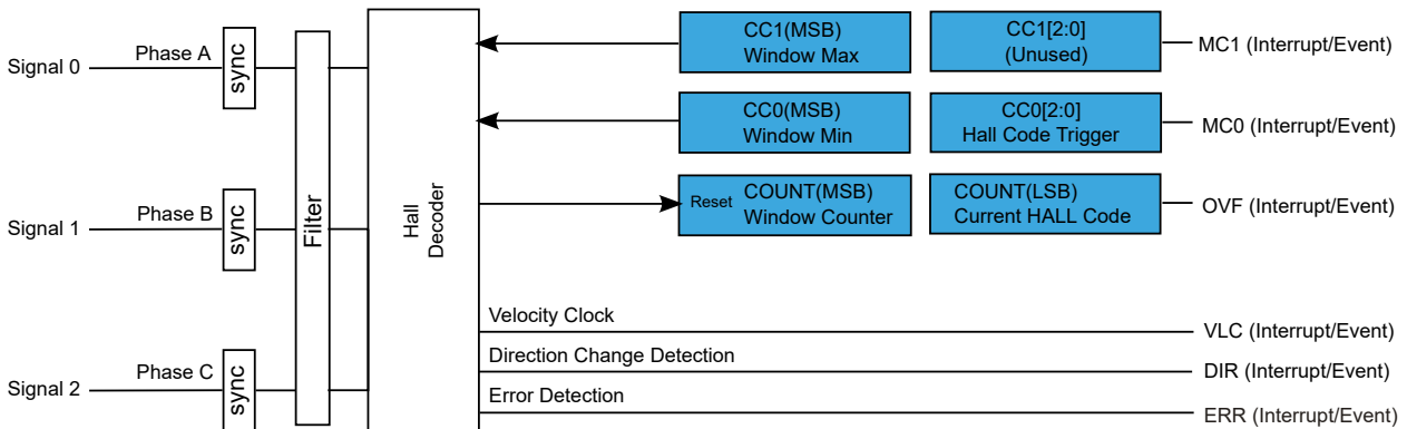
Figure 42-10. HALL Block Diagram
