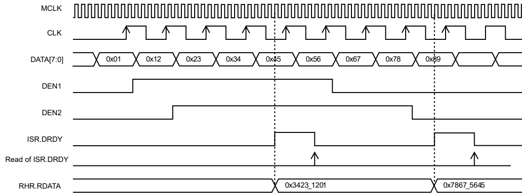
Figure 39-7. PCC Waveforms (ISIZE = 10_BITS, DSIZE = 2_DATA, ALWAYS = 1, HALFS = 0, SCALE = 0)
