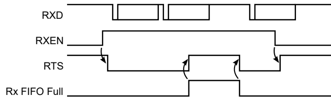
Figure 32-10. Receiver Behavior when Operating with Hardware Handshaking
