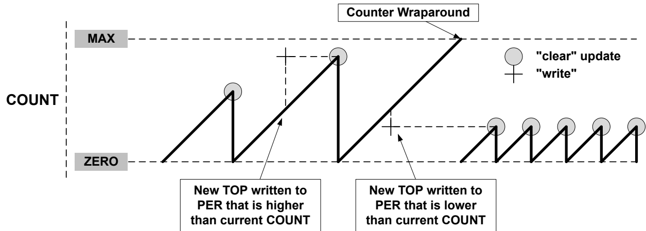
Figure 44-8. Unbuffered Single-Slope Up-Counting Operation
