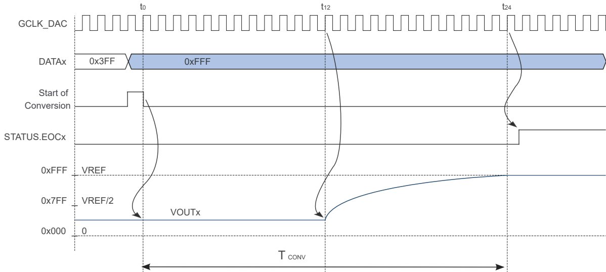
Figure 53-2. Single DAC Conversion
