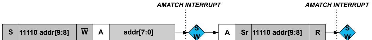
Figure 34-11. 10-bit Addressing
