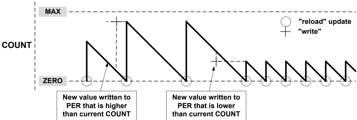
Figure 45-11. Unbuffered Single-Slope Down-Counting Operation
