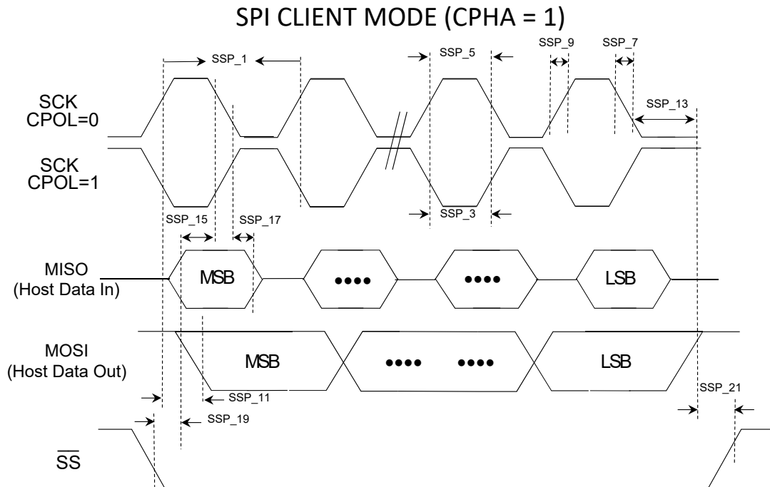
Figure 55-4. SPI Client Module (CPHA = 1) Timing Diagrams
