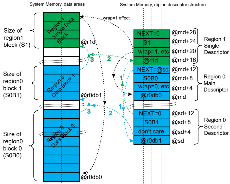
Figure 49-4. Example - Monitoring of 3 Memory Data Blocks (Defined as 2 Regions)
