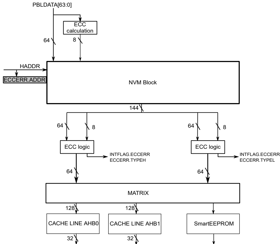
Figure 27-2. ECC Diagram
