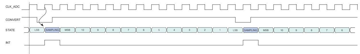
Figure 51-6. ADC Timing for Free Running in 12-bit Resolution
