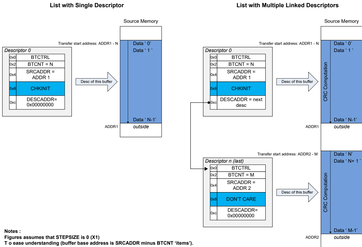
Figure 25-20. CRC Computation with Single Linked Transfers
