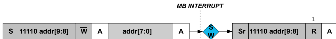
Figure 34-9. 10-bit Address Transmission for a Read Transaction
