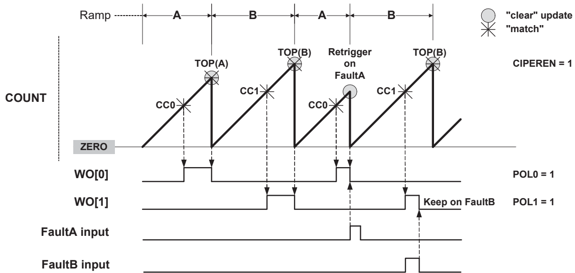
Figure 45-18. RAMP2 Standard Operation
