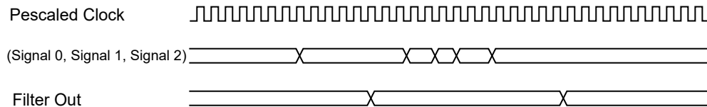
Figure 42-3. Input Signal Filtering
