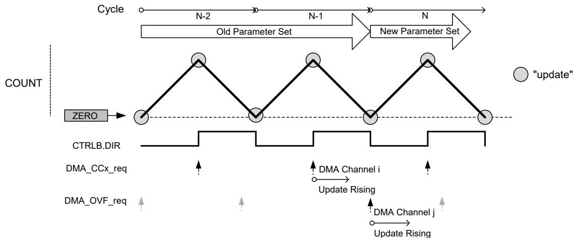
Figure 45-39. DMA Triggers in DSBOTH Operation Mode and Circular Buffer Enabled
