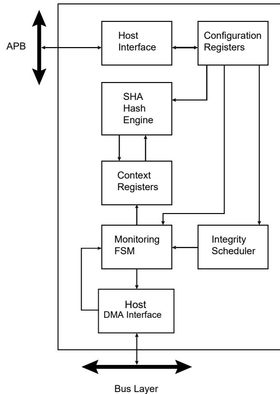
Figure 49-1. Integrity Check Monitor Block Diagram
