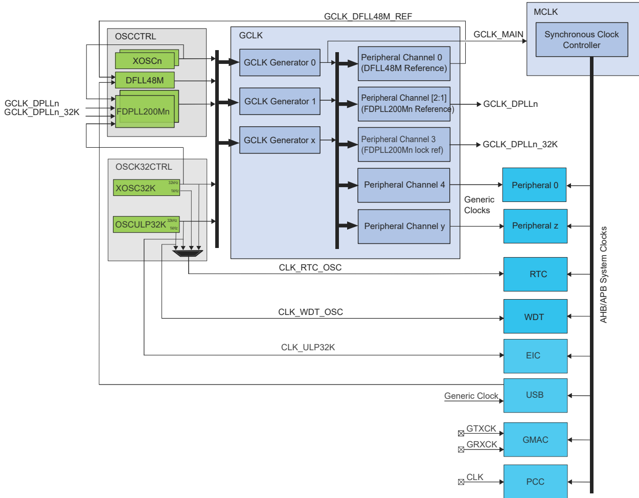
Figure 14-1. Clock Distribution
