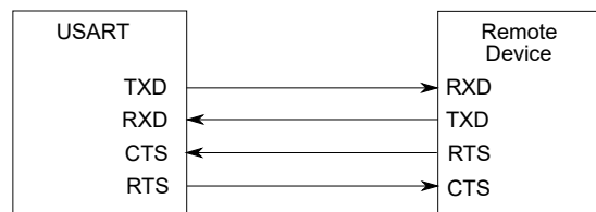
Figure 32-9. Connection with a Remote Device for Hardware Handshaking
