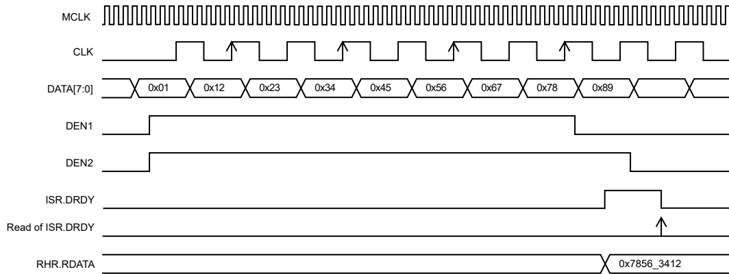
Figure 39-13. PCC Waveforms (ISIZE = 10_BITS, DSIZE = 2_DATA, ALWAYS = 0, HALFS = 1, FRSTS = 1, SCALE = 0)
