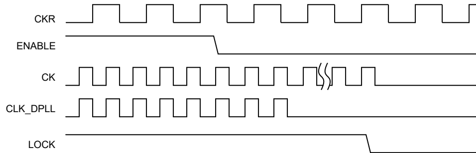
Figure 18-6. CK and CLK_DPLL Output from Running Mode to DPLLC Off Mode.
