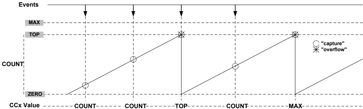
Figure 44-15. Time-Stamp
