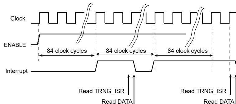
Figure 48-2. TRNG Data Generation Sequence
