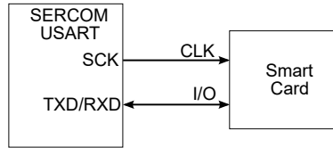
Figure 32-19. Connection of a Smart Card to the SERCOM USART
