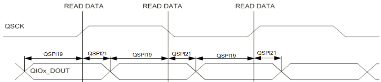
Figure 55-14. QSPI DDR Mode 0 Read Timing Diagram
