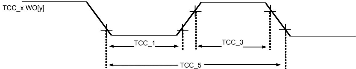
Figure 56-14. TCC Timer Compare Output Module Timing Diagrams
