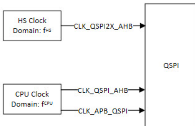
Figure 35-2. QSPI Clock Organization
