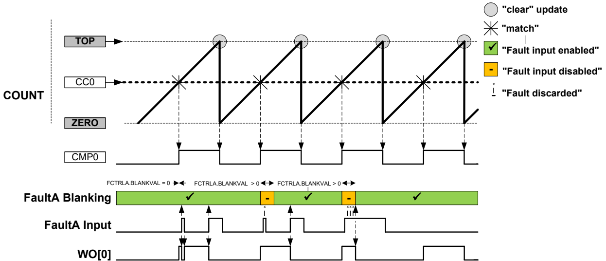
Figure 45-22. Fault Blanking in RAMP1 Operation with Inverted Polarity
