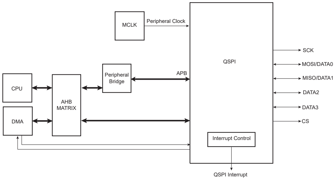
Figure 35-1. QSPI Block Diagram
