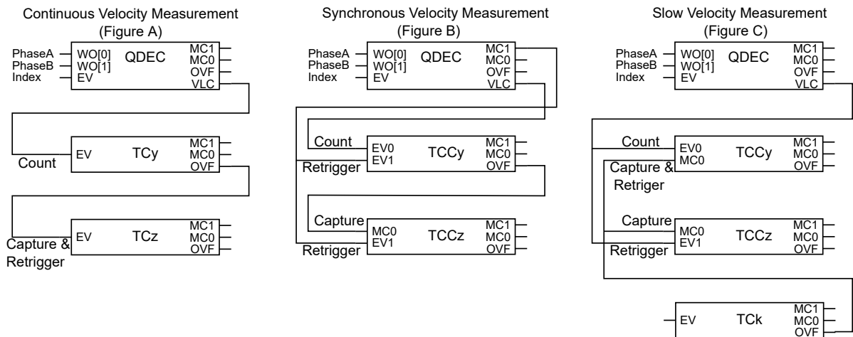
Figure 42-9. Speed Measurement
