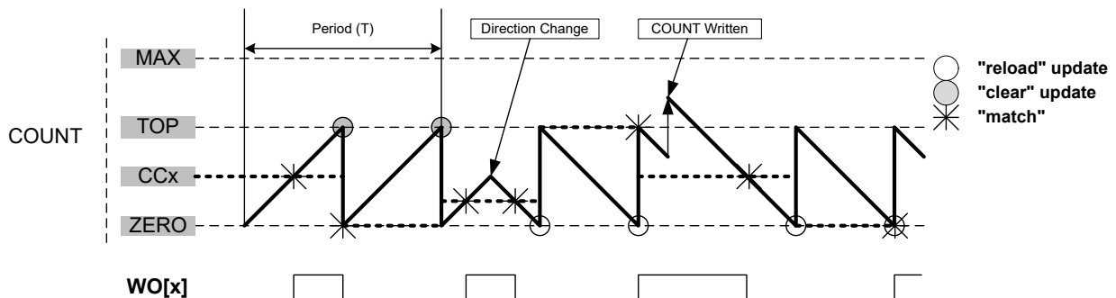
Figure 44-4. Normal Frequency Operation
