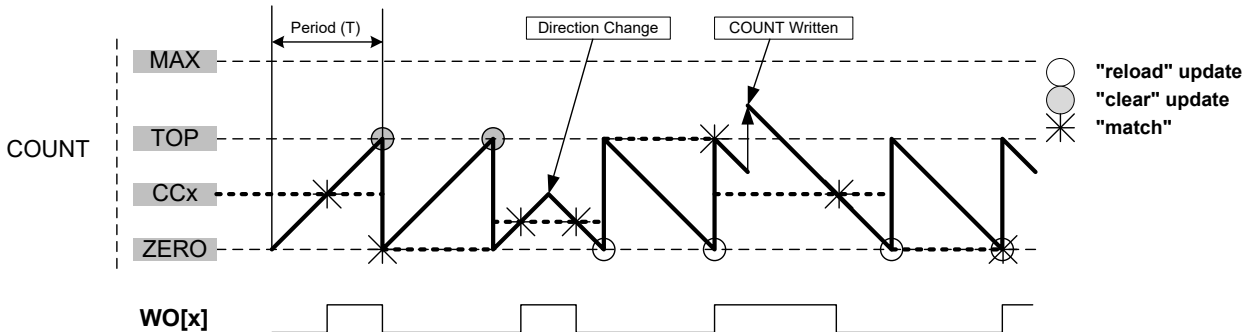
Figure 45-4. Normal Frequency Operation
