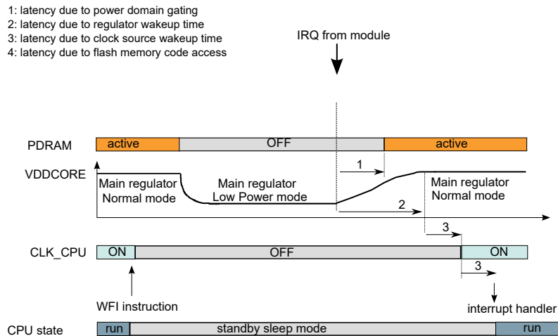
Figure 20-3. Total Wake-up Time from Standby Sleep Mode
