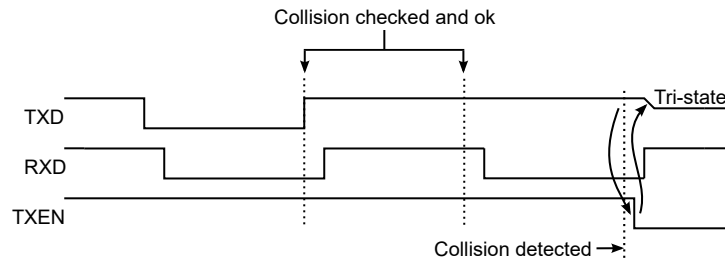
Figure 32-23. Collision Detected
