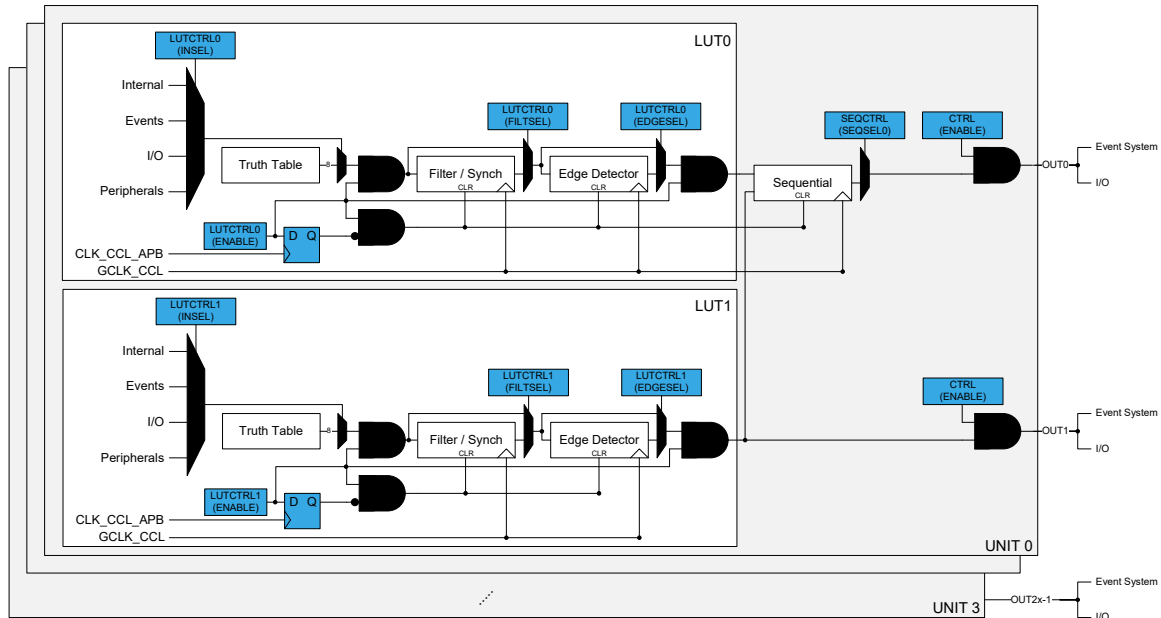
Figure 43-1. Configurable Custom Logic
