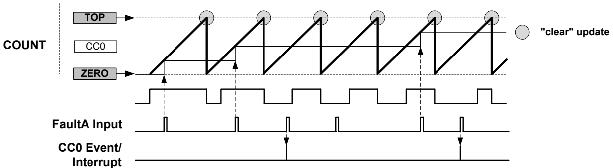
Figure 45-28. Capture Action "CAPTMAX"
