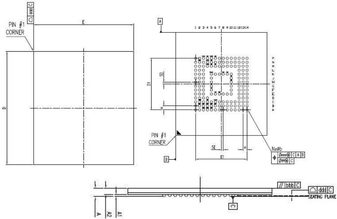
Figure 2 – Package Dimensions
