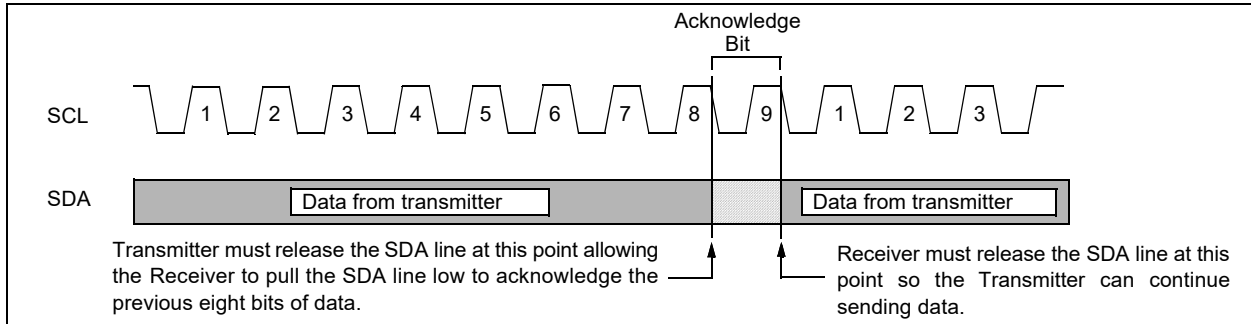
FIGURE 4-2: ACKNOWLEDGE TIMING
