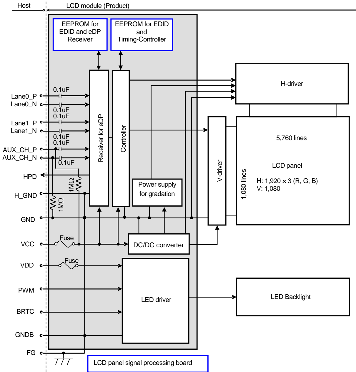
Block diagram
