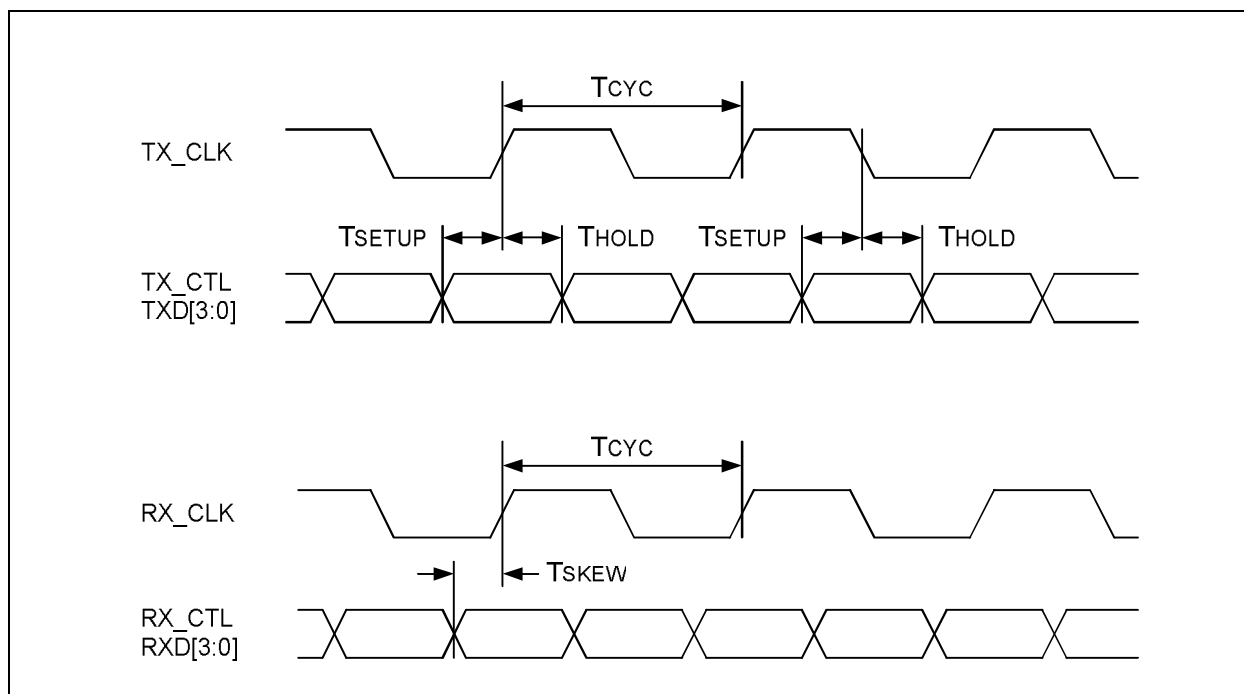
FIGURE 6-1: RGMII TIMING
