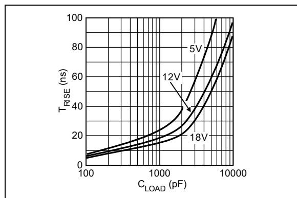
FIGURE 2-3: Rise Time vs. Capacitive Load.
