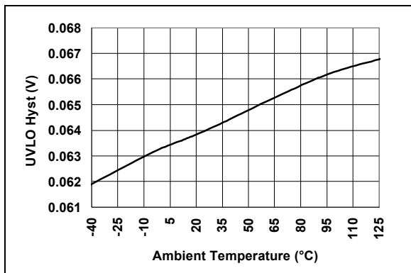
FIGURE 2-2: Undervoltage Lockout Hysteresis vs. Temperature.
