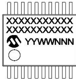
20-Lead SSOP (All Devices)
