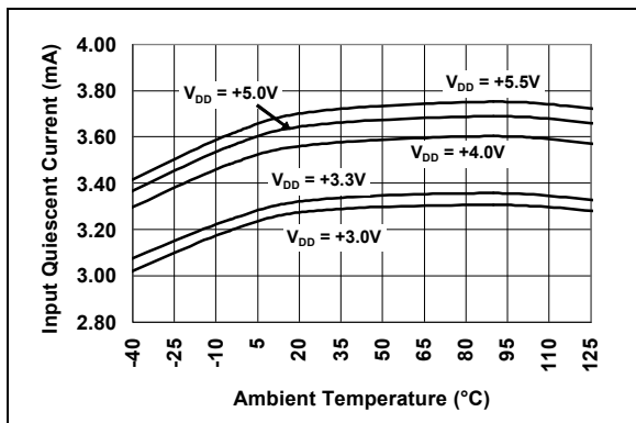
FIGURE 2-3: Input Quiescent Current vs. Temperature.
