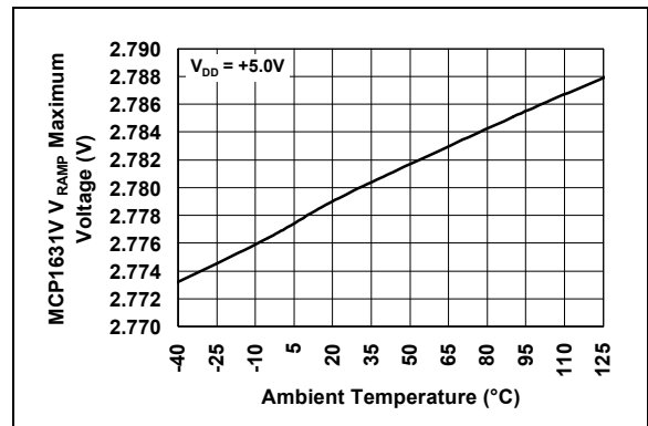
FIGURE 2-24: MCP1631V and MCP1631VHV V_{RAMP} Max Voltage (V).
