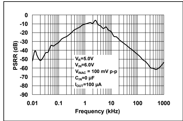
FIGURE 2-35: LDO PSRR vs. Frequency.
