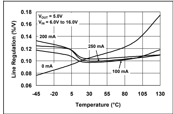
FIGURE 2-34: LDO Line Regulation vs. Temperature.
