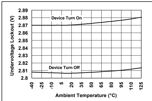
FIGURE 2-1: Undervoltage Lockout vs. Temperature.
