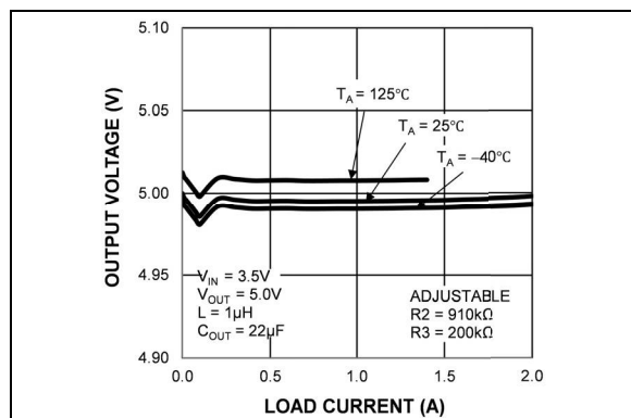
FIGURE 2-2: Output Voltage vs. Load Current.
