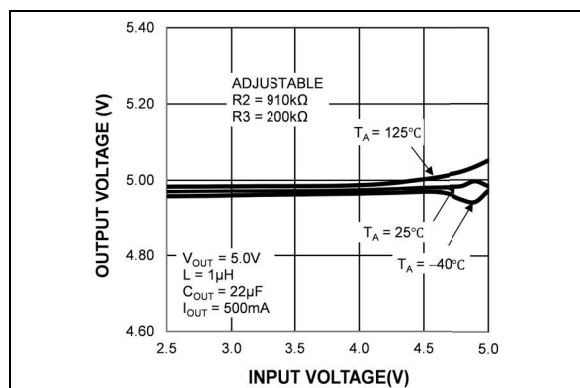
FIGURE 2-3: Output Voltage vs. Input Voltage.
