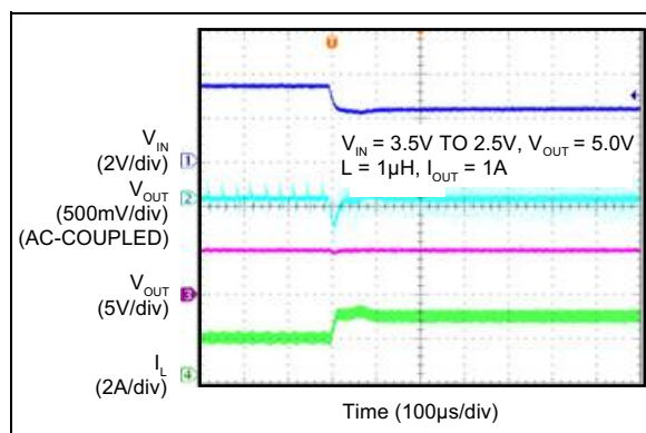
FIGURE 2-13: Line Transient (3.5V to 2.5V).
