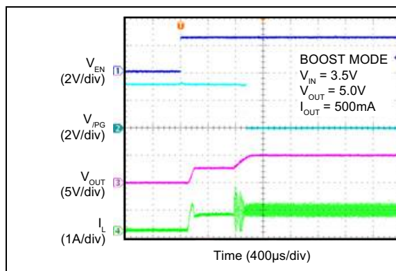
FIGURE 2-18: Soft-Start (Boost Mode).
