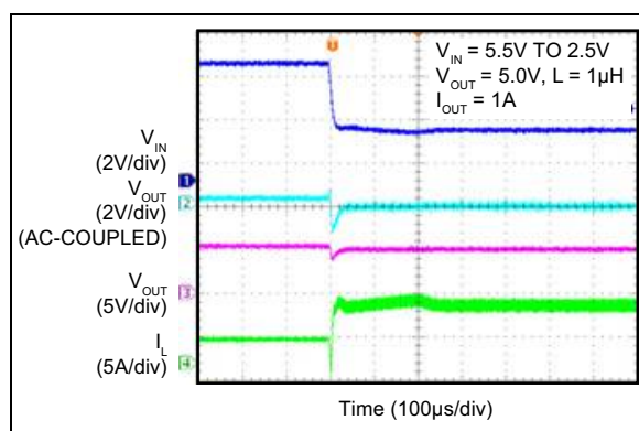
FIGURE 2-15: Line Transient (5.5V to 2.5V).
