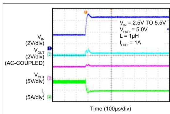
FIGURE 2-14: Line Transient (2.5V to 5.5V).
