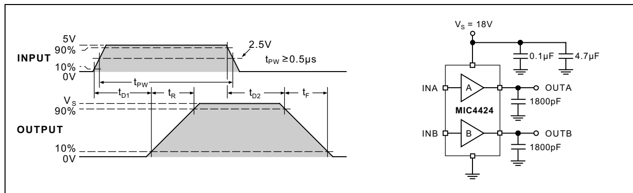
FIGURE 1-2: Non-Inverting Driver Switching Time.
