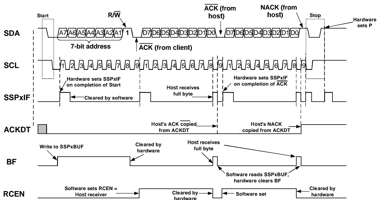
Figure 25-31. I 2 C Host Mode Waveform (Reception, 7-Bit Address)
