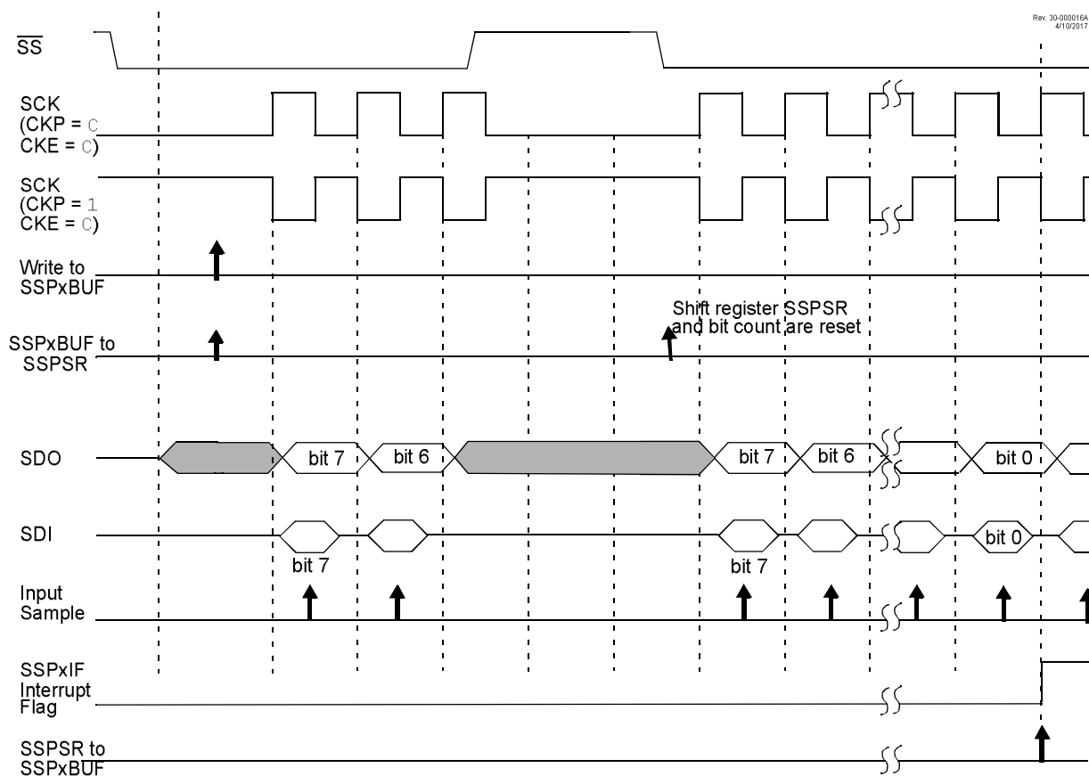
Figure 25-6. Client Select Synchronous Waveform
