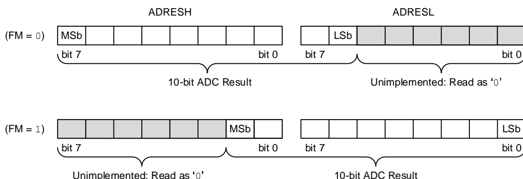
Figure 27-3. 10-Bit ADC Conversion Result Format
