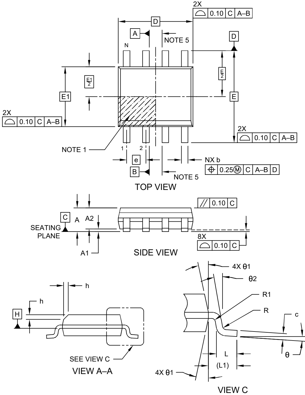
Microchip Technology Drawing No. C04-057-SN Rev H Sheet 1 of 2
