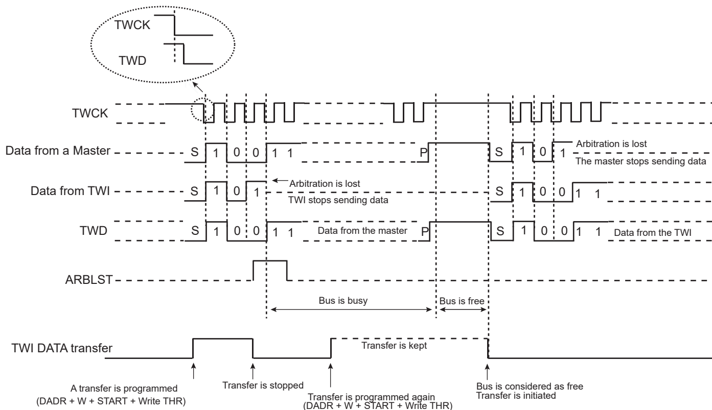
Figure 37-20: Arbitration Cases
