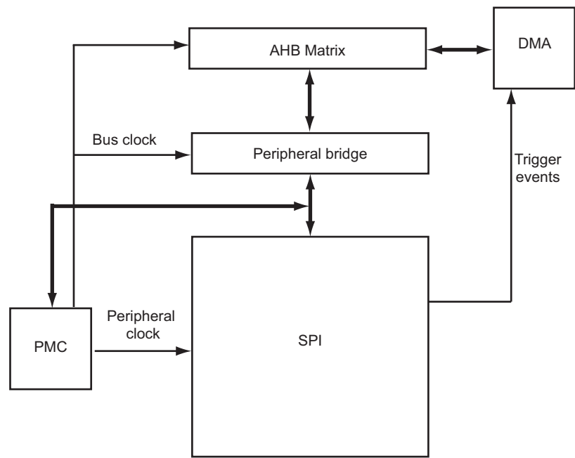
Figure 34-1: Block Diagram
