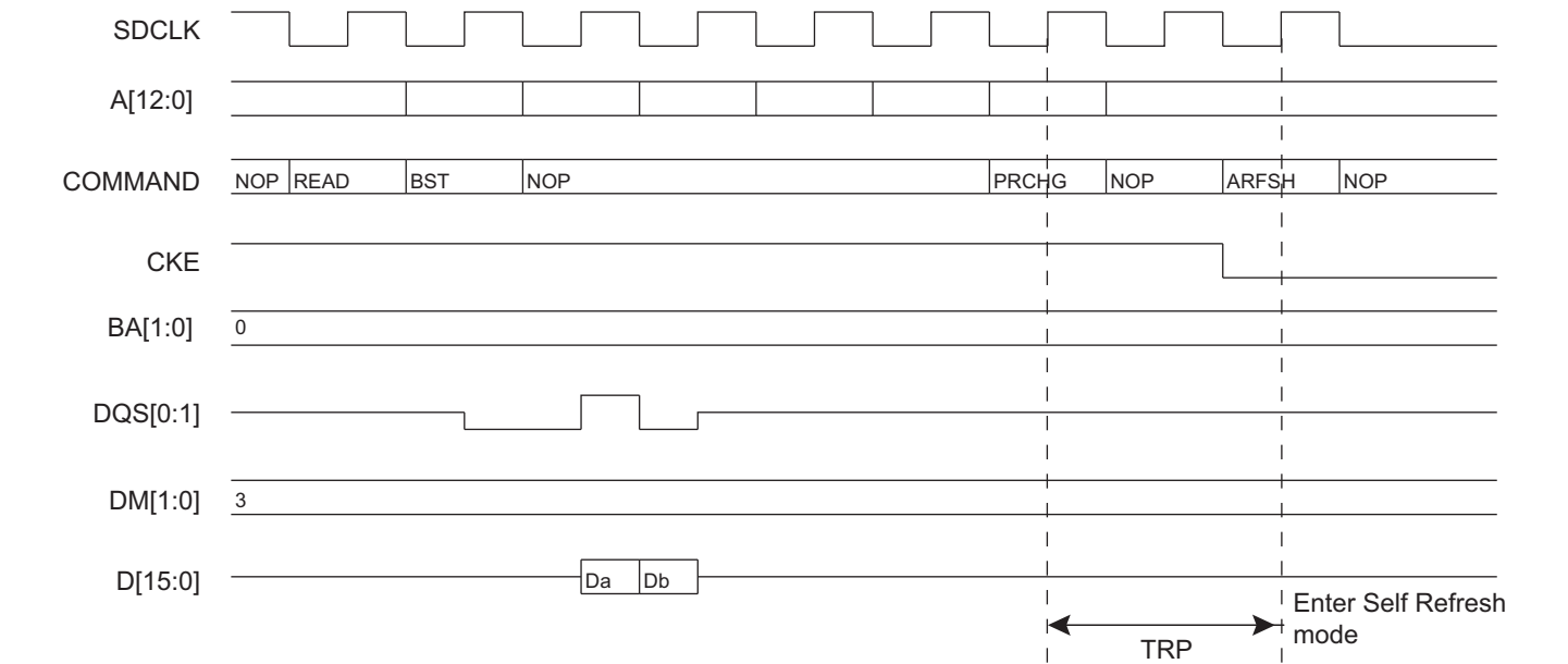
Figure 29-17: Self Refresh Mode Entry, DDRSDRC_LPR.TIMEOUT = 0
