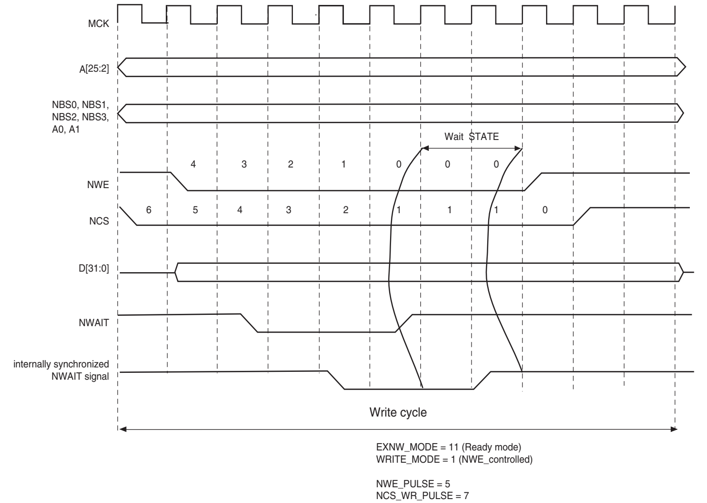
Figure 28-28: NWAIT Assertion in Write Access: Ready Mode (EXNW_MODE = 11)
