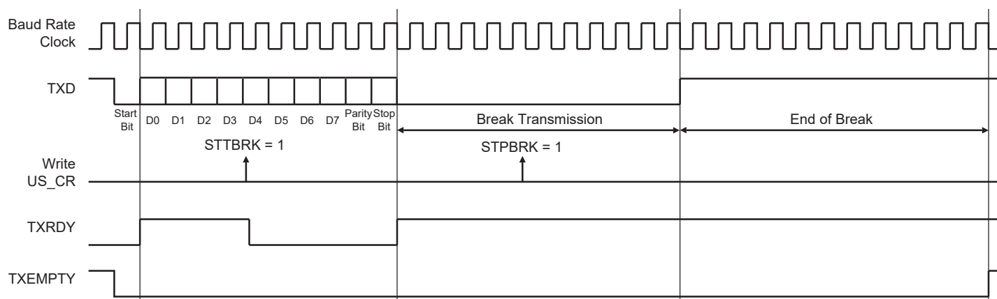
Figure 38-25: Break Transmission
