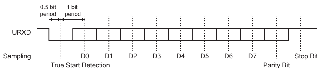
Figure 39-4: Character Reception
