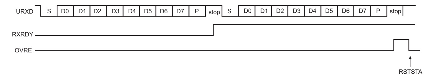
Figure 39-6: Receiver Overrun
