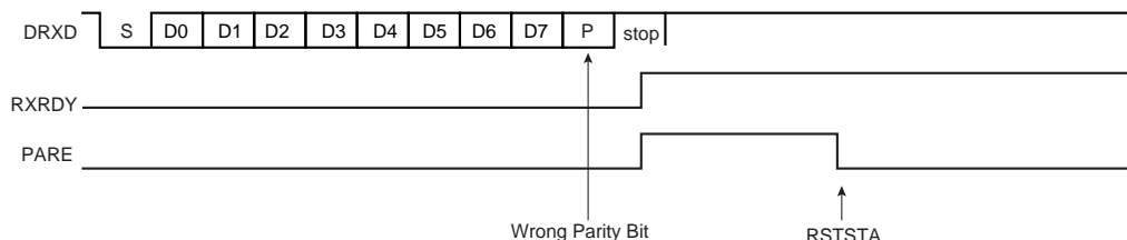
Figure 23-8: Parity Error
