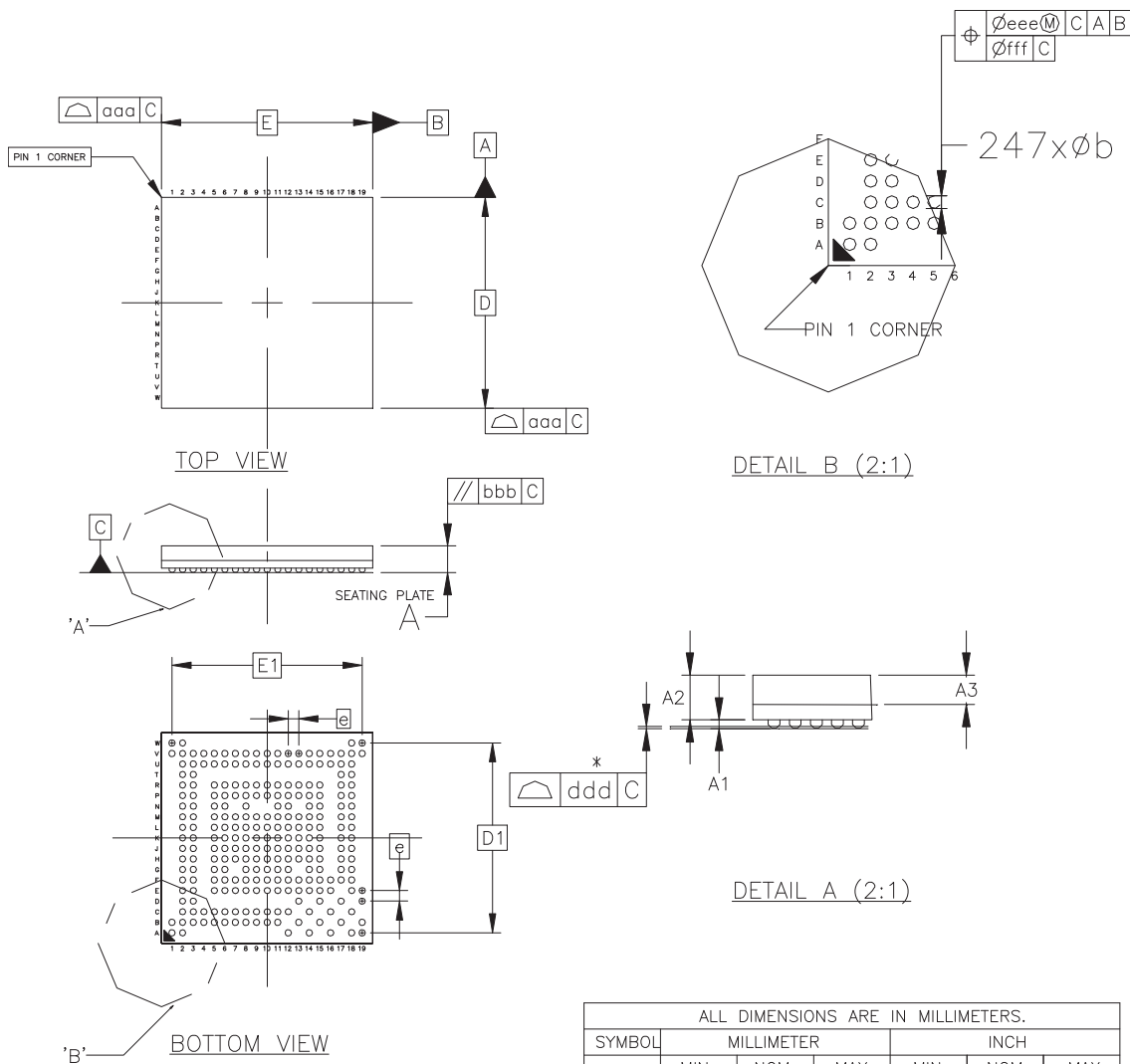
Figure 46-2: 247-ball TFBGA Package Drawing
