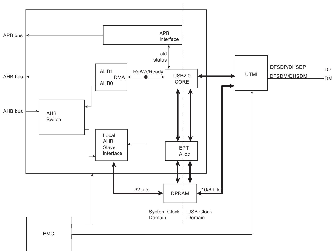
Figure 31-1: Block Diagram
