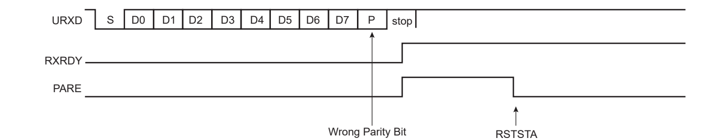
Figure 39-7: Parity Error
