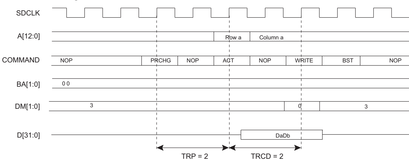
Figure 29-4: Single Write Access, Row Closed, SDR-SDRAM Device
