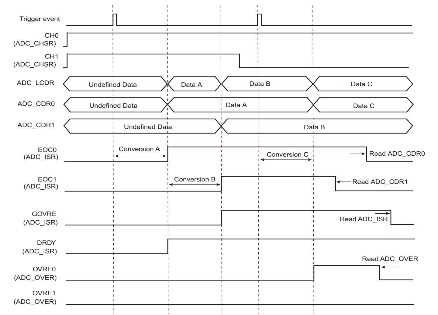
Figure 40-4: EOCx, OVREx and GOVREx Flag Behavior
