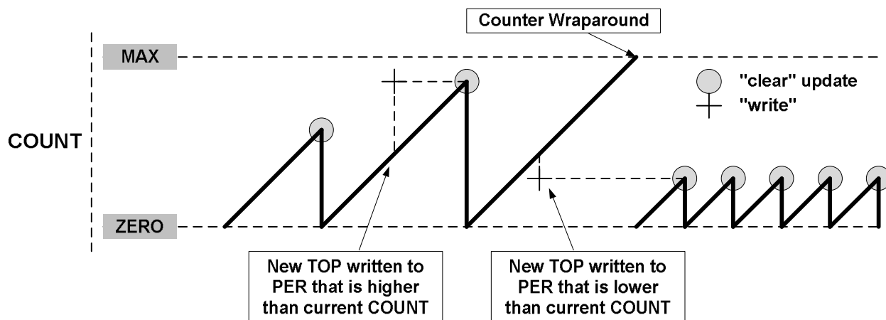
Figure 39-8. Unbuffered Single-Slope Up-Counting Operation
