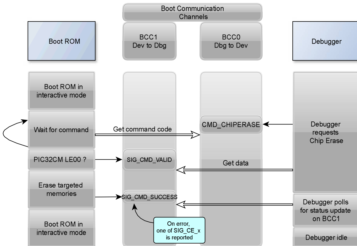
Figure 13-16. CMD_CHIPERASE and CM_CHIPERASE_ALL Flow diagram
