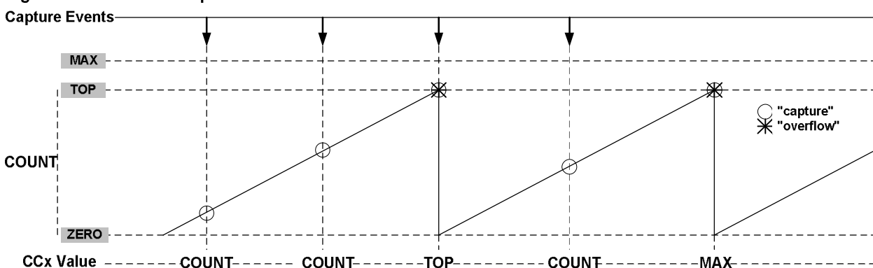
Figure 40-35. Time-Stamp
