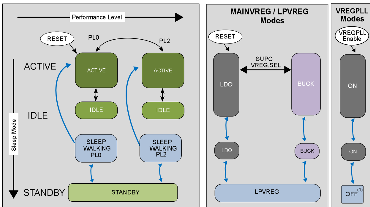
Figure 22-4. Operating Conditions and SleepWalking
