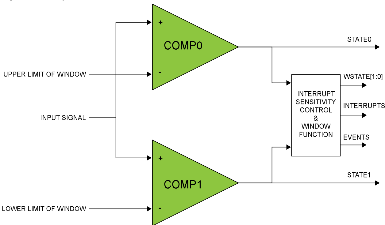
Figure 45-5. Comparators in Window Mode
