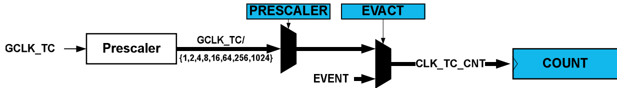
Figure 39-2. Prescaler
