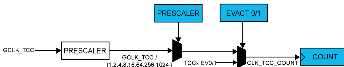
Figure 40-2. Prescaler
