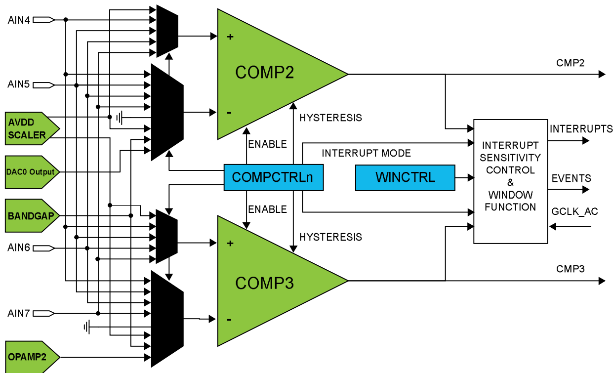
Figure 45-2. Analog Comparator Block Diagram (Second Pair)
