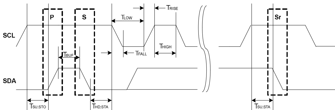
Figure 36-7. SCL Timing
