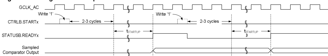
Figure 45-4. Single-Shot Example
