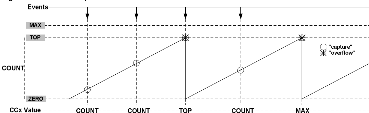
Figure 39-15. Time-Stamp
