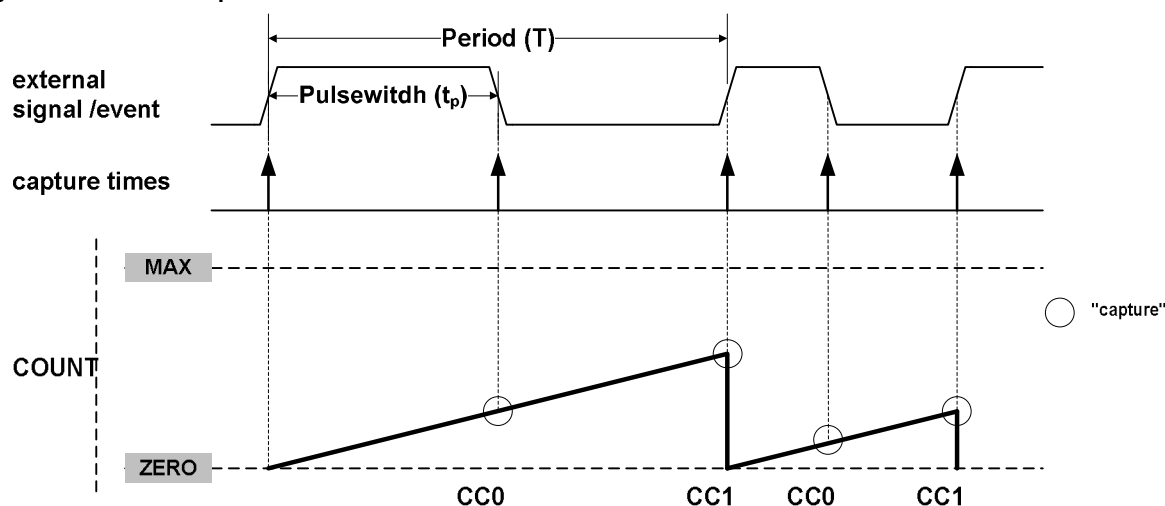
Figure 40-17. PWP Capture
