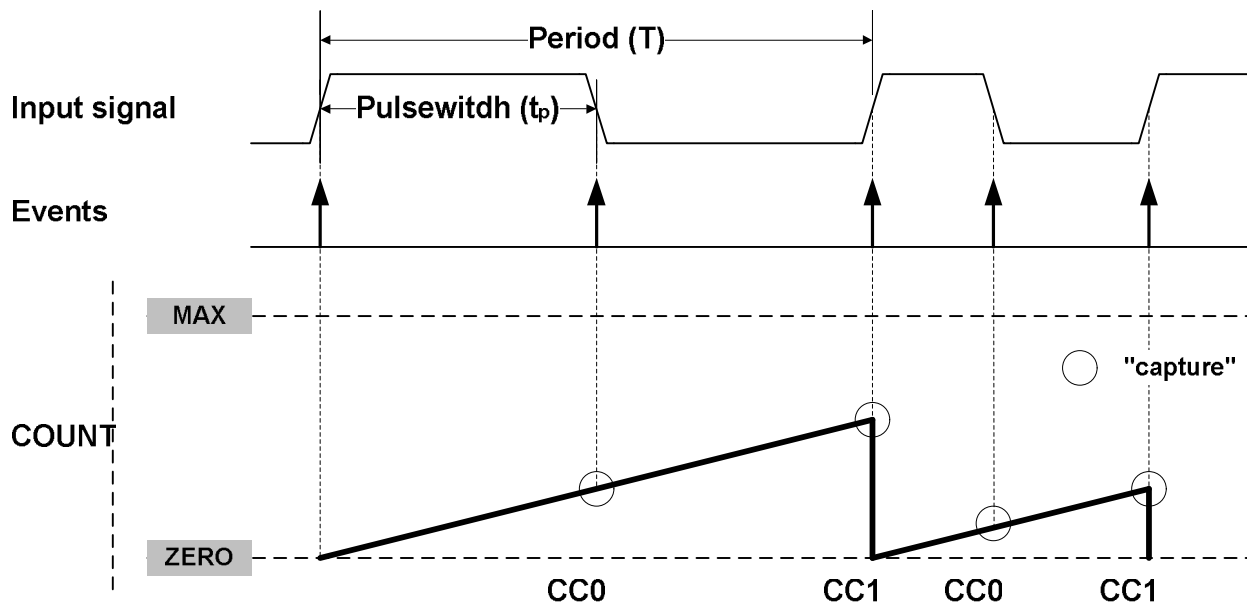
Figure 39-13. PWP Capture
