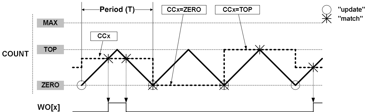
Figure 40-7. Dual-Slope Pulse Width Modulation
