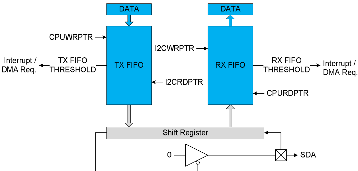
Figure 36-17. FIFO Overview
