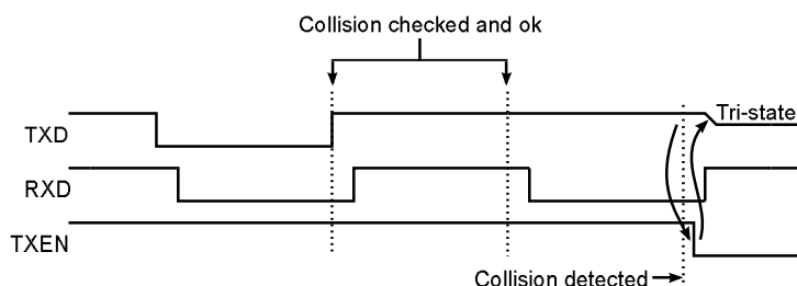
Figure 34-21. Collision Detected
