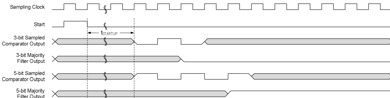
Figure 45-8. Single-Shot Filtering
