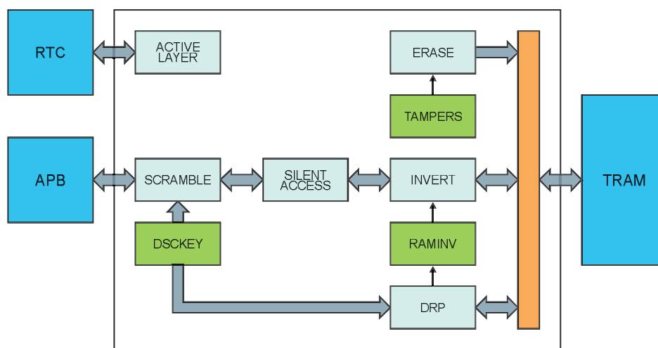
Figure 30-1. Block Diagram
