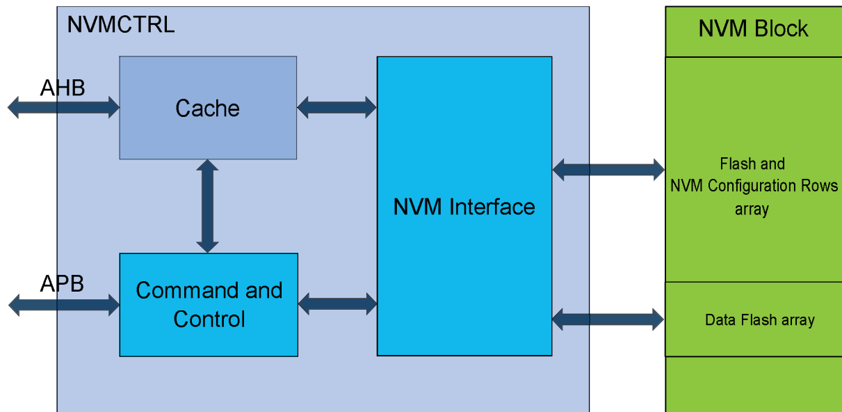
Figure 29-1. Block Diagram
