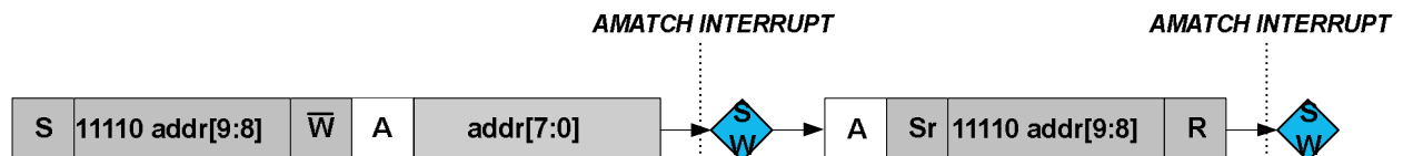
Figure 36-12. 10-bit Addressing
