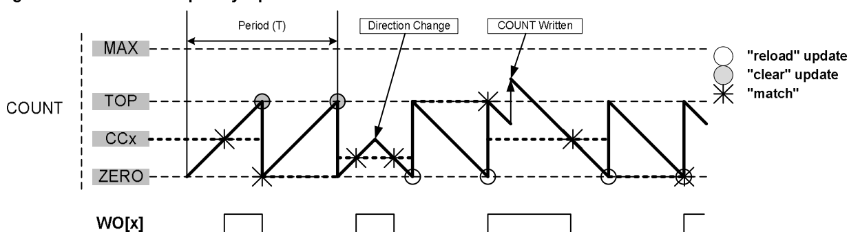
Figure 39-4. Normal Frequency Operation
