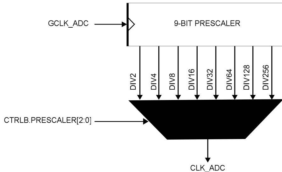
Figure 44-2. ADC Prescaler
