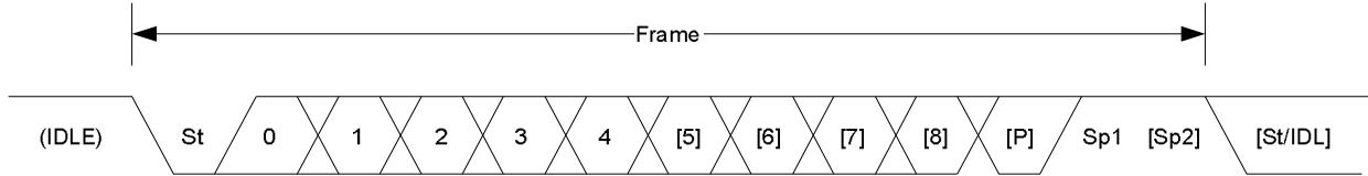
Figure 34-2. Frame Formats
