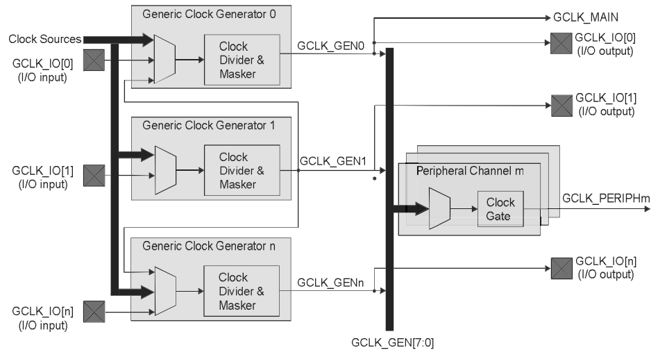
Figure 17-2. Generic Clock Controller Block Diagram
