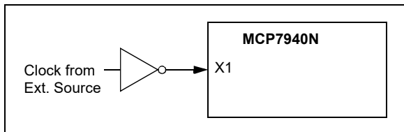
FIGURE 5-4: EXTERNAL CLOCK INPUT OPERATION
