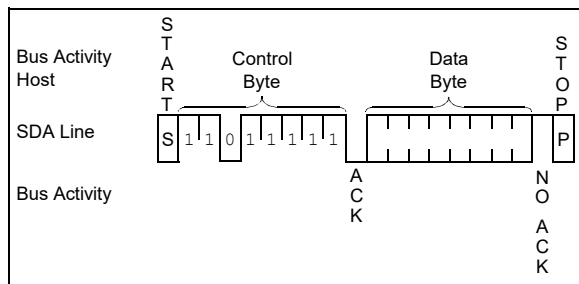
FIGURE 6-3: SRAM/RTCC CURRENT ADDRESS READ
