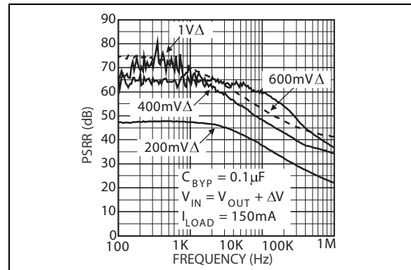
FIGURE 2-29: Power Supply Rejection Ratio, 3V_{OUT} .
