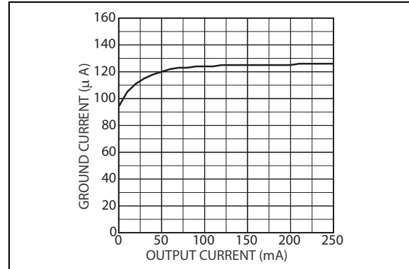
FIGURE 2-16: Ground Current vs. Load Current for LDO 3.
