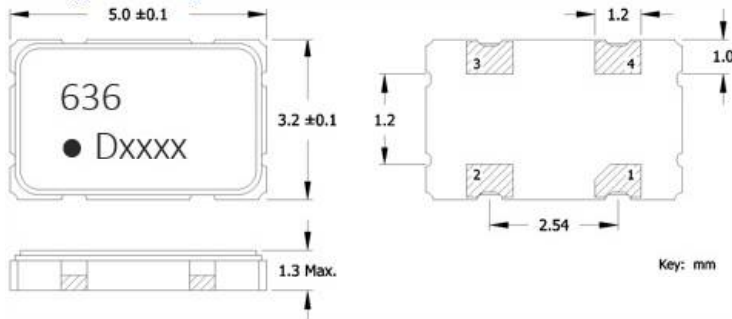
Package Drawing
