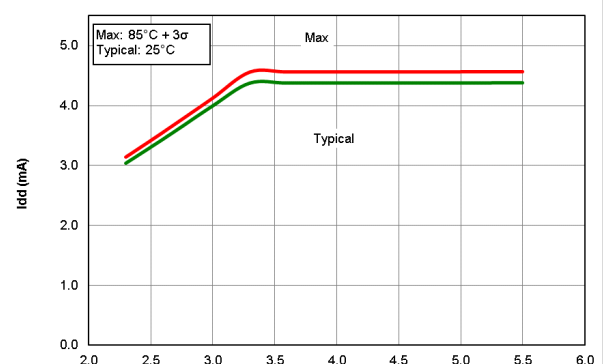
Figure 40-16. I_{DD} HS Oscillator 32 MHz, PIC16F18426/46 only
