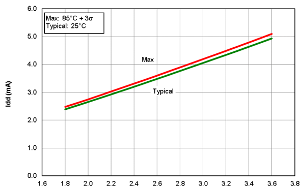
Figure 40-17. I_{DD} HFINTOSC Mode, F OSC = 32 MHz, PIC16LF18426/46 only
