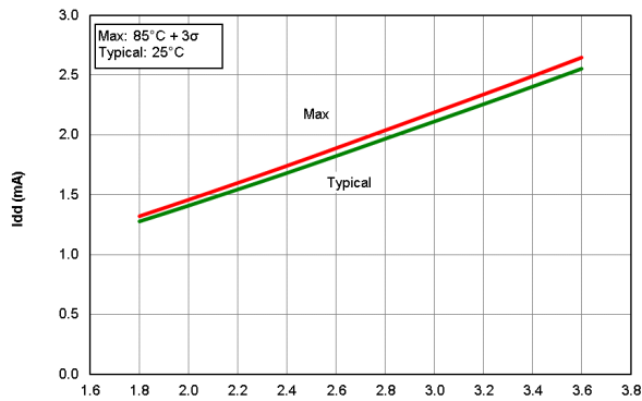
Figure 40-19. I_{DD} HFINTOSC Mode, F_{OSC}=16 MHz, PIC16LF18426/46 only
