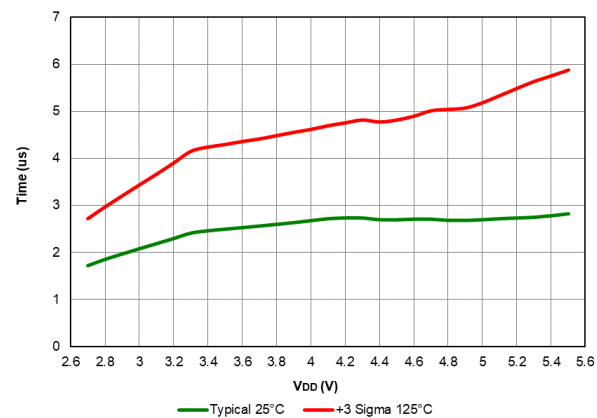
Figure 40-47. BOR Response Time, PIC16F18426/46 only
