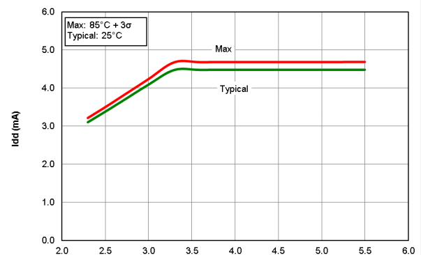
Figure 40-18. I_{DD} HFINTOSC Mode, F OSC = 32 MHz, PIC16F18426/46 only
