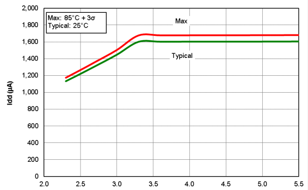
Figure 40-22. I_{DD} HFINTOSC Idle Mode, F_{OSC}=16 MHz, PIC16F18426/46 only
