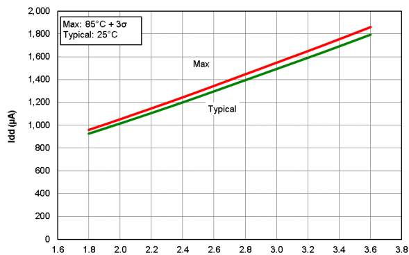
Figure 40-23. I_{DD} HFINTOSC Doze Mode, F_{OSC}=16 MHz, PIC16LF18426/46 only
