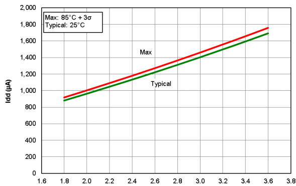
Figure 40-21. I_{DD} HFINTOSC Idle Mode, F_{OSC}=16 MHz, PIC16LF18426/46 only
