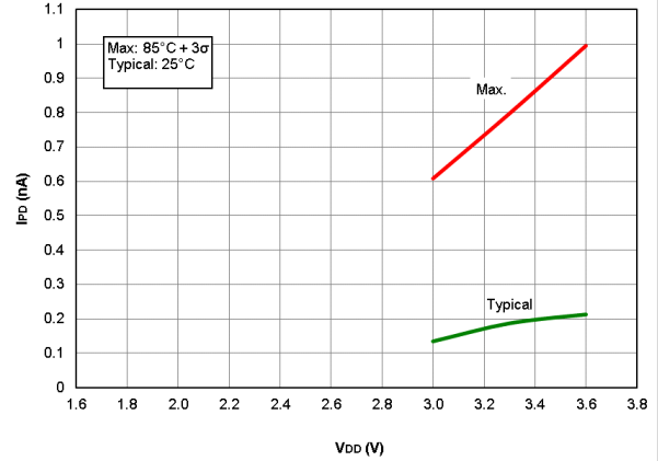
Figure 40-10. I_{PD} Comparator, PIC16F18426/46 only
