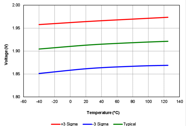
Figure 40-42. Brown-Out Reset Voltage, Trip Point BORV = 01, PIC16F18426/46 only
