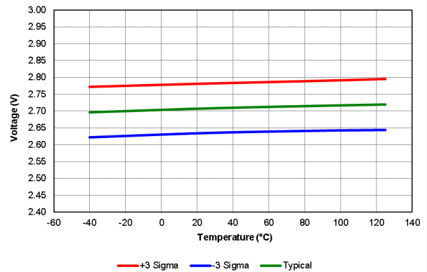
Figure 40-40. Brown-Out Reset Voltage, Trip Point BORV = 01, PIC16LF18426/46 only
