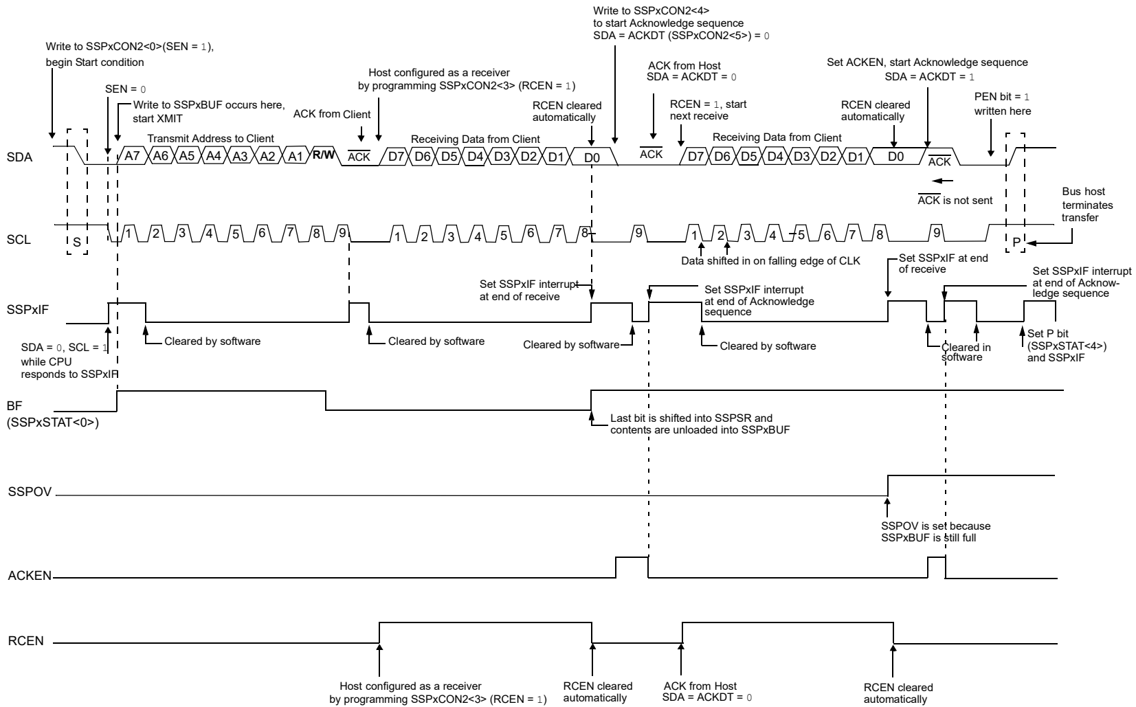
Figure 29-29. I 2 C Host Mode Waveform (Reception, 7-Bit Address)
