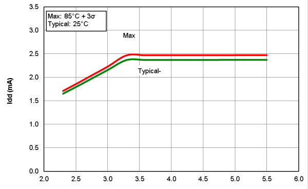
Figure 40-20. I_{DD} HFINTOSC Mode, F_{OSC}=16 MHz, PIC16F18426/46 only
