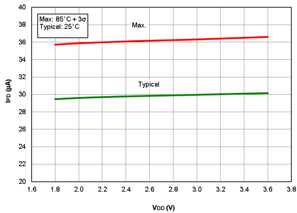
Figure 40-11. I_{PD} Base, 01, PIC16F18426/46 only
