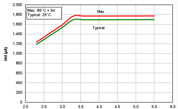
Figure 40-24. I_{DD} HFINTOSC Doze Mode, F_{OSC}=16 MHz, PIC16F18426/46 only
