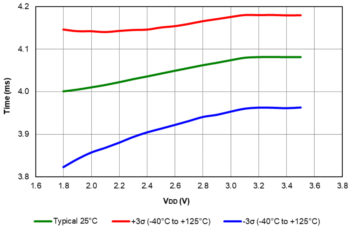
Figure 40-115. WDT Time-Out Period, PIC16LF18426/46 only
