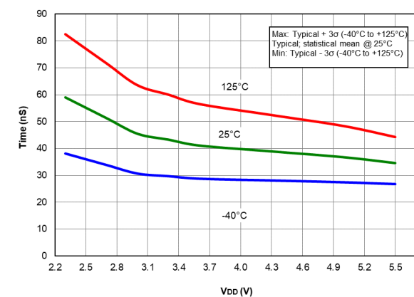
Figure 40-84. Comparator Response Time Overvoltage, Normal Power Mode (CxSP = 1), Typical Measured Values, PIC16F18426/46 only
