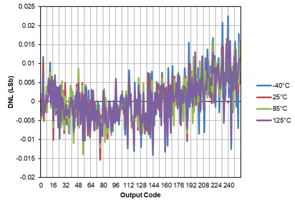
Figure 40-68. Typical DAC DNL Error, V DD = 3.0V, V REF = External 3V, All devices
