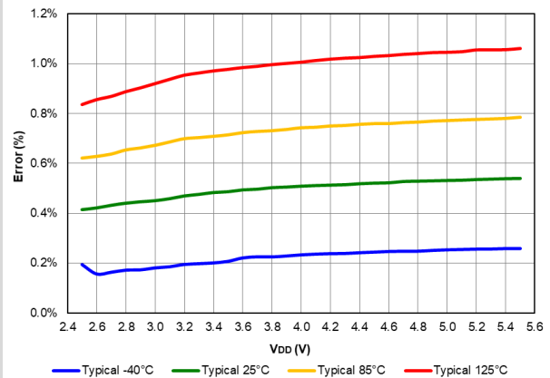
Figure 40-94. FVR Voltage Error 2x, PIC16F18426/46 only
