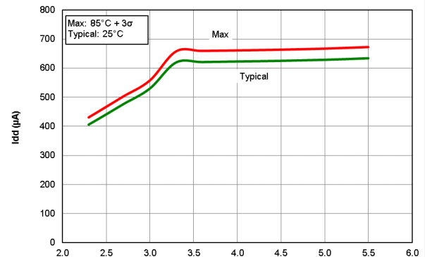
Figure 40-14. I_{DD} XT Oscillator 4 MHz, PIC16F18426/46 only
