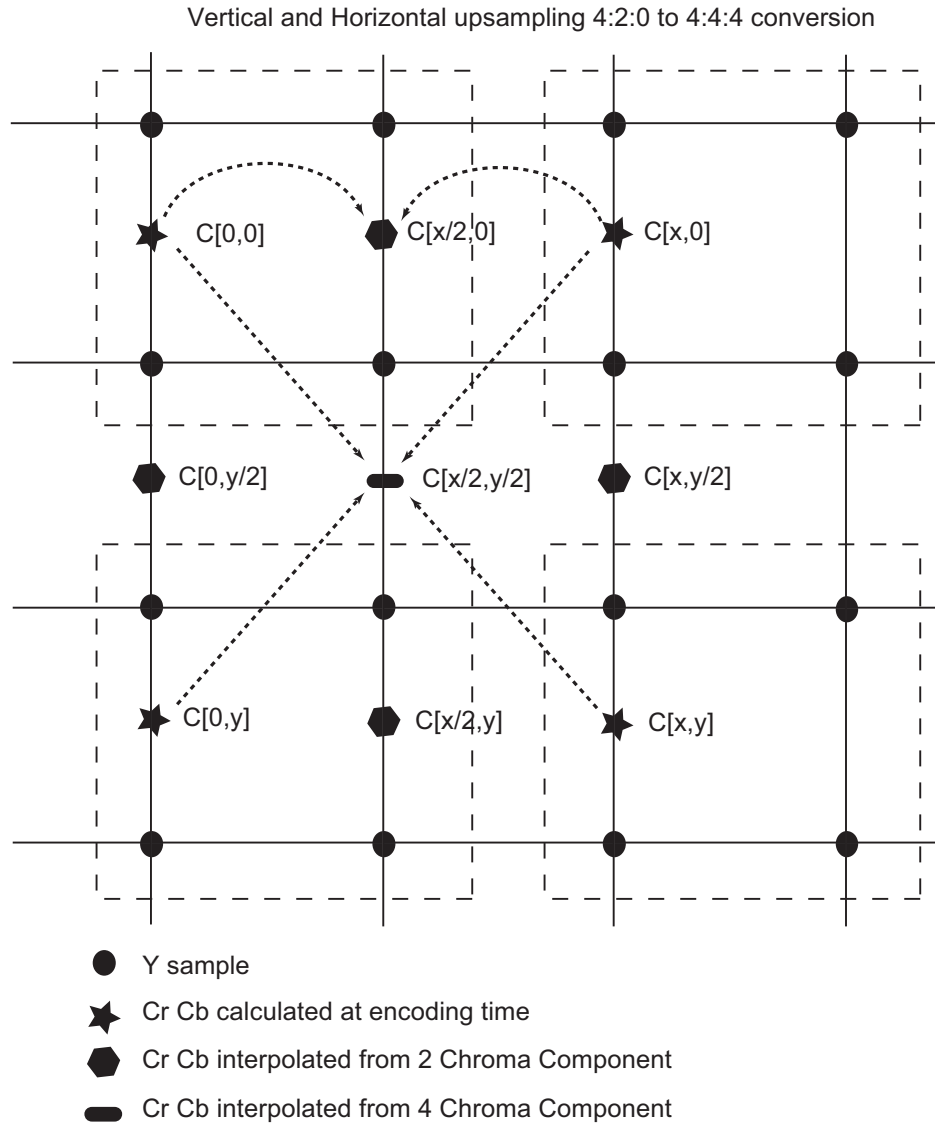
Figure 44-5: 4:2:0 Upsampling Algorithm
