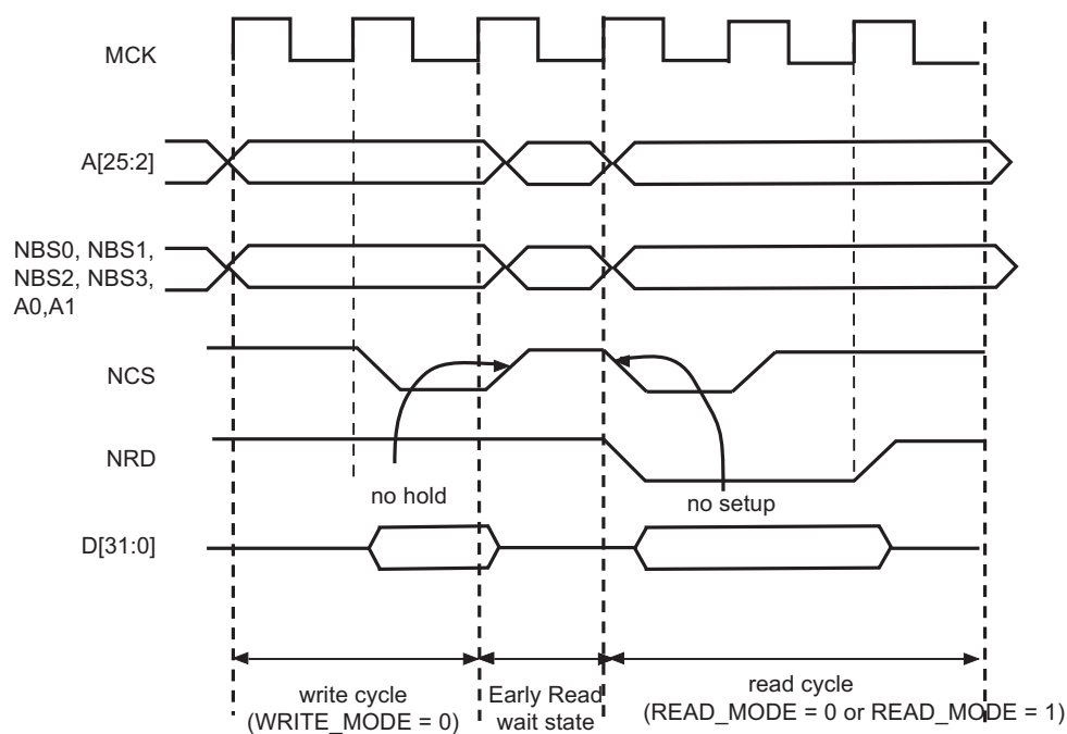
Figure 28-18: Early Read Wait State: NCS Controlled Write with No Hold Followed by a Read with No NCS Setup
