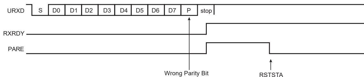
Figure 39-7: Parity Error
