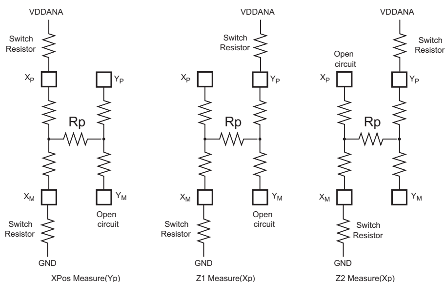
Figure 40-8: Pressure Measurement
