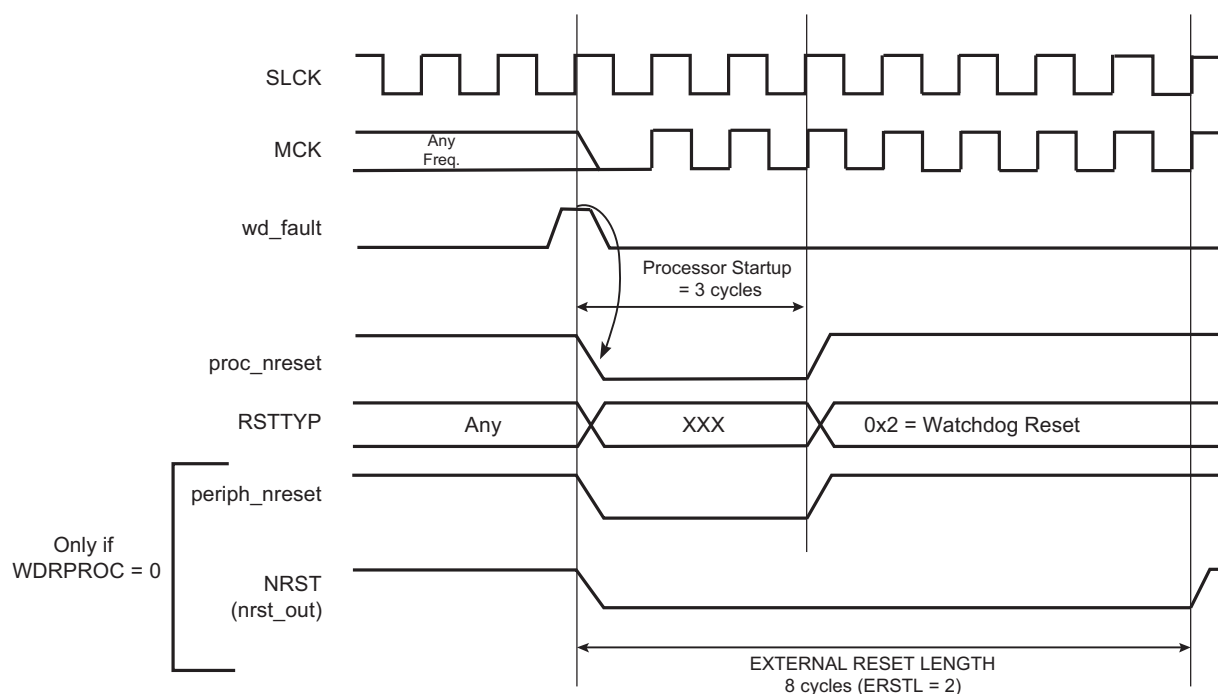
Figure 13-8: Watchdog Reset
