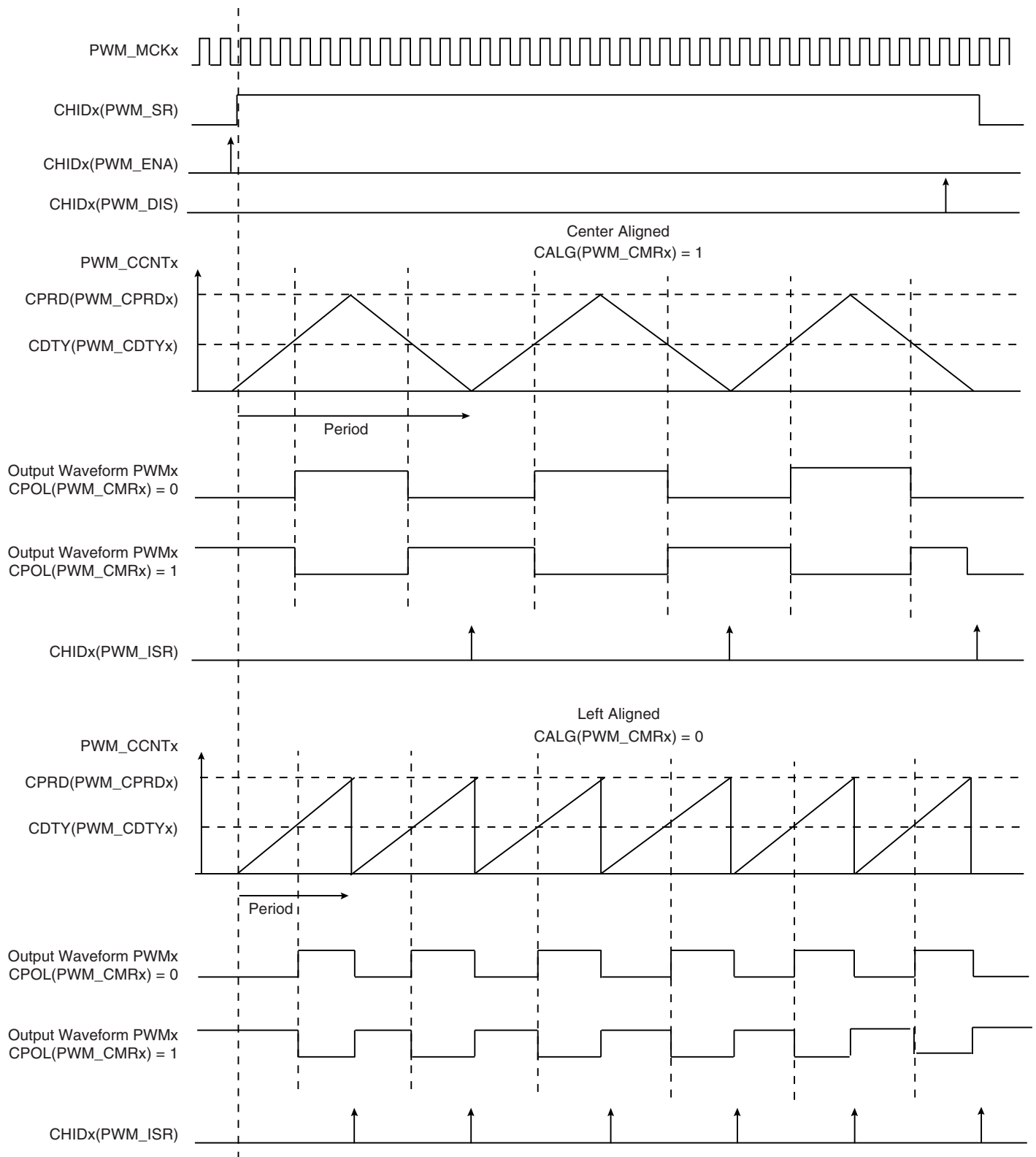
Figure 36-5: Waveform Properties
