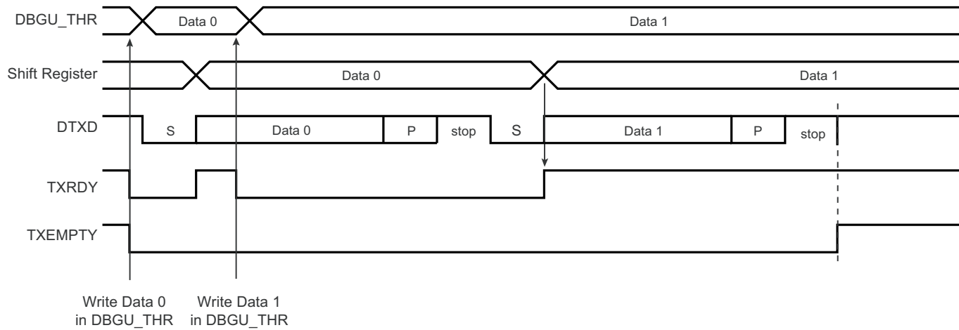
Figure 23-11: Transmitter Control
