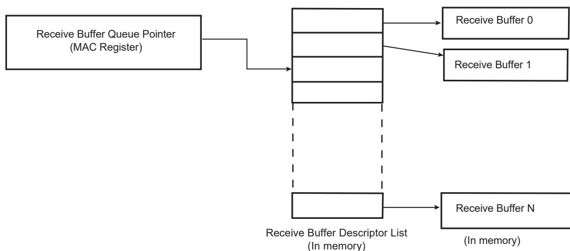
Figure 43-2: Receive Buffer List
