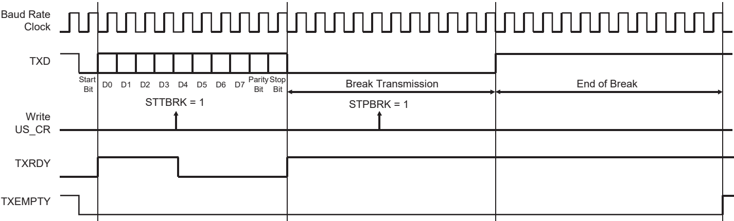
Figure 38-25: Break Transmission
