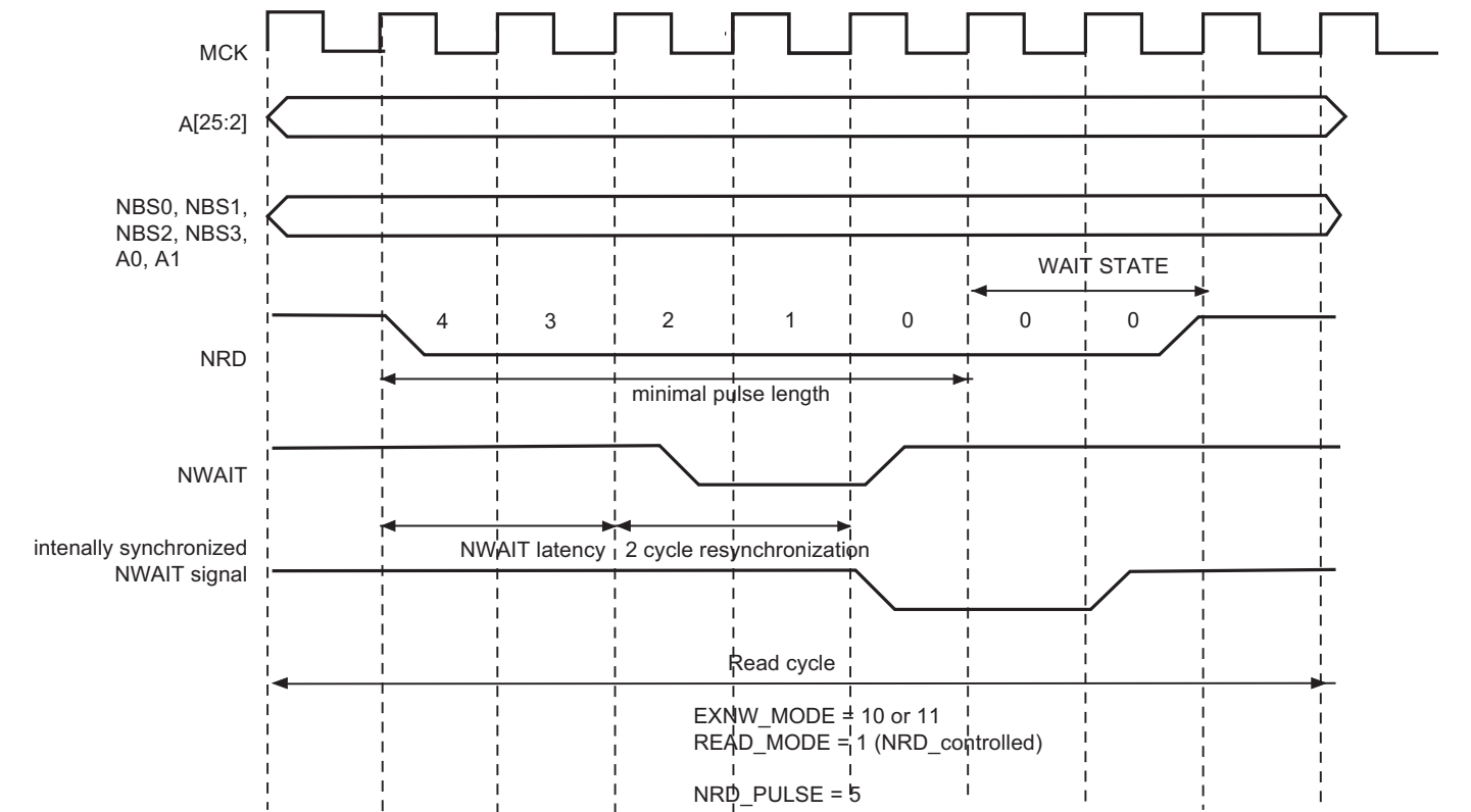
Figure 28-30: NWAIT Latency
