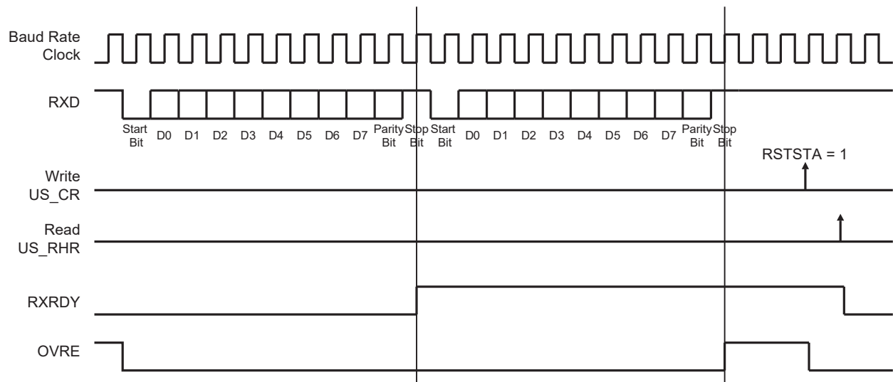
Figure 38-20: Receiver Status
