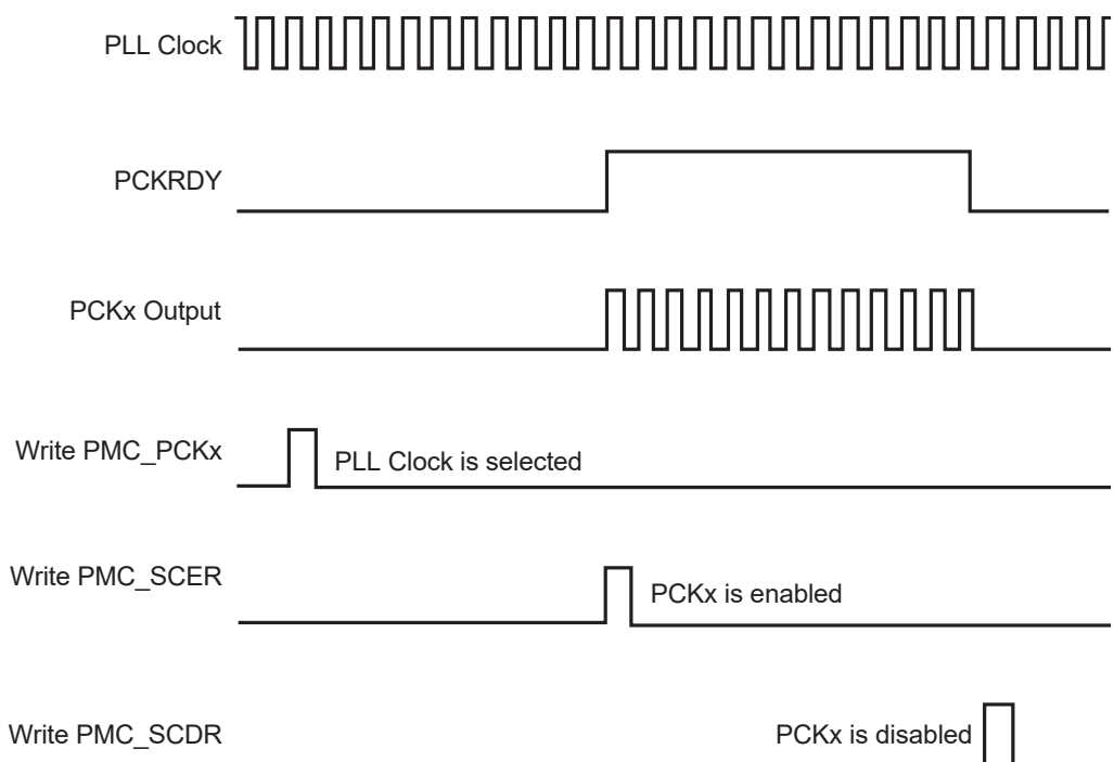
Figure 21-9: Programmable Clock Output Programming
