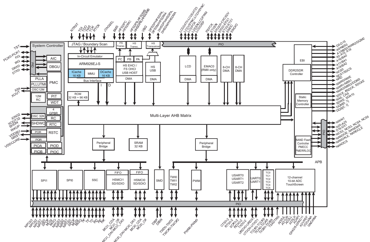
Figure 1-1: SAM9G35 Block Diagram
