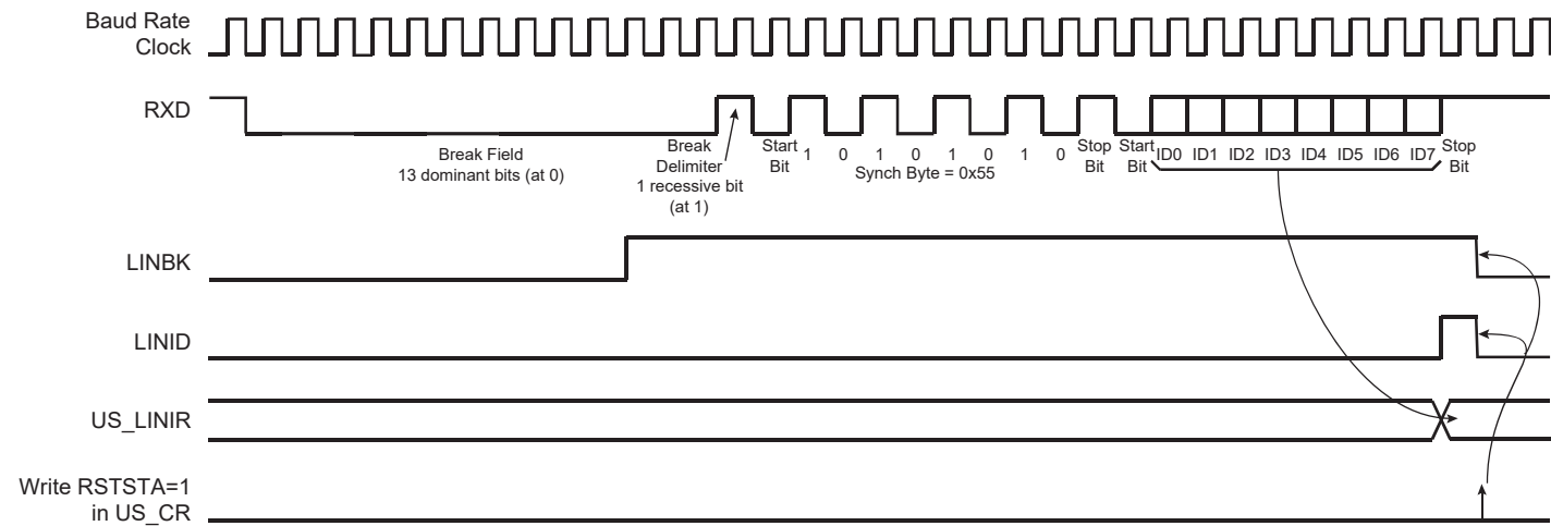
Figure 38-40: Header Reception
