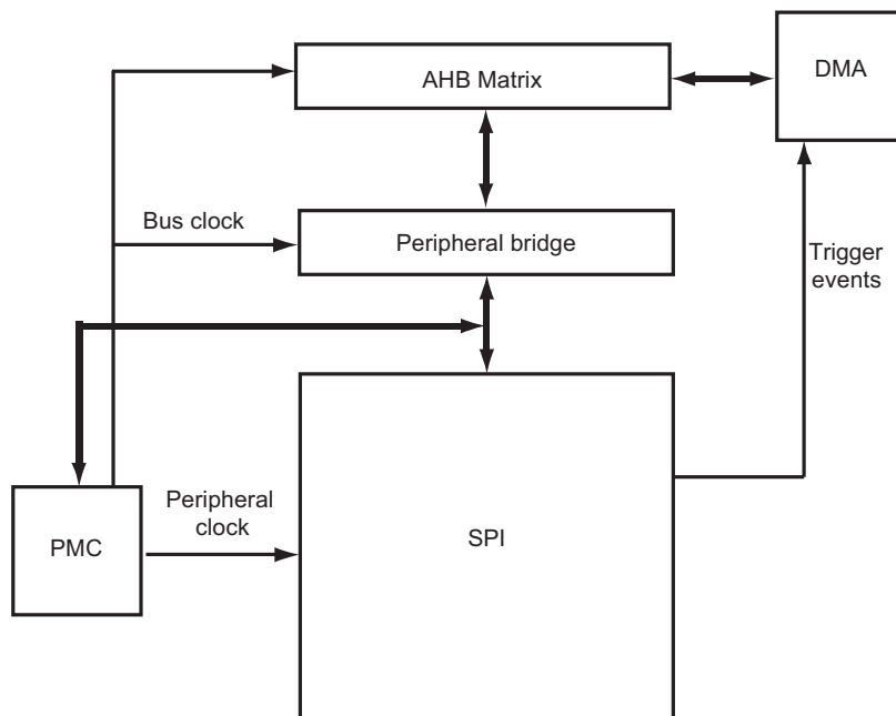
Figure 34-1: Block Diagram
