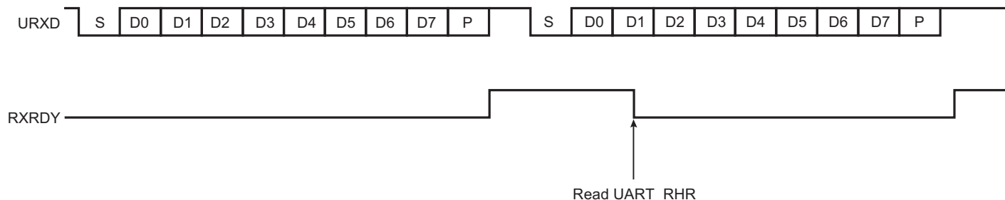
Figure 39-5: Receiver Ready
